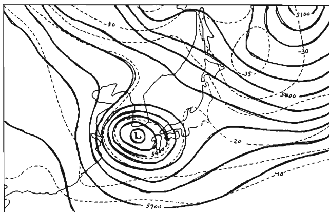
Fig. 5. 500 mb chart at 21 LST 16 March 1965. (black lines: isohyps, dotted lines: isotherms)
