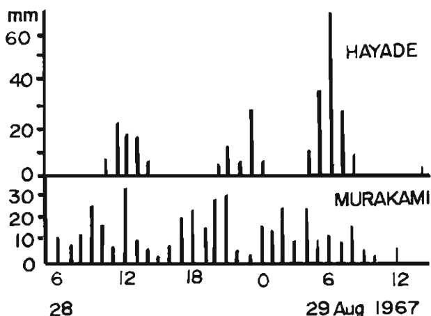
Fig. 21. Sequence of the hourly amount of the rainfall at Hayade and Murakami in Niigata Prefecture from 06 LST 28 to 12 LST 29 August 1967.
