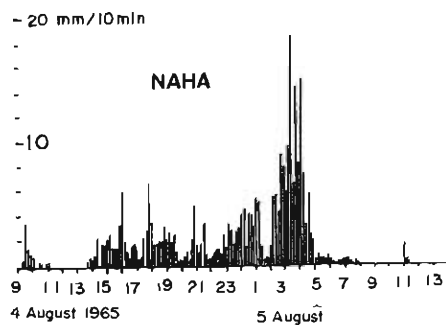
Fig. 13 b. Same as Fig. 12 but for 4-5 August 1972 at NAHA.
