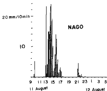
Fig. 13 a. Same as Fig. 12 but for 11-12 August 1972 at NAGO in OKI-NAWA.
