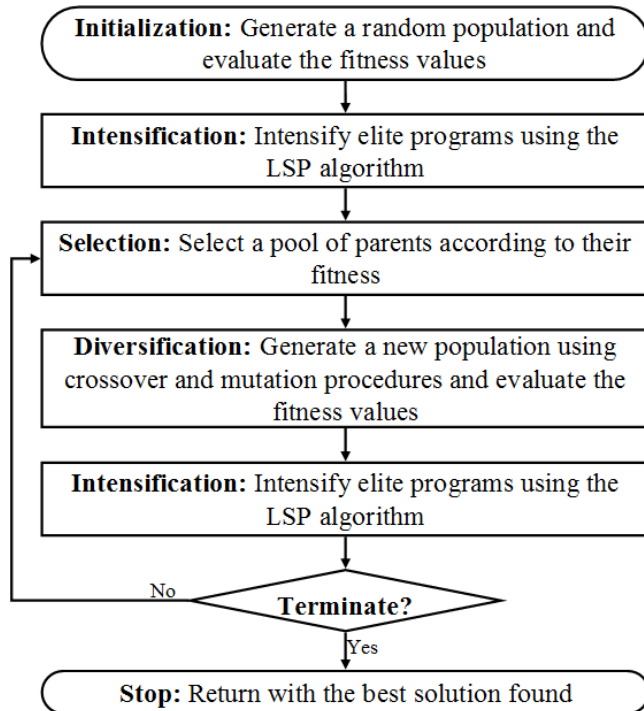
Fig.5 The flowchart of the MP algorithm
