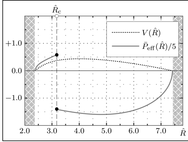
FIG. 2: Plot of the effective potential and of the effective Euclidean momentum along a tunnelling trajectory. The quantities are calculated for a Minkowski Schwarzschild junction in which M = 1 , \tilde{\sigma} = 0.25 , which results in the relevant sign for the outside spacetime to change at \hat{R}_c \approx 3.175 . The plot clearly emphasizes the discontinuity in the expression for the effective momentum (16) due to the change in the \epsilon_+ sign.
