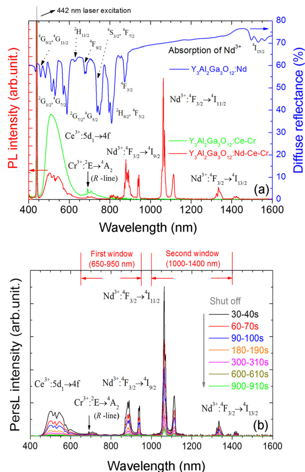
FIG. 1. (a) PL spectra of the YAGG:Ce-Cr and YAGG:Nd-Ce-Cr ceramics as well as the diffuse reflectance of the YAGG:Nd ceramic and (b) PersL spectra of the YAGG:Ce-Cr and YAGG:Nd-Ce-Cr ceramics (integrating time: 10 s).
