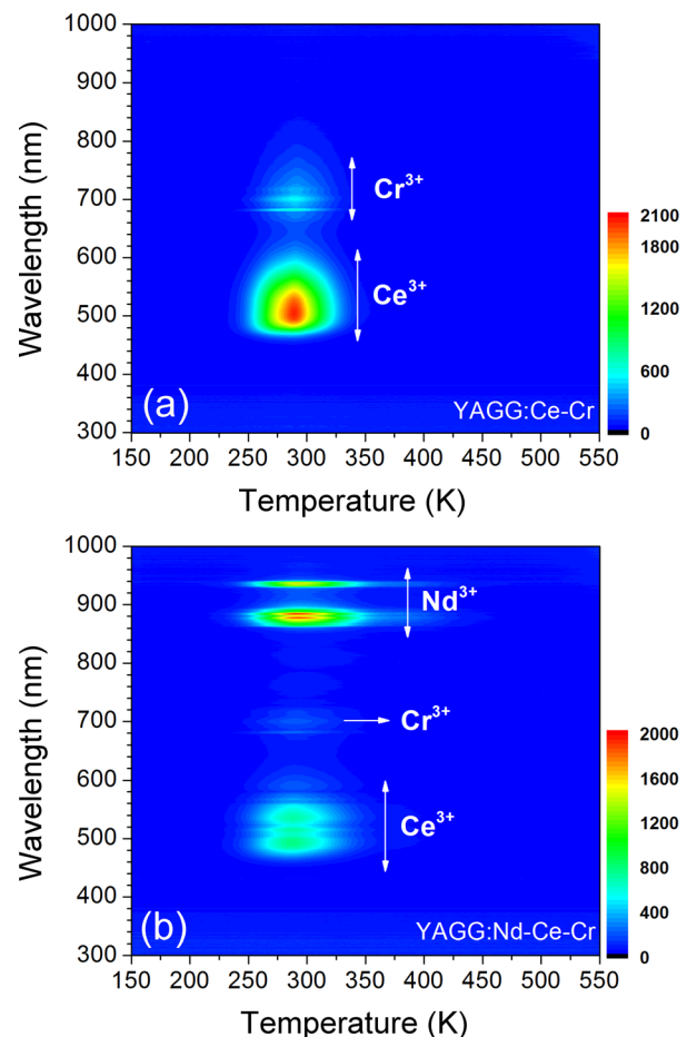
FIG. 3. Wavelength-temperature ( \lambda -T) contour plots of the (a) YAGG:Ce-Cr and (b) YAGG:Nd-Ce-Cr ceramics.
