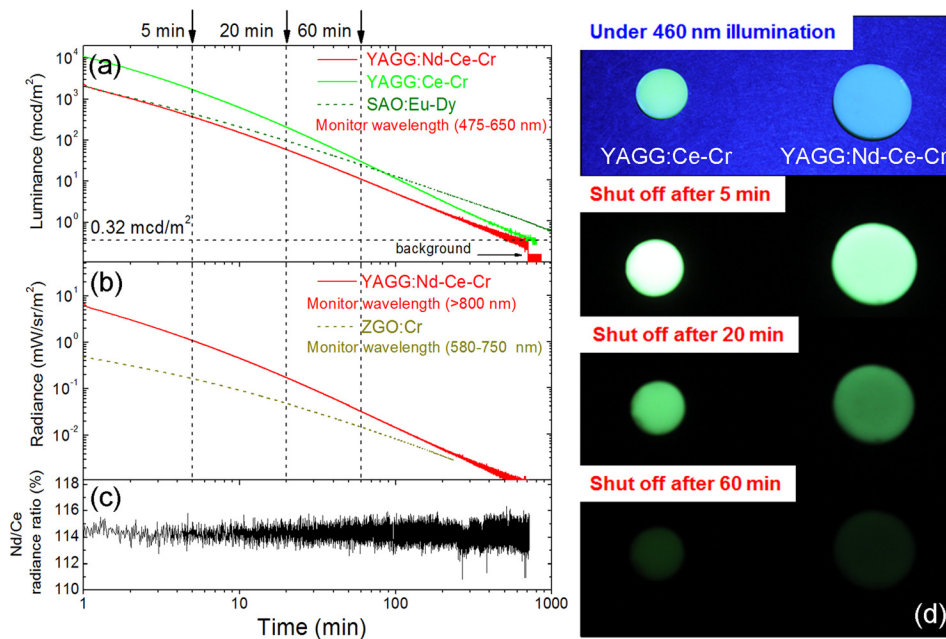
FIG. 2. Persistent decay curves of the YAGG:Nd-Ce-Cr ceramic: (a) luminance monitoring Ce 3+ (YAGG:Ce-Cr and SrAl 2 O 4 :Eu 2+ -Dy 3+ ceramics as references), (b) radiance monitoring Nd 3+ (ZnGa 2 O 4 :Cr 3+ ceramic as a reference), (c) Nd 3+ /Ce 3+ radiance ratio (%) against the monitoring time of the decay curve, and (d) photographs of the YAGG:Ce-Cr and YAGG:Nd-Ce-Cr ceramics under and after blue LED lamp (460 nm, 3 W output) illumination.
