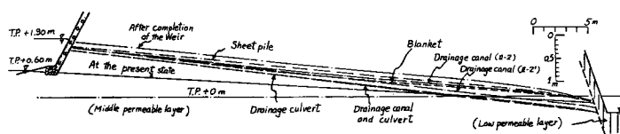
Fig. 12 Free surface.
