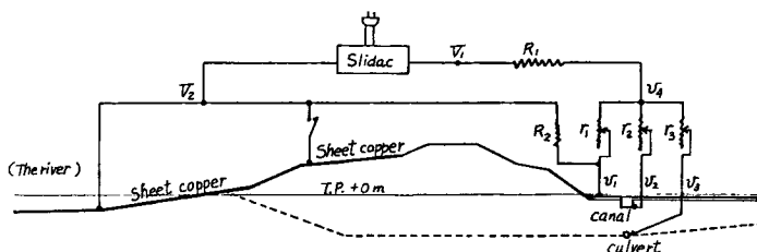
Fig. 8 Electric circuit of an experimental model.
