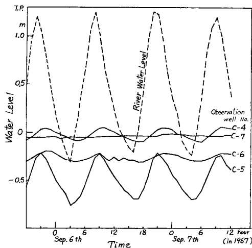
Fig. 4 Variation in the groundwater head.
