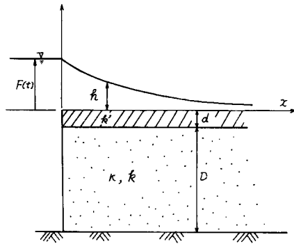
Fig. 3 Ground model.
