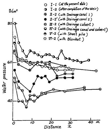
Fig. 10 Water pressure distribution.
