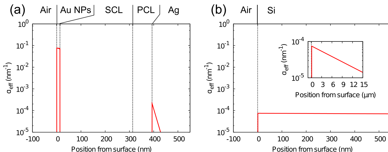
FIG. 3. Effective absorption coefficient, \alpha_{\text{eff}} (nm -1 ), as a function of position from surface for (a) local plasmon resonator with 80-nm-thick PCL ( A = 0.99 ) and (b) Si wafer ( A = 0.67 ) at the wavelength of 785 nm. Inset in (b) shows a gradual decrease in \alpha_{\text{eff}} over several micrometers in the Si wafer.
