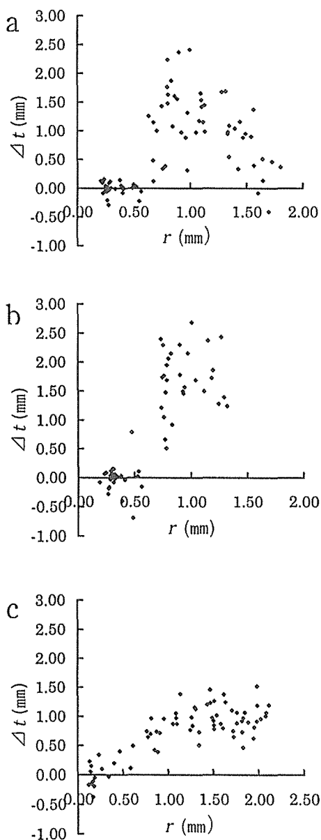
Fig. 6 The displacements ( \Delta r ) in tangential direction. X-axis is radial position at one end. If \Delta t is plus, the inclination is S-helix to the general direction of the vessels formed at the beginning of the season. a: Earlywood in Castanea crenata . b: Earlywood in C. crenata , which has narrow annual ring. c: Juglans sieboldiana .
