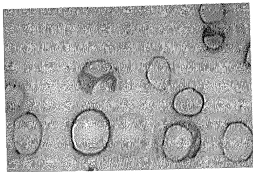
Fig. 8 A set of video-microscopic photographs on a transverse section of a saw-cut end of Paulownia tomentosa block. Vessels on the current annual ring can be identified by various colored pigments injected before the saw-cutting. b: Magnified view of box a. Bar: 1 mm.
