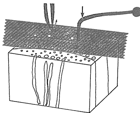
Fig. 1 A schematic illustration for the pigment injection. The surface of a specimen block was covered by a cellophane tape and then opened on the vessels, being made holes by a point of a pin or cut off by a razor blade. A small droplet of pigments was put on the opened pores.
