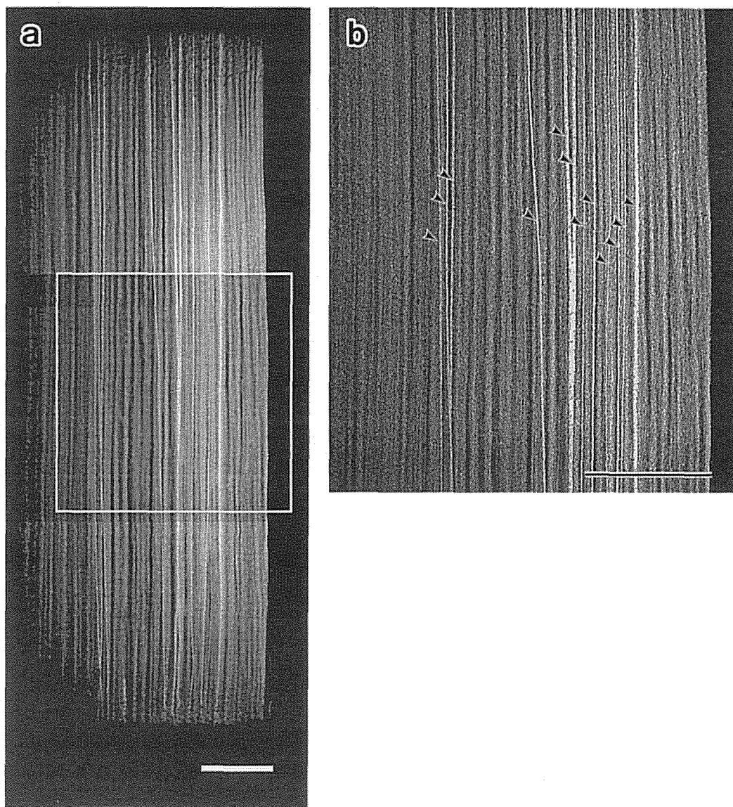
Fig. 2 Sofx X-ray figures for the block of Castanea crenata which has 5 mm thick. a: Whole figure of specimen. b: Magnified figure of box of a. Arrowheads point out the location of inserted wire. There are 3 kinds of wire (0.2 mm, 0.1 mm and 0.05 mm in diameter). The number of inserted wire is 12. Bars: 5 mm.
