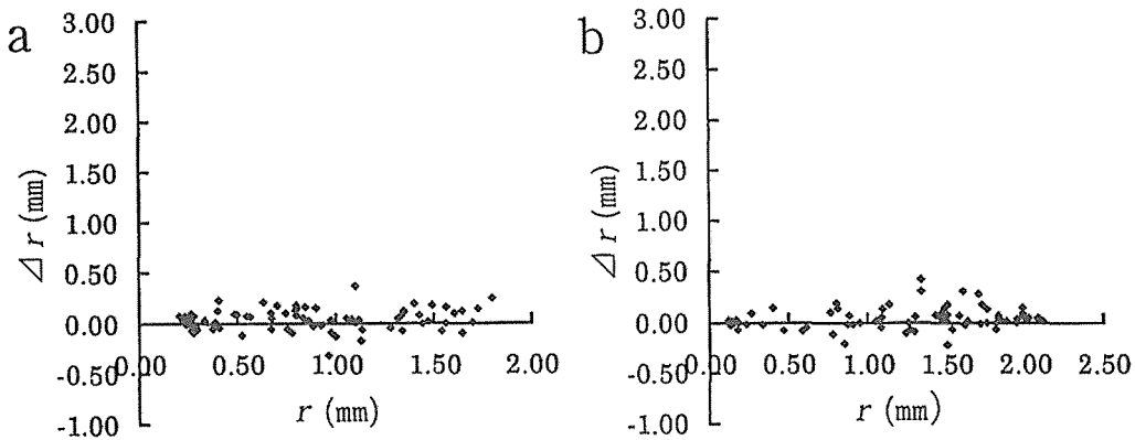
Fig. 5 The displacements ( \Delta r ) in radial direction. X-axis is radial position at one end. a: Earlywood in Castanea crenata . b: Juglans sieboldiana .
