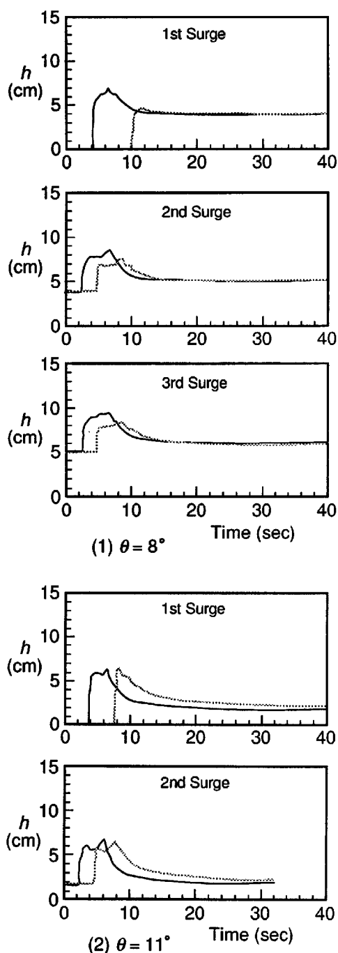
Fig. 8 Temporal depth variations measured at upstream and downstream stations along the flume. (1) Channel slope is 8^\circ , (2) Channel slope is 11^\circ
