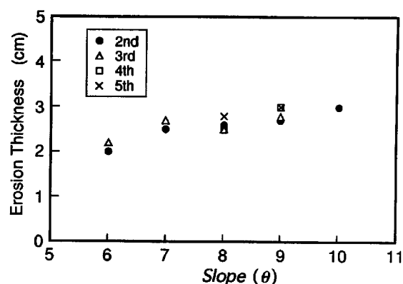
Fig. 11 Thickness of erosion of the newly deposited layer by the passage of the debris flow surge
