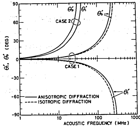
Fig.3.2-2 Calculated angles of incidence and diffraction outside the Te crystal at 10.6 \mu\text{m} as a function of frequency of a shear acoustic wave propagating in the y direction with displacement parallel to the x axis. The incident light is an ordinary wave polarized along the x axis and the diffraction plane lies in the y-z plane. The solid curves are obtained for anisotropic Bragg diffraction, while the broken curves are for isotropic Bragg diffraction. There are two kinds of solutions denoted respectively by "case 1" and "case 2" for the anisotropic diffraction.
