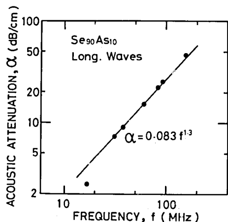
Fig.5.2-10 Acoustic loss as a function of acoustic frequency at room temperature. (a) and (b) are respectively for longitudinal and shear waves in Se 95 As 5 , and (c) and (d) are respectively for longitudinal and shear waves in Se 90 As 10 .
