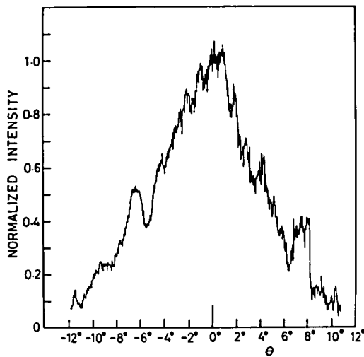
Fig.6.2-4 Angular distribution of the far-field intensity pattern. The thickness and the length of the Se film are 44\text{ }\mu\text{m} and 5.4\text{ mm} , respectively.
