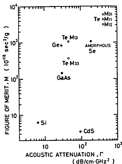
Fig.2.6-2 Relation between figure of merit and acoustic attenuation for various acousto-optic materials measured at 10.6\text{ }\mu\text{m} . The open circles denote the values for Te.
