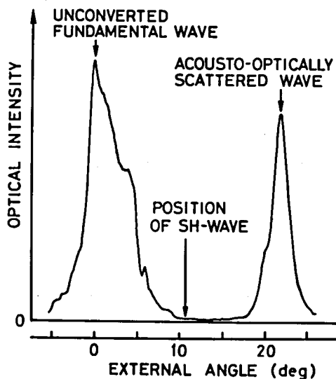
Fig.4.3-3 Intensity distributions of the emergent optical signals. The angles were measured outside the crystal.
