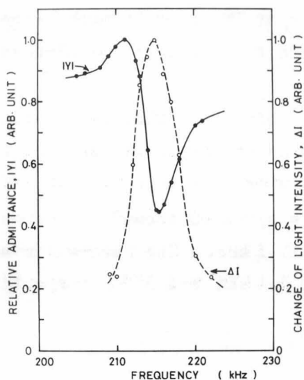
Fig.6.2-8 The electrical admittance of the modulator and the change in the amplitude of the detected light intensity as a function of driving frequency. The applied voltage is maintained constant at 22.5 V
