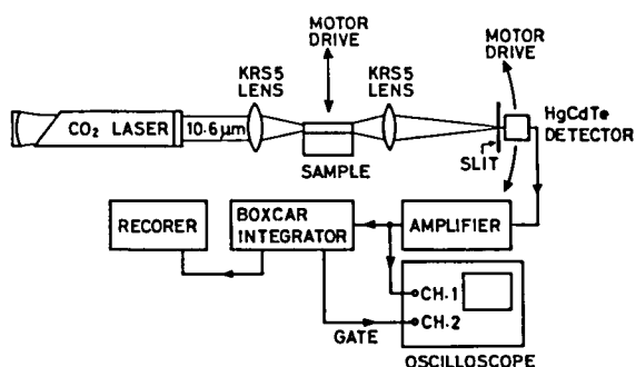
Fig.6.2-2 Experimental setup.
