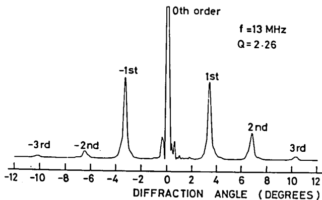
Fig.2.5-4 Angular distribution of the diffracted light intensities. The angles were measured outside the medium.
