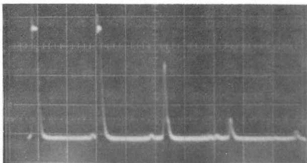
Fig.3.3-2 Acoustic echo train. Horizontal sweep: 5 \mu\text{sec/div.}
