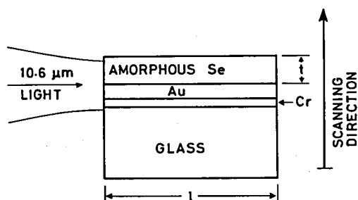
Fig.6.2-1 Structure of the waveguide.
