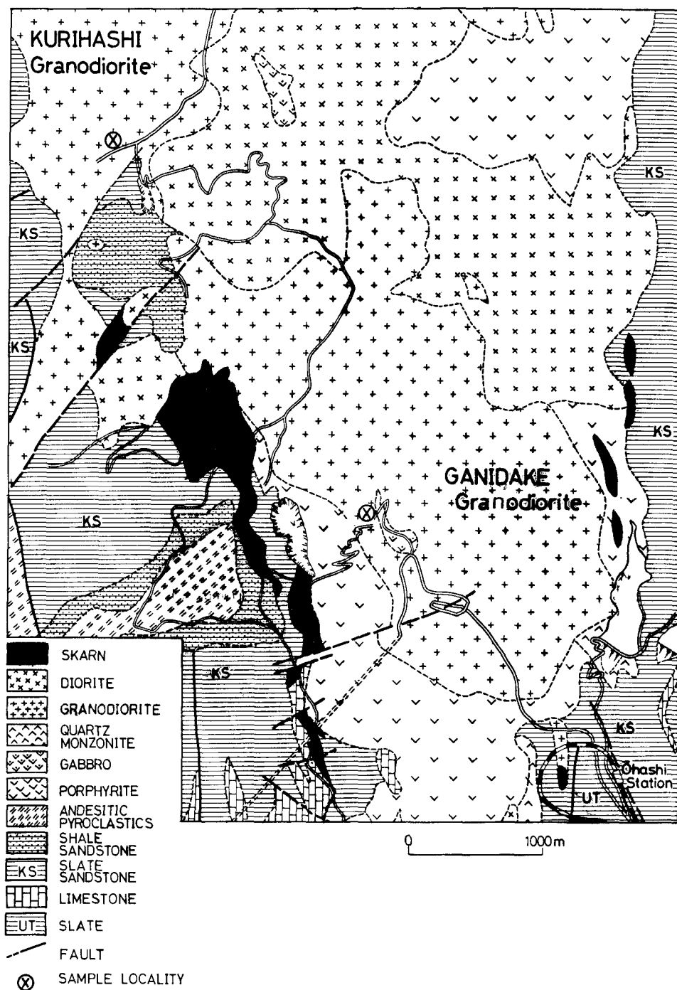
Fig. 1. Geological map of Kamaishi Mine (Nittetsu Mining Co., Ltd., 1973).
