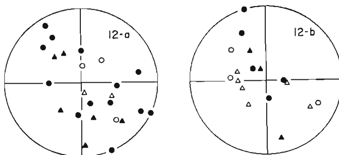
Fig. 25. Fiji (12-a) and Tonga-Kermadec (12-b) regions. ○, △ ; T \leq 5000 min and L \leq 20 km, ●, ▲ ; T \leq 1000 min and L \leq 20 km.
