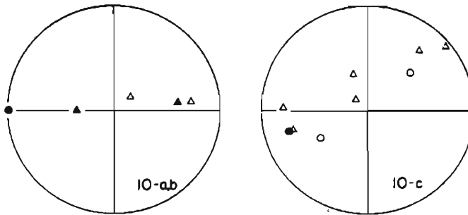
Fig. 17. The directional distributions of subsequent earthquakes in 10-a, b and c areas.
