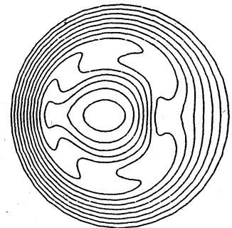
PLASMA PRESSURE PROFILE
