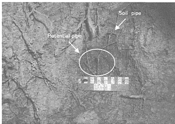
Photo. 2 Part of the potential pipe
