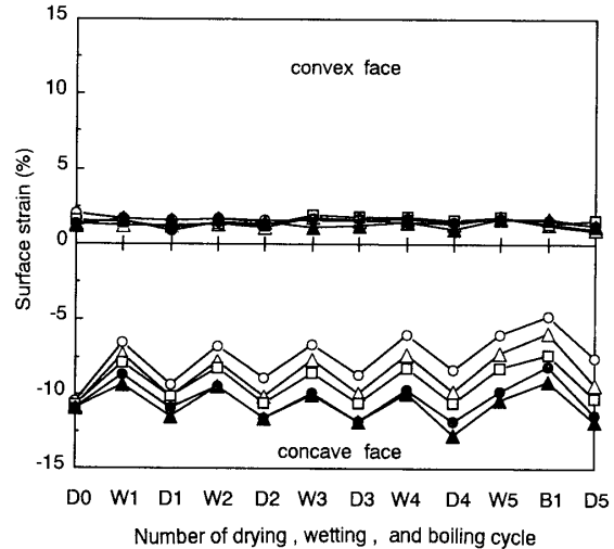
Fig. 12. The recovery of strain of the convex and concave faces for the bends treated at 180°C after wetting (W), ovendrying (D) and boiling (B) test. Treating time ○: 2 hr, △: 4 hr, □: 8 hr, ●: 16 hr, ▲: 32 hr.
