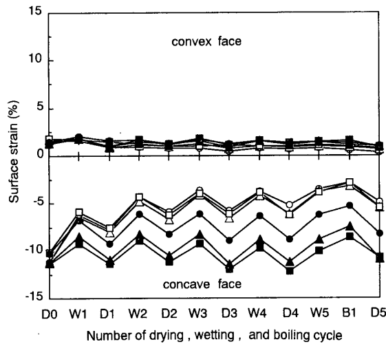
Fig. 11. The recovery of strain of the convex and concave faces for the bends treated at 160°C after wetting (W), ovendrying (D) and boiling (B) test. Treating time ○: 2 hr, △: 4 hr, □: 8 hr, ●: 16 hr, ▲: 32 hr, ■: 64 hr.
