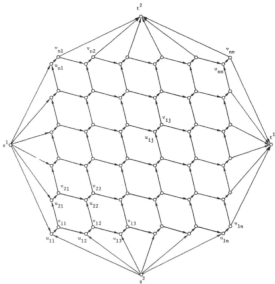
Fig. 5.10 A counterexample to integral flow property.
