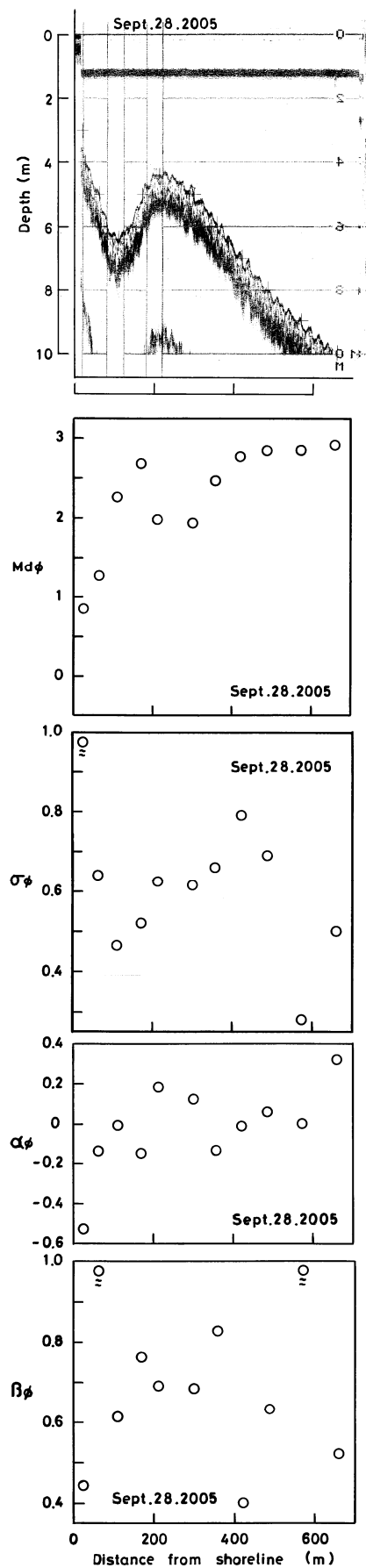
Fig.8 At the jointed measuring line on the crescent-shaped bar, on Sept.28,2005.
