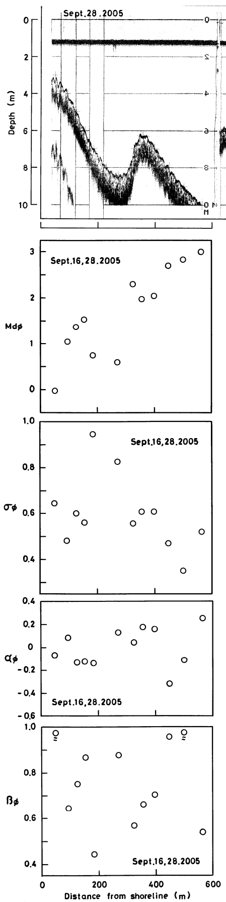
Fig.7 At the central measuring line on the crescent-shaped bar, on Sept.16,28,2005.
