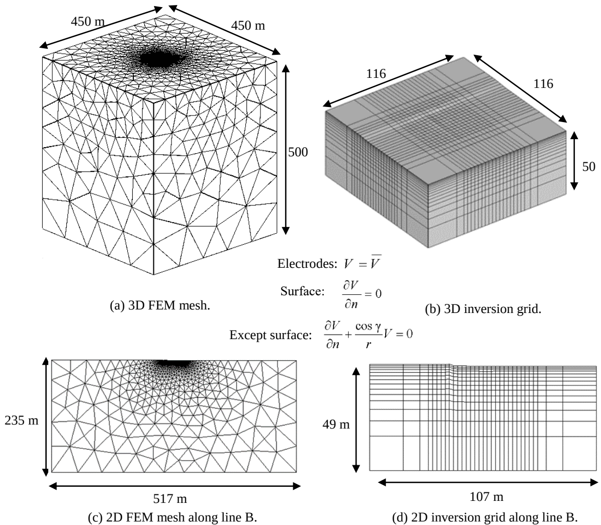
Figure 5.1 Schematic views of the 3D FEM mesh (a) and the inversion grid (b), and 2D FEM mesh (c) and inversion grid (d) along line B.
