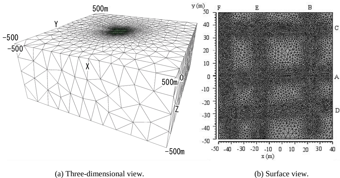
Figure 4.10 (a) Three-dimensional view and (b) surface view of the FEM mesh used to generate synthetic data.
