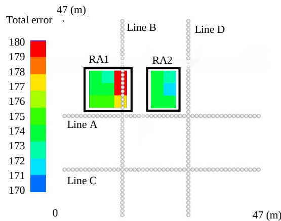
Figure 6.10 Total errors of the observed data in the field against 15 possible models.
