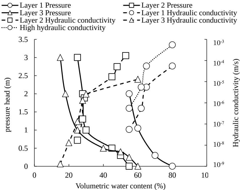
Figure 6.4 Relationship between the unsaturated hydraulic conductivity and the water pressure head against the volumetric water content used in the seepage analysis. The relation is based on the unsaturated flow examination conducted near the survey area (Nakano et al., 1981) and high hydraulic conductivity in layer 1 is assumed to be ten times higher than the hydraulic conductivity of the layer 1.
