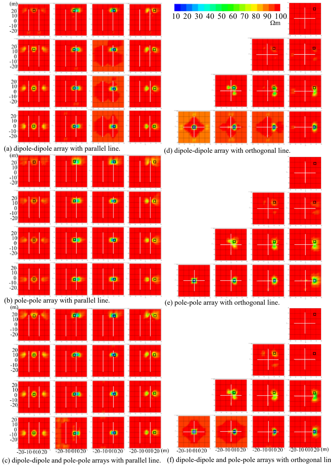
Figure 4.3 A resistivity slice at depth of 4 m reconstructed from 3D inversion of synthetic data obtained along two parallel lines (a, b and c) and two orthogonal lines (d, e and f). The square black box shows the location of the conductive body in the half-space.
