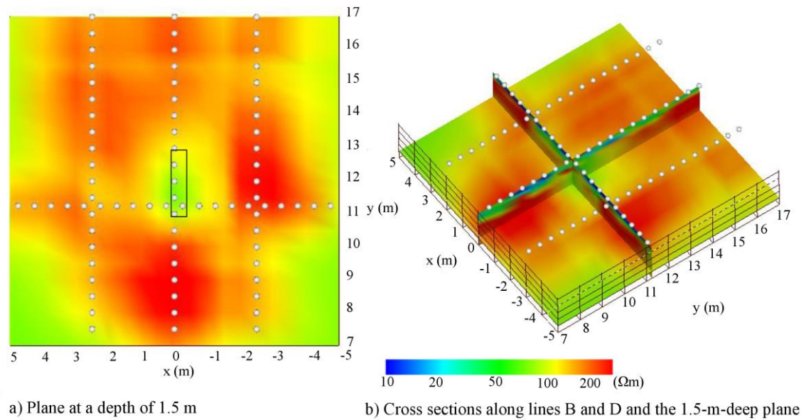
Figure 4.6 Resistivity plane at a depth of 1.5 m and cross sections along lines B and D reconstructed from 3D inversion of synthetic data gathered using 3D and 2D data obtained from the pole-pole and dipole-dipole arrays.
