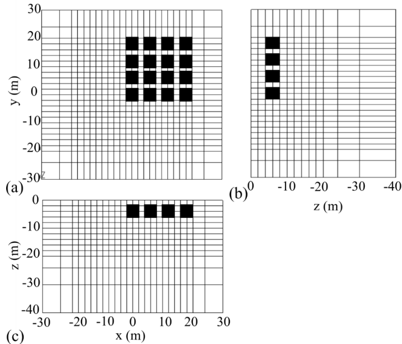
Figure 4.1 (a) x-y, (b) y-z and (c) x-z planes showing a resistivity model. The 16 locations of a conductive 10\ \Omega\text{m} body (black) in a homogeneous 100\ \Omega\text{m} half-space, as shown.
