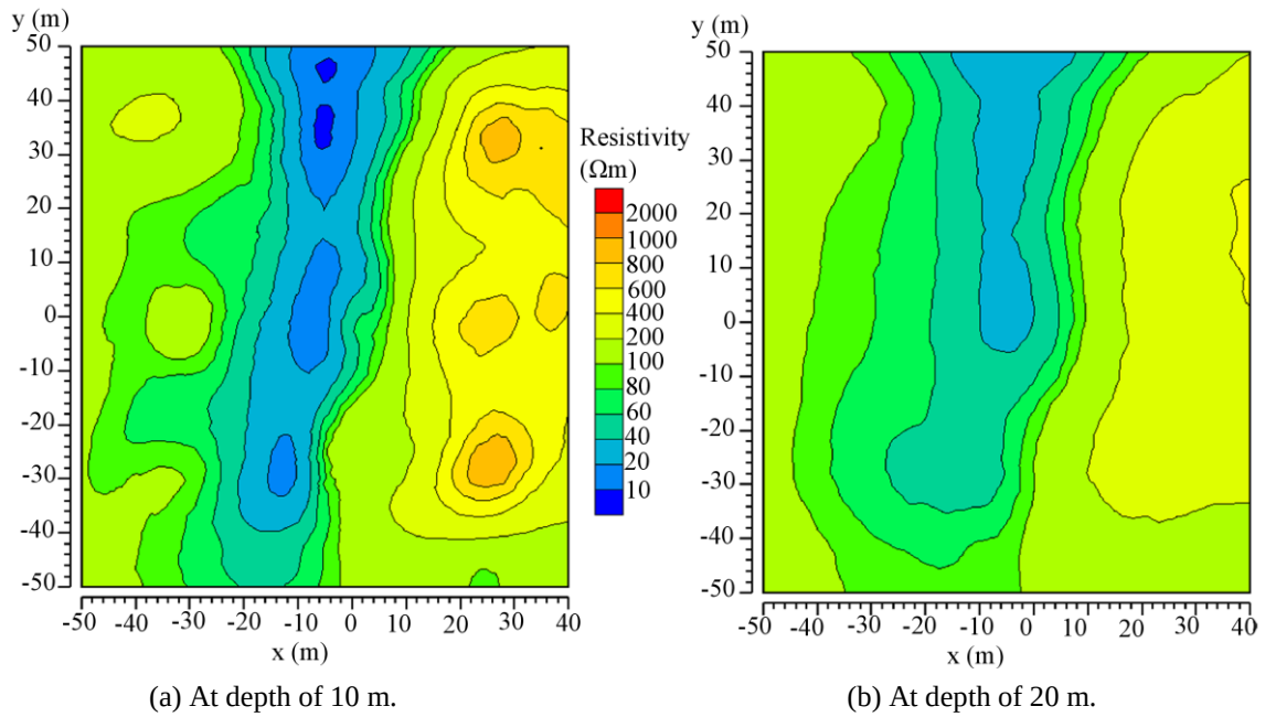
Figure 4.11 Resistivity distributions at depths of (a) 10 m and (b) 20 m reconstructed from 3D inversion of field data gathered using six dipole-dipole arrays.
