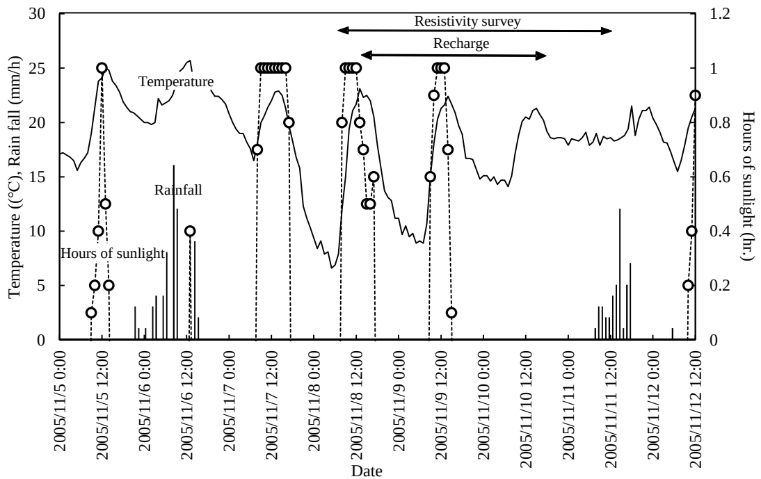
Figure 3.4 Temperature (°C), rainfall (mm/h) and hours of sunlight (h) observed near the survey area from November 5 to November 12, 2005 (Kanoya Magnetic Observatory).
