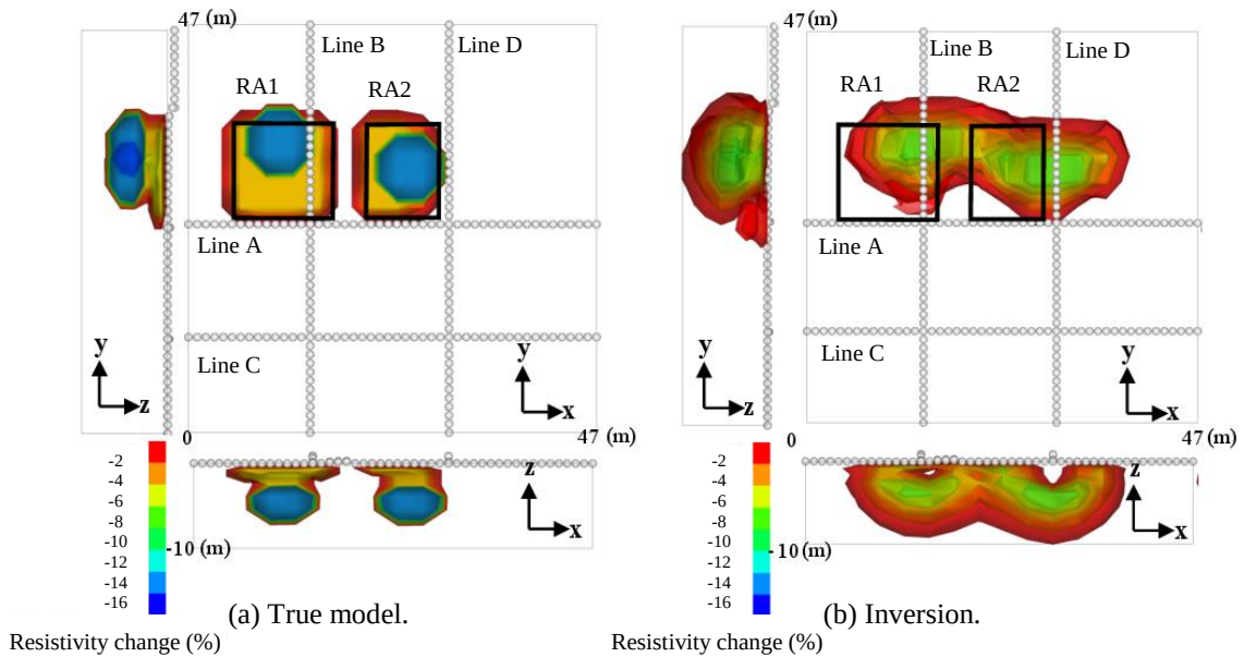
Figure 6.6 Isosurfaces of resistivity change in the numerical field model shown in Figure 6.3: (a) converted from pressure head at 4 hr. after the recharge experiment started, (b) inverted from resistivity data simulated for the water content 0–4 hr. after the recharge started displaying surfaces of constant data value in three dimensions. The transparency level of the isosurfaces is set to 50% to display inner isosurfaces that are obscured by outer isosurfaces. Figures with x-y, z-x and y-z axis are views from z, y and x directions, respectively. Open circles show electrodes.
