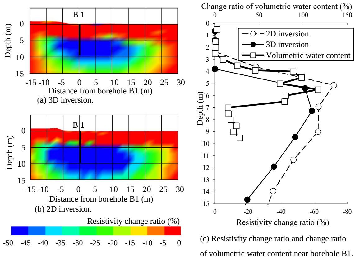
Figure 5.4 Resistivity change ratio sections along line B derived from (a) 3D and (b) 2D inversions of normalized resistivity data and (c) the change ratio of volumetric water content at bore hole B1 and resistivity change ratio near borehole B1 derived from 2D and 3D inversions of normalized resistivity data gathered 52 – 56 hr. after the recharge started (0 – 4 hr. before the recharge terminated). The change ratio of volumetric water content was observed 53 hr. after recharge started and was compared with the volumetric water content before the recharge experiment.
