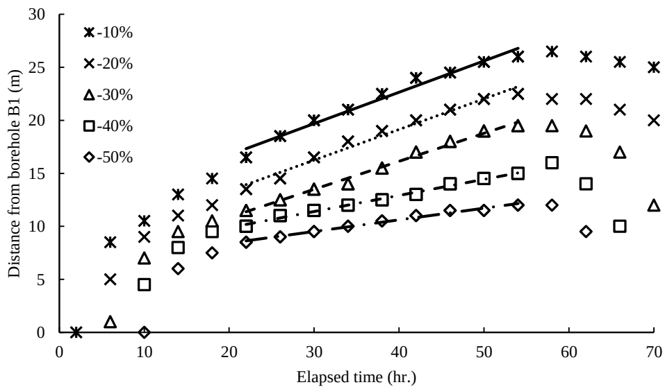
Figure 5.7 Distances of the RCR contour lines in Figure 5.6 from borehole B1 at 7 m depth (positive to the right).
