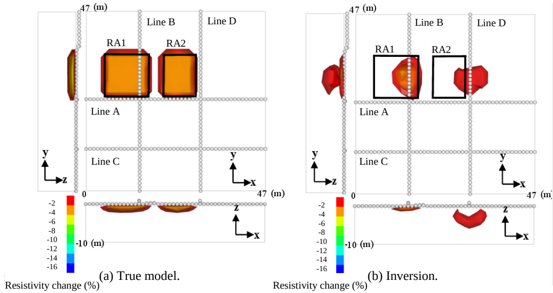
Figure 6.7 Isosurfaces of resistivity change in the model of no high hydraulic conductivity, (a) converted from pressure head at 4 hr. after the recharge experiment started, (b) inverted from resistivity data simulated for the water content 0–4 hr. after the recharge started displaying surfaces of constant data value in three dimensions. The transparency level of the isosurfaces is set to 50% to display inner isosurfaces that are obscured by outer isosurfaces. Figures with x-y, z-x and y-z axis are views from z, y and x directions, respectively. Open circles show electrodes.
