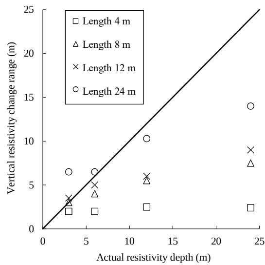
Figure 2.8 Estimated and actual depth of crack along the survey line that is orthogonal to the crack.
