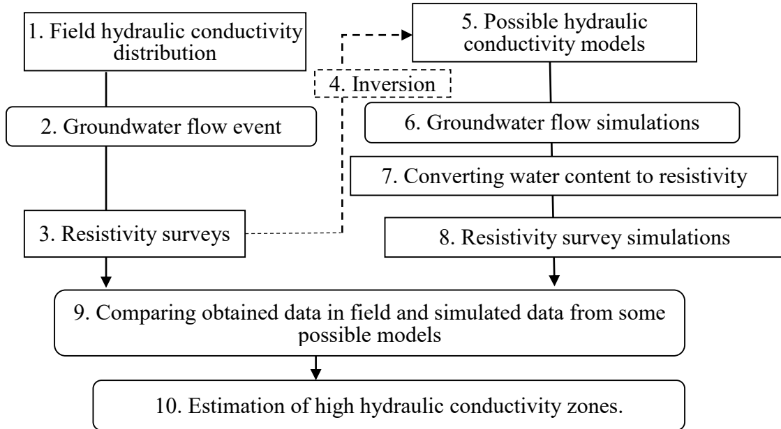
Figure 6.2 Flow to estimate high hydraulic conductivity zones.
