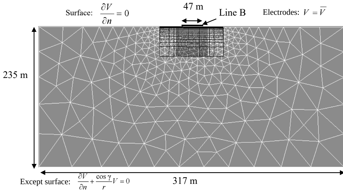
Figure 3.5 FEM mesh and inversion grid along line B.
