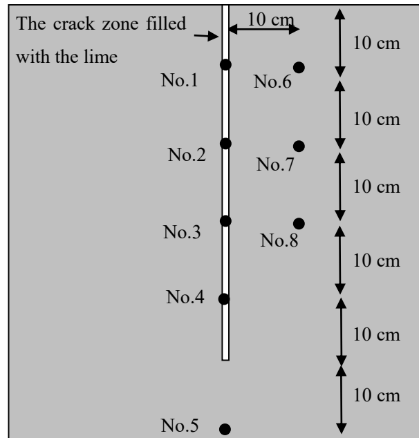
Figure 2.15 Measurement points for apparent resistivity along the cross section.
