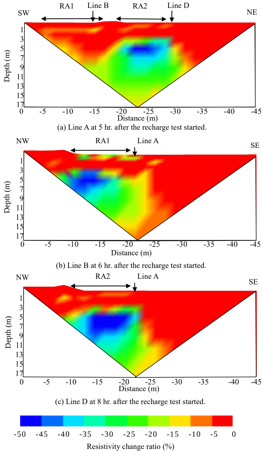
Figure 3.12 Distribution of the resistivity change ratio at (a) 5 hr., (b) 6 hr. and (c) 8 hr. after the recharge test started.
