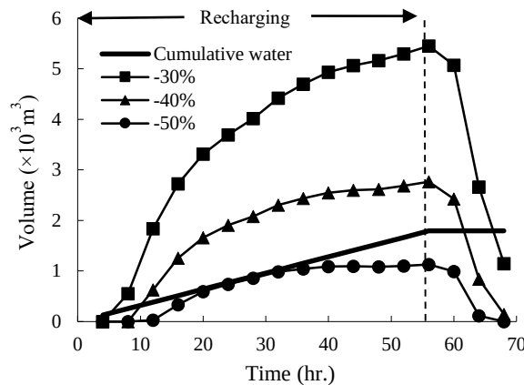
Figure 5.8 Cumulative water supplied (thick line) and variations in volumes of RCR of -30\% (rectangles), -40\% (triangles), and -50\% (circles) in the recharge experiment.
