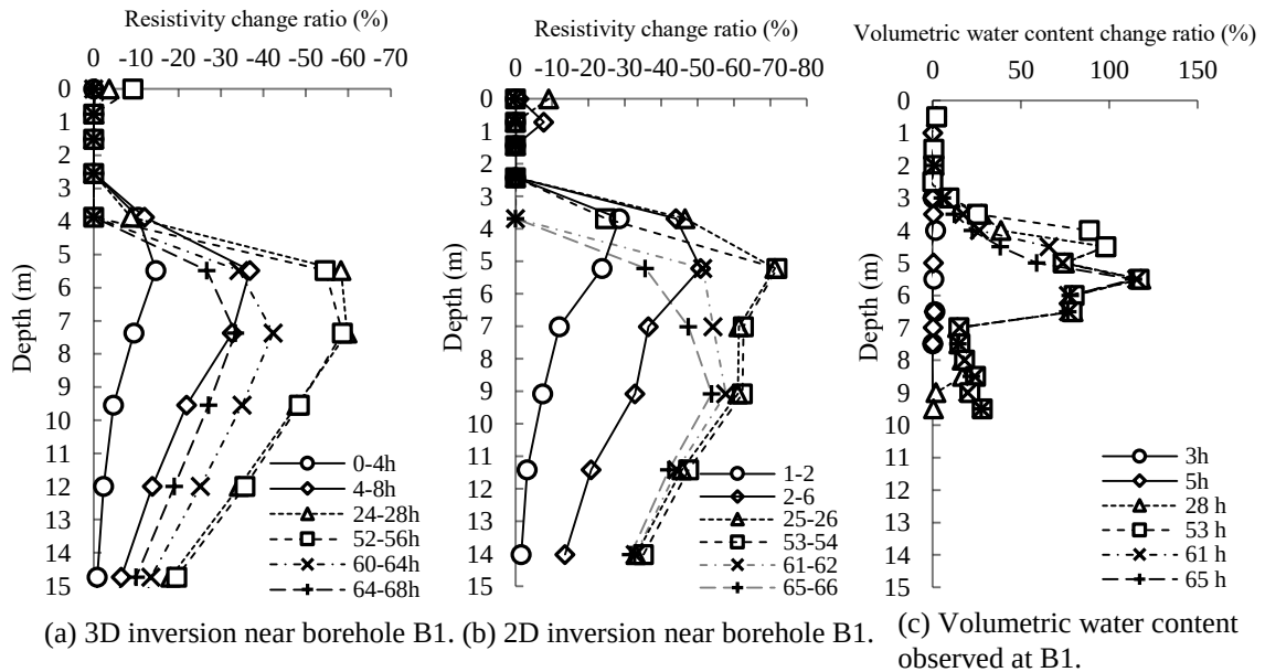
Figure 5.5 Profiles of the RCR and the volumetric water content change ratio. (a) 3D RCR near borehole B1, (b) 2D RCR near borehole B1, and (c) volumetric water content at borehole B1.
