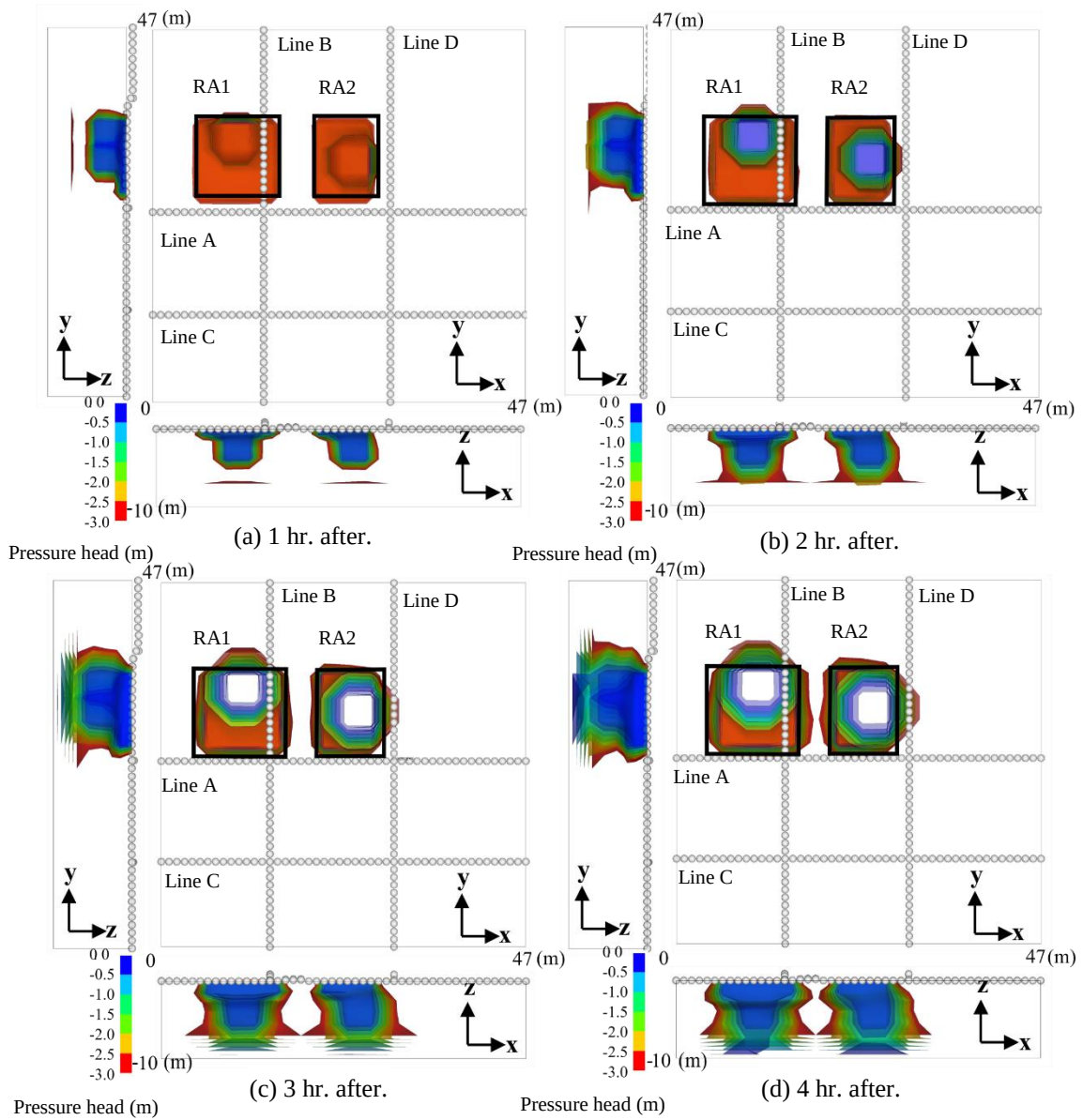
Figure 6.5 Isosurfaces of pressure head at (a) 1 hr., (b) 2 hr., (c) 3 hr. and (d) 4 hr. after the recharge started. displaying surfaces of constant data value in three dimensions. The transparency level of the isosurfaces is set to 50% to display inner isosurfaces that are obscured by outer isosurfaces. Figures with x-y, z-x and y-z axis are views from z, y and x directions, respectively. Open circles show electrodes.
