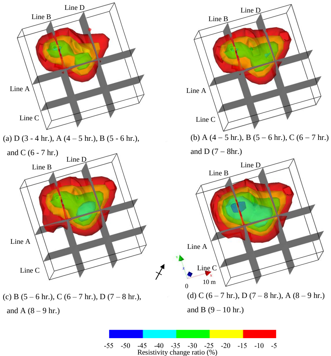
Figure 5.10 Change in the volume of resistivity change ratio derived from 3D inversion of resistivity data collected (a) 3 – 7 hr., (b) 4 – 8 hr., (c) 5 – 9 hr., and (d) 6 – 10 hr. after the recharge experiment started.
