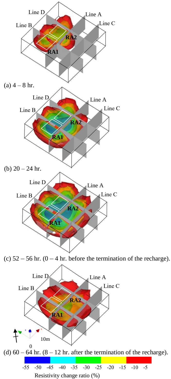
Figure 5.9 Change in the volume of resistivity change ratio derived from 3D inversion of resistivity data measured (a) 4 – 8 hr., (b) 20 – 24 hr., (c) 52 – 56 hr. and (d) 60 – 64 hr. after the recharge experiment started.
