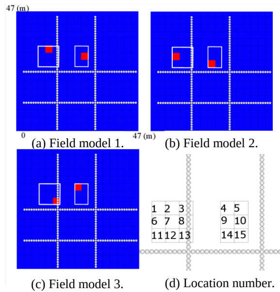
Figure 6.8 High hydraulic conductivity models. (a), (b) and (c) are numerical field models and (d) is the location number in recharge areas and the location of the high hydraulic conductivity zone at each possible model. Possible model 1 has a hydraulic conductivity zone at location 1, possible models 2 – 15 have a hydraulic conductivity zone at location 2 – 15, respectively. Field models 1, 2 and 3 have two hydraulic conductivity zones at locations 6 and 14, 2 and 10, and 13 and 4, respectively.
