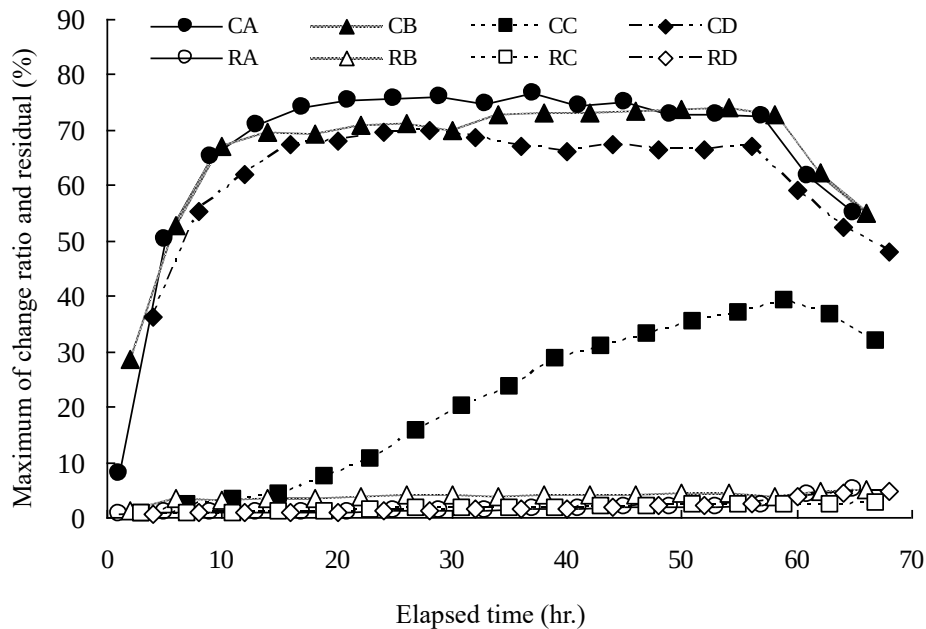
Figure 3.11 The maximum levels for the resistivity change ratios and residuals levels of the inversions in the inverted resistivity sections along the survey line for each time. CA – CD: Maximums levels of the resistivity change ratios along lines A – D. RA – RD: Residual levels of the inversions of lines A – D.
