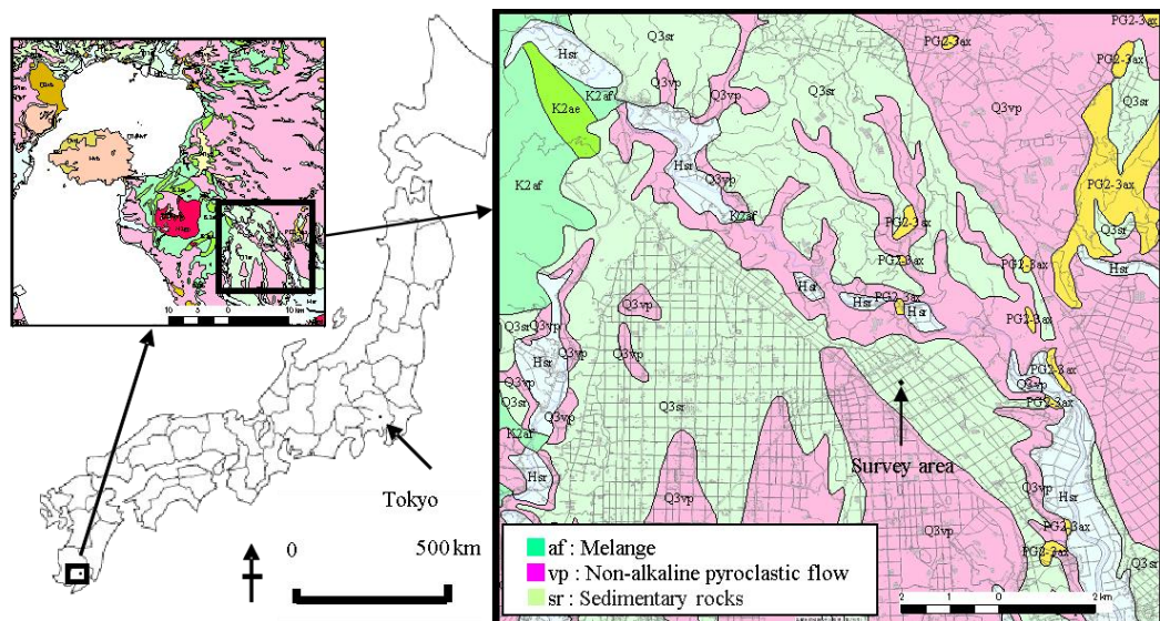
Figure 3.1 Location of the survey area and geological map (Geological Survey of Japan, AIST (ed.), 2014).
