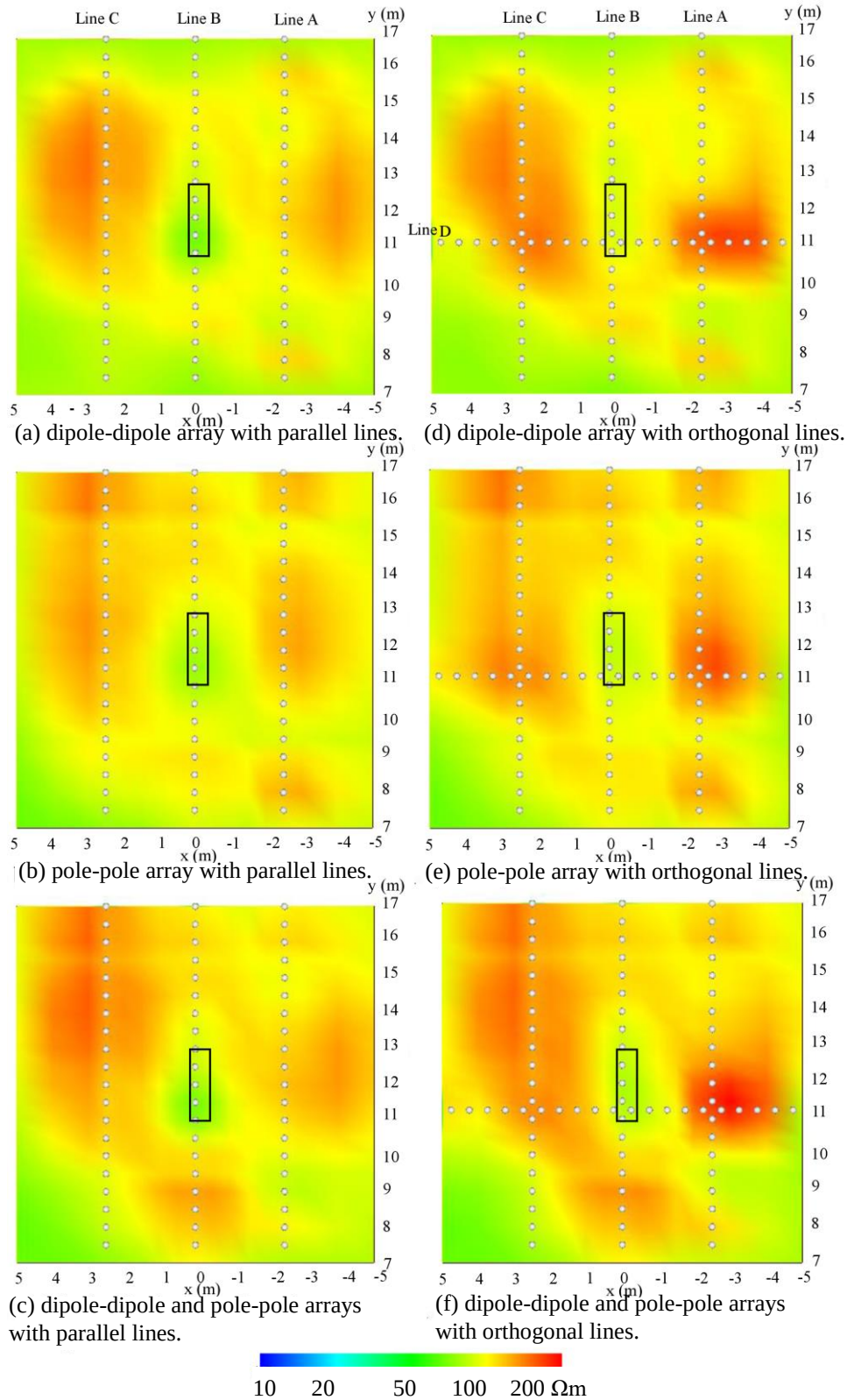
Figure 4.7 Resistivity plane at a depth of 1.5 m with (a, b and c) three parallel lines and (d, e and f) four lines including an orthogonal line.
