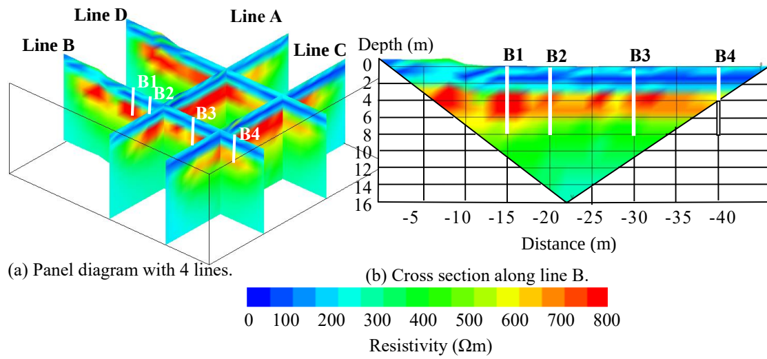
Figure 3.8 Inverted resistivity distribution before the recharge test. (a) Panel diagram with 4 lines. (b) Cross section along survey line B.
