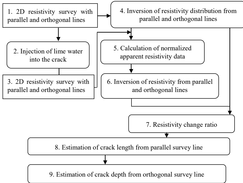
Figure 2.2 Flow of the proposed method illustrating the steps.
