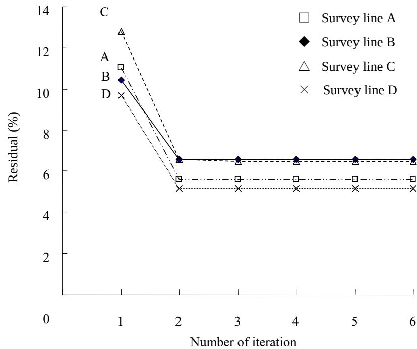
Figure 3.9 Residual levels at each iterations of the resistivity inversion before the recharge test started. A – D: Residual levels of the inversions of survey lines A – D.
