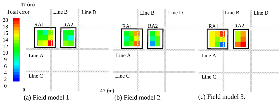
Figure 6.9 Total errors of observed resistivity data in (a) field model 1 in Figure 6.8 (a), (b) field model 2 in Figure 6.8 (b) and (c) field model 3 in Figure 6.8 (c) against resistivity data of 15 possible models shown in Figure 6.8 (d).
