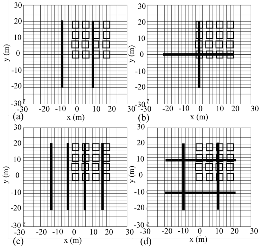
Figure 4.2 Survey lines on the surface: (a) two parallel, (b) two orthogonal, (c) four parallel and (d) four orthogonal lines.
