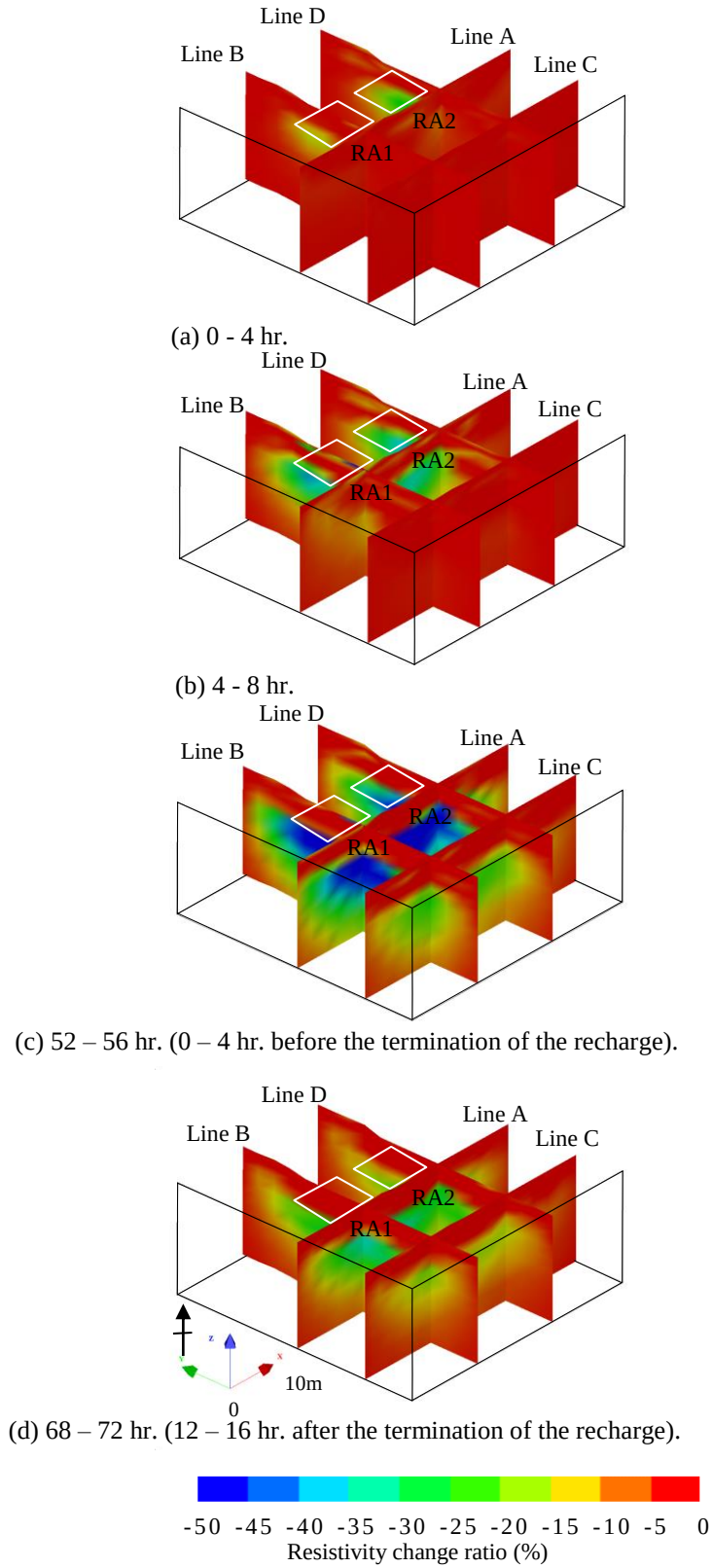
Figure 5.3 Resistivity change ratio distributions. (a) 0 – 4 hr., (b) 4 – 8 hr., (c) 52 – 56 hr. and (d) 68 – 72 hr. after the recharge experiment started.
