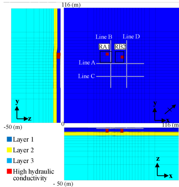
Figure 6.3 Projection view of FEM mesh for seepage analysis and resistivity survey lines. White dotted lines show four resistivity 2D resistivity survey lines. The smallest mesh size is 3 m in the horizontal direction and 1 m in the vertical direction. This mesh size is same with grid size of inversion of resistivity and it is easy to convert water content to resistivity. All nodes are initially set at -10 m of the hydraulic total head. Surface nodes in the recharge areas have the pressure head at 0.3 m during the recharge experiment. The surface of the site is inclined slightly from north-west to south-east.
