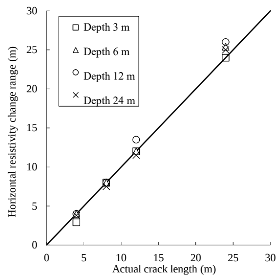
Figure 2.6 Estimated and actual length of crack along survey line that is parallel to the crack.
