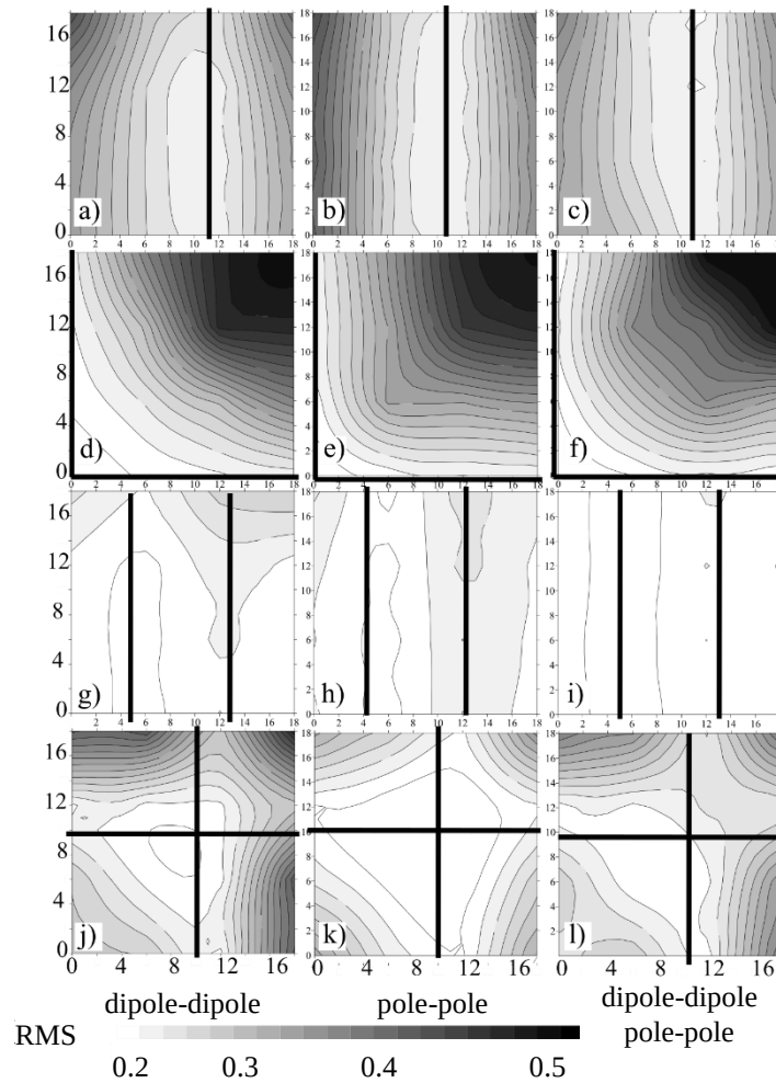
Figure 4.5 Map of RMS error in resistivity for (a, b and c) two parallel lines, (d, e and f) two orthogonal lines, (g, h and i) four parallel lines and (j, k and l) four orthogonal lines. Only the first quadrant of the contour map is shown. The RMS error is assigned to the position of body.
