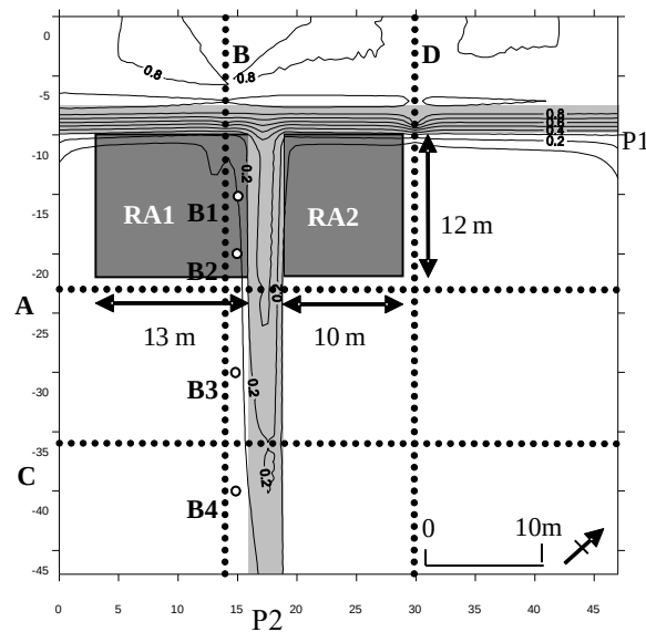
Figure 3.2 Survey area where the groundwater recharge experiment was conducted. Four lines A, B, C and D (black dots), four boreholes B1, B2, B3 and B4 (white dot), and two recharge areas RA1 (12 m × 13 m) and RA2 (12 m × 10 m) were set up in the area. Symbols P1 and P2 indicate the roads in the survey area.
