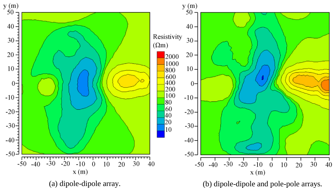
Figure 4.12 Resistivity distributions at depths of 10 m reconstructed from 3D inversion of field data gathered using (a) two dipole-dipole arrays and (b) two pole-pole and dipole-dipole arrays.
