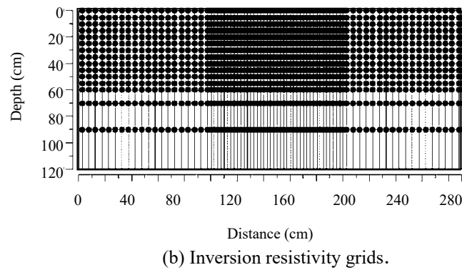
Figure 2.10 FEM mesh and inversion resistivity grid.
