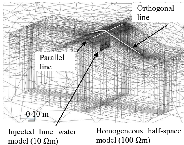
Figure 2.4 FEM mesh incorporating the resistivity model in the numerical experiment (after injection of lime water).
