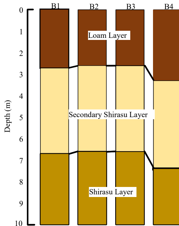
Figure 3.3 Logs of boreholes B1, B2, B3 and B4 shown in Figure 3.2. The loam layer, the secondary Shirasu layer (lacustrine or marine sediments of pyroclastic origin), and the Shirasu layer (pyroclastic) were observed in order of depth.
