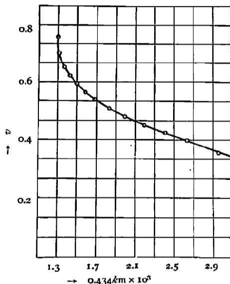
Fig. 3. Chemisorption of carbon dioxide by catalyst III at 370°C.
