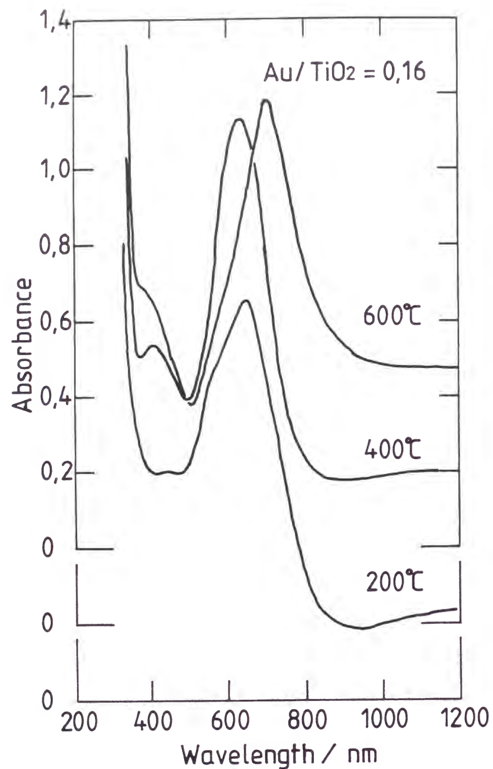
Fig.3 Optical absorption spectra of surface-wiped Au:TiO 2 films heat-treated at 200° , 400° and 600° C. A small and broad increase of absorbance from 500 to 1200nm in pure TiO 2 is due to the interference of light by the film with high refractive index.
