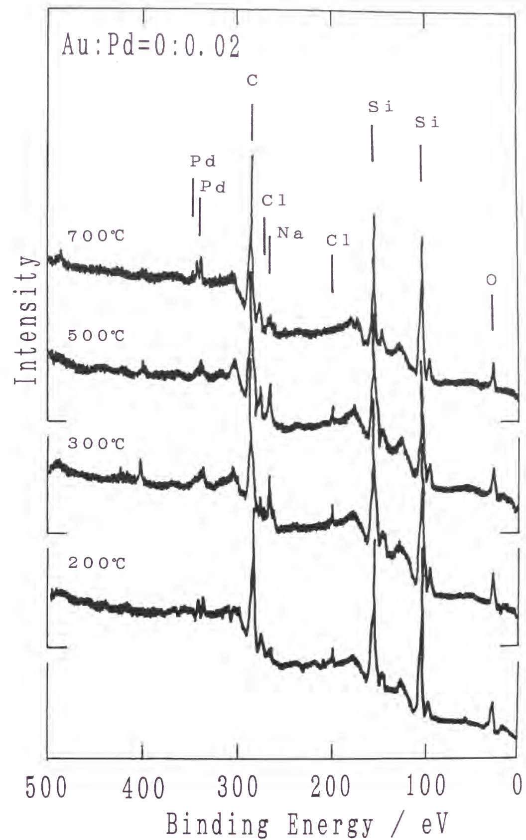
Fig.6(c) Wide range X-ray photoelectron spectra of Pd-doped films heat-treated at a temperature from 200° to 700° C.
