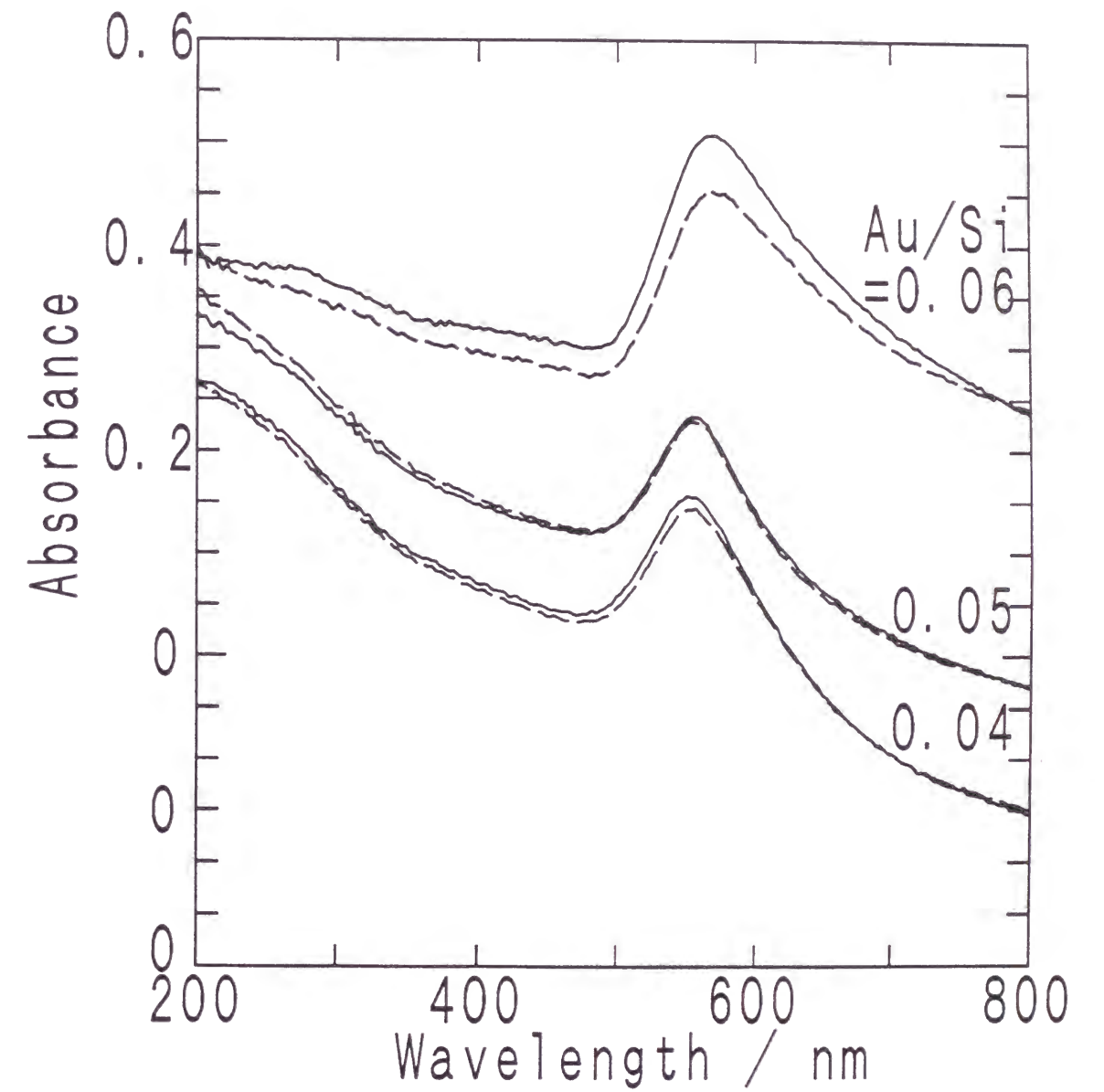
Fig.1(c) Optical absorption spectra of as-prepared (solid line) and surface wiped (dashed line) films with different Au/Si molar ratio and \text{NaNO}_3/\text{TEOS} = 0.06 .
