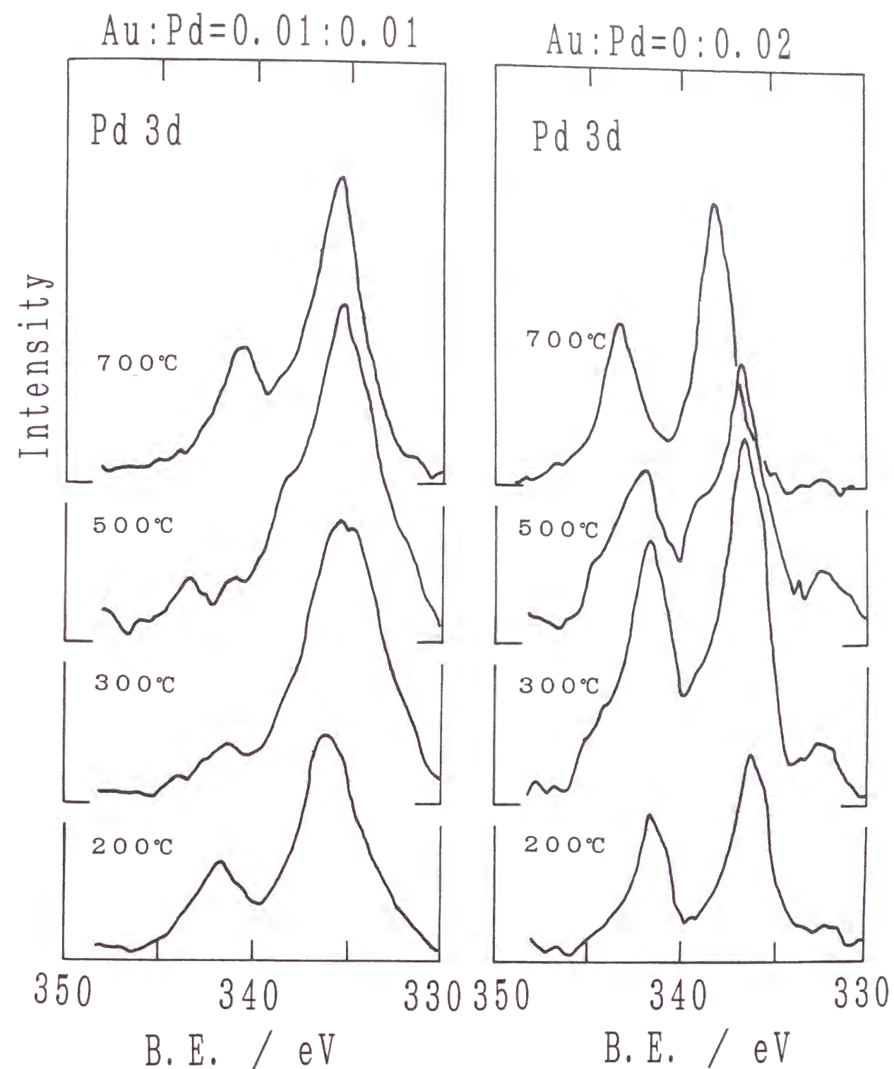
Fig.7(b) Pd-3d (b) X-ray photoelectron spectra of Au-Pd co-doped and Pd-doped films heat treated at a temperature from 200° to 700°C.
