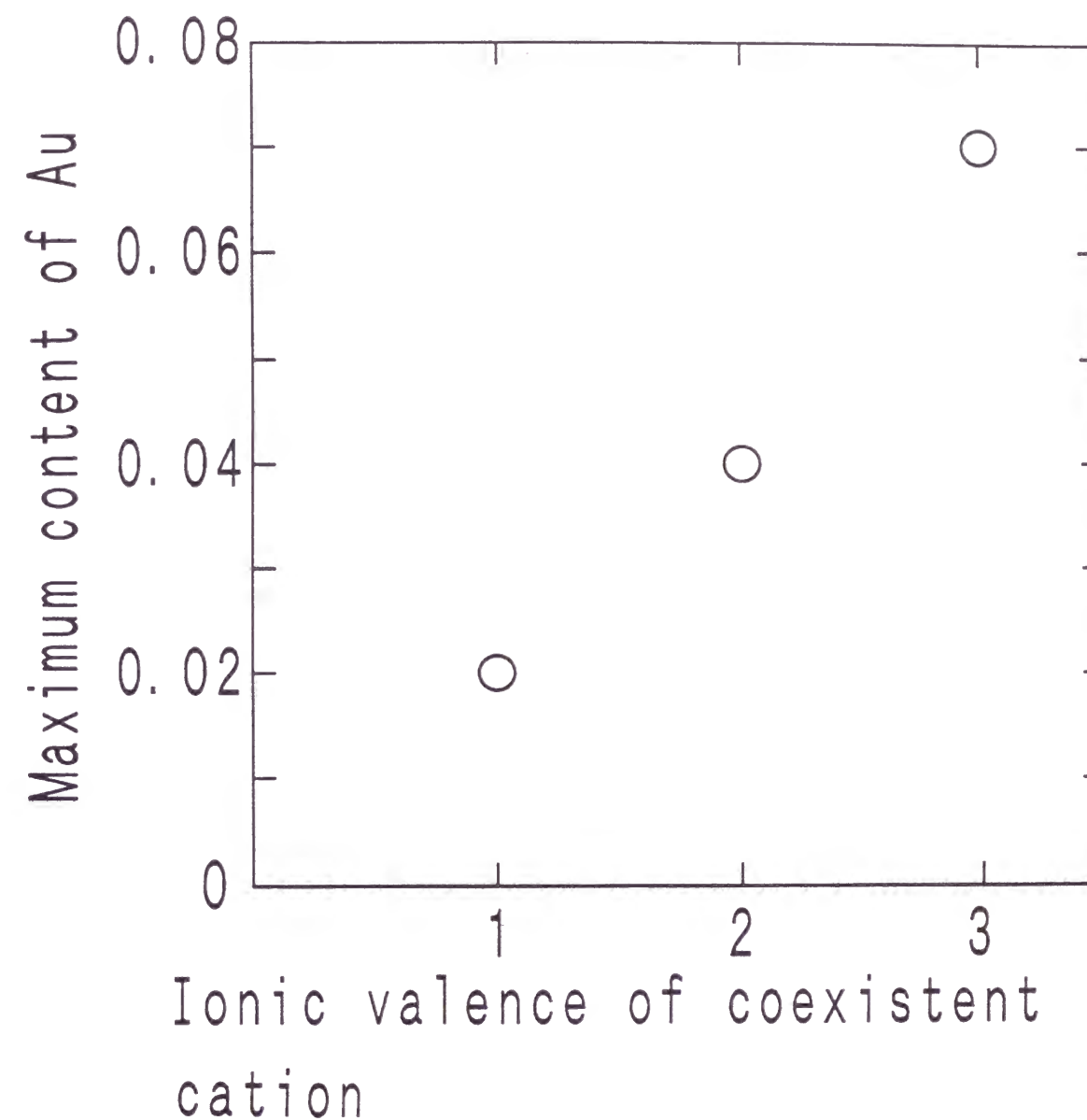
Fig.4 The maximum amount of gold microcrystals incorporated in the films prepared from dip-coating solutions containing \text{M}(\text{NO}_3)_n ( \text{M}=\text{Na} , \text{Ca} , and \text{La} ) with the molar concentration of \text{M}(\text{NO}_3)_n/\text{TEOS} = 0.01 .
