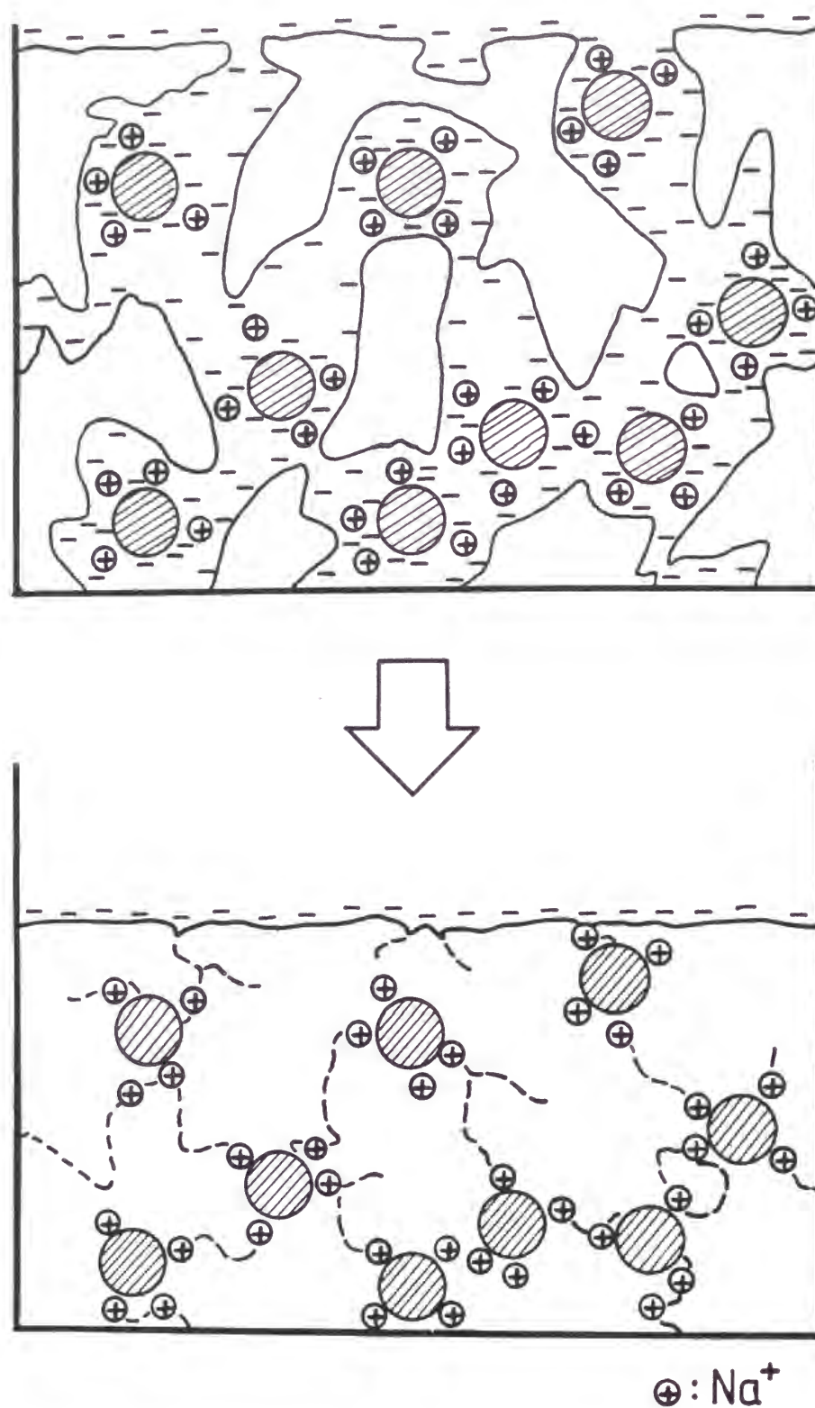
Fig.5(b) Schematic diagram of the sintering process of \text{AuCl}_4^- -contained \text{SiO}_2 gel films containing \text{Na}^+ ions. Shaded circles are \text{AuCl}_4^- ions, and small circles are \text{Na}^+ ions.
