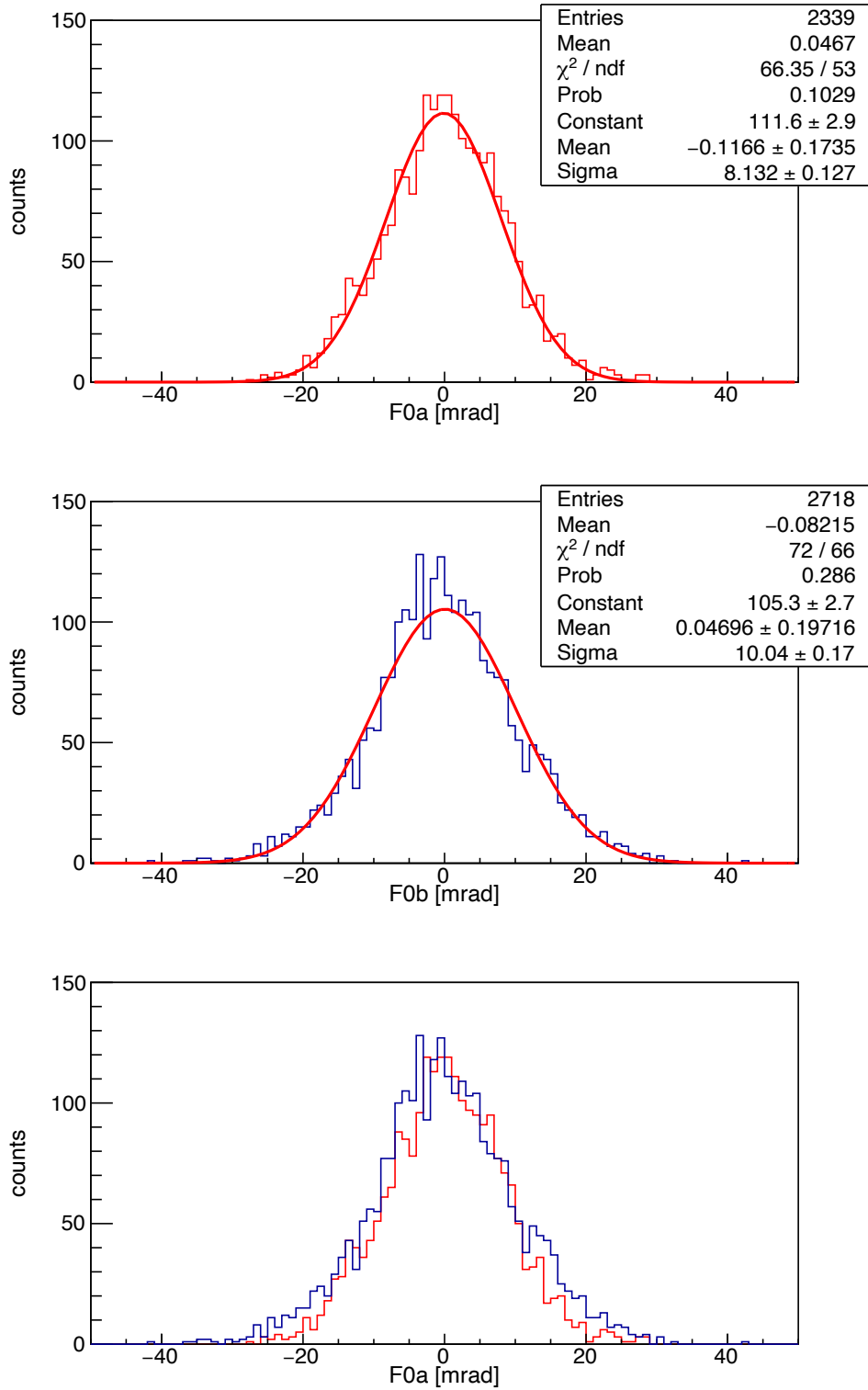
Figure 3.19: The projection of the reconstructed distribution of the horizontal angles and the vertical angles deduced with the original values of (a|a)_{F0 \rightarrow F5} and (b|b)_{F0 \rightarrow F5} . Top panel: F0a, middle panel: F0b, bottom panel: F0a and F0b are overlaid.
