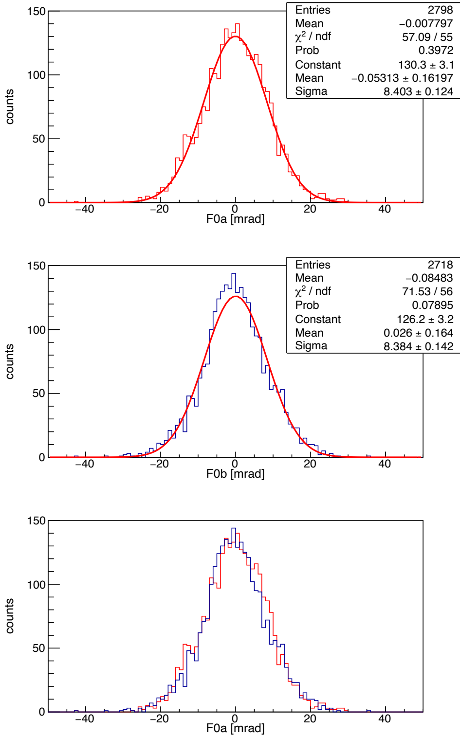
Figure 3.21: Same as Fig. 3.19 but the (b|b)_{F0 \rightarrow F5} is scaled by 1.18.
