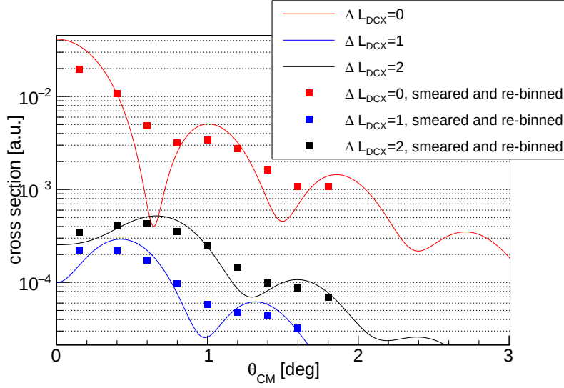
Figure B.1: Calculated angular distribution of \Delta L_{\text{DCX}} = 0, 1, 2 (before smearing) and re-binned points for angular region used in MDA after smearing. Red, blue, and black lines and points correspond to \Delta L_{\text{DCX}} = 0, 1 , and 2 transition, respectively.
