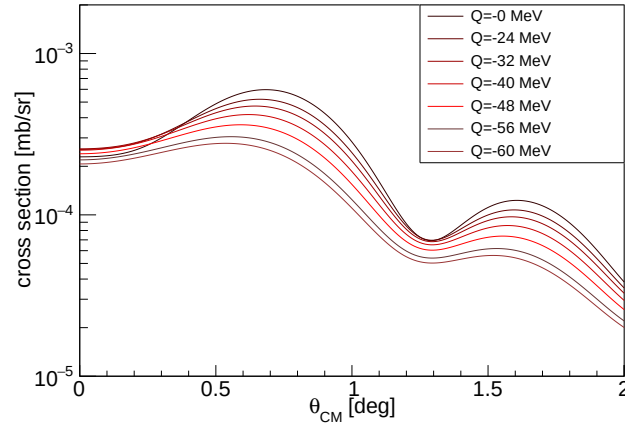
Figure B.4: Angular distributions of \Delta L_{\text{DCX}} = 2 calculated with different Q -values.
