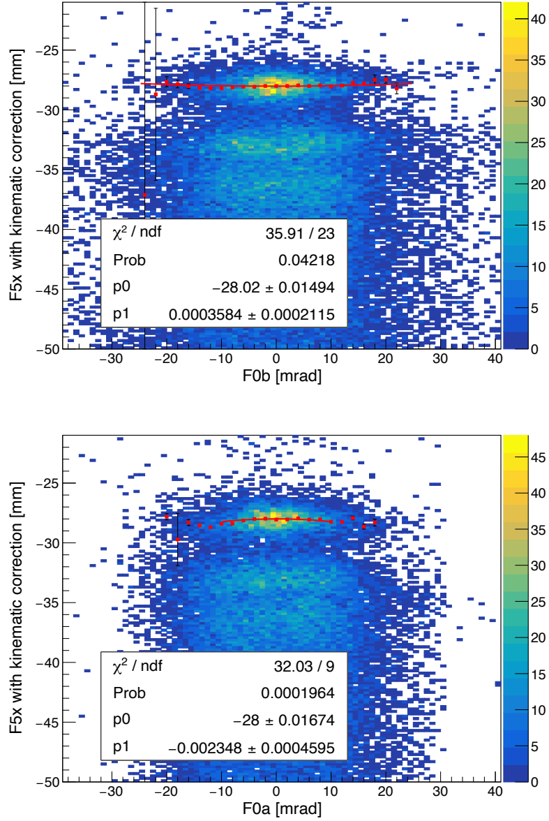
Figure 3.23: Correlation between the reconstructed angle and the horizontal position at F5 after correction of the scale. Top: correlation with the vertical angle F0b, bottom: the horizontal angle F0a.
