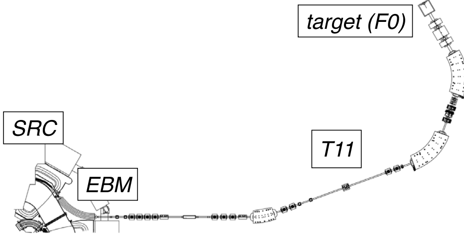
Figure 2.6: Schematic view of the beam line from SRC to target (F0). This is taken from Ref. [6].
