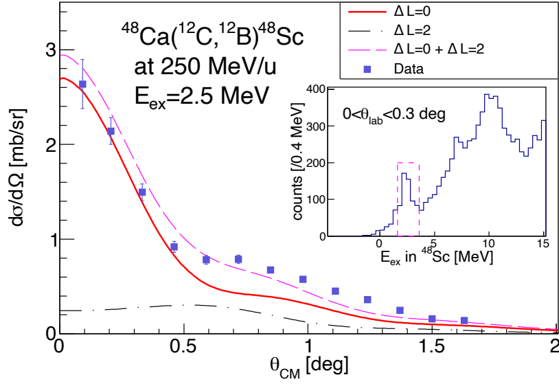
Figure 4.8: Angular distribution for the SCX reaction of ^{48}\text{Ca}(^{12}\text{C}, ^{12}\text{B})^{48}\text{Sc} around E_{\text{ex}} = 2.5 MeV. Red and black curves are calculated angular distributions using ECIS for \Delta L = 0 and \Delta L = 2 , respectively. Magenta curve is the sum of \Delta L = 0 and \Delta L = 2 . The inset shows the observed counts at \theta_{\text{lab}} = 0^\circ\text{--}0.3^\circ against the excitation energy in ^{48}\text{Sc} .
