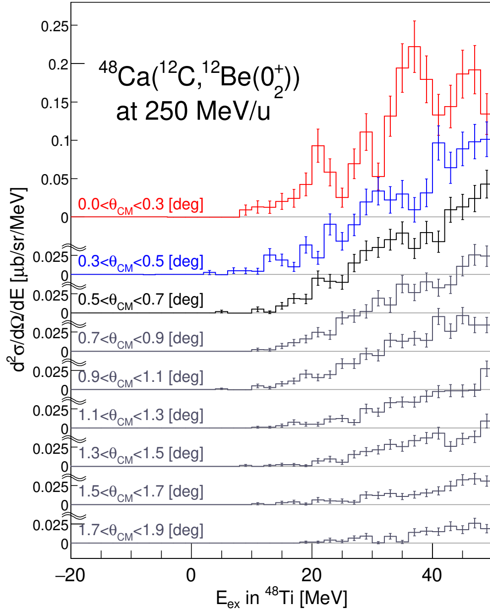
Figure 3.31: Double-differential cross sections of the ^{48}\text{Ca}(^{12}\text{C}, ^{12}\text{Be}(0_2^+))^{48}\text{Ti} reaction against the excitation energy in ^{48}\text{Ti} for each angle from 0.0^\circ to 1.9^\circ .
