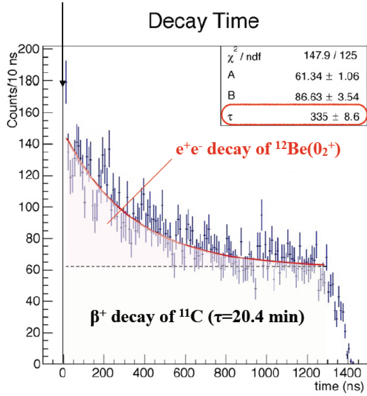
Figure 1.6: The timing of the \gamma -rays measured by the NaI scintillator array in the experiment of ( ^{12}\text{C} , ^{12}\text{Be}(0_2^+) ) performed at RCNP [3].
