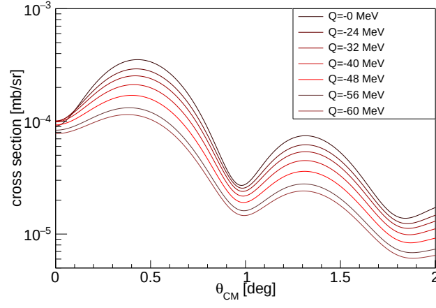
Figure B.3: Angular distributions of \Delta L_{\text{DCX}} = 1 calculated with different Q -values.
