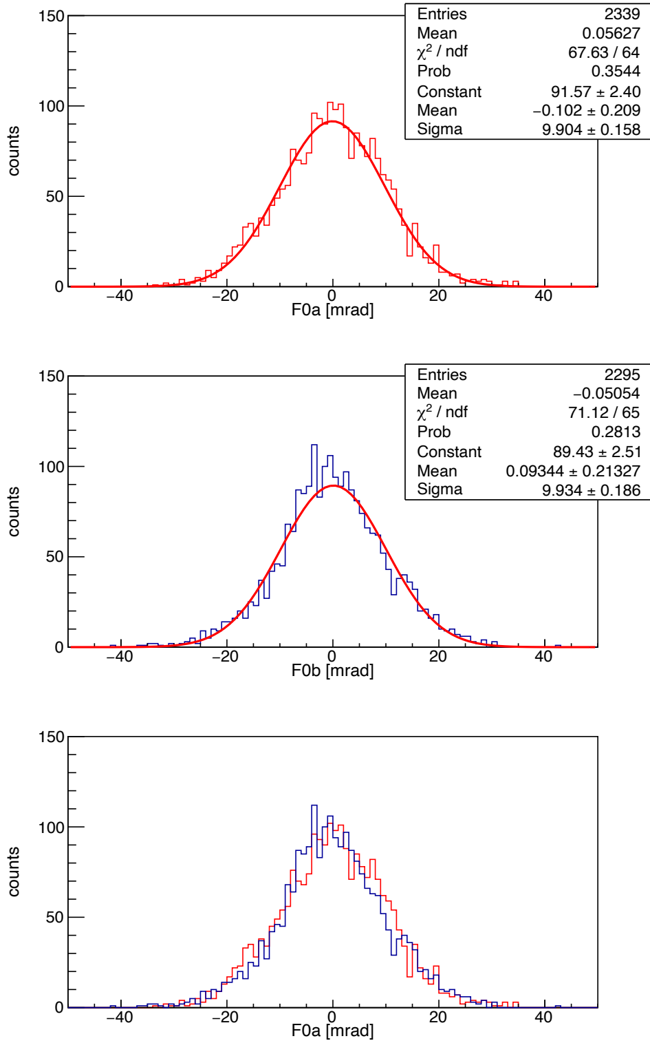
Figure 3.20: Same as Fig. 3.19 but the (a|a)_{F0 \rightarrow F5} is scaled by 0.85.
