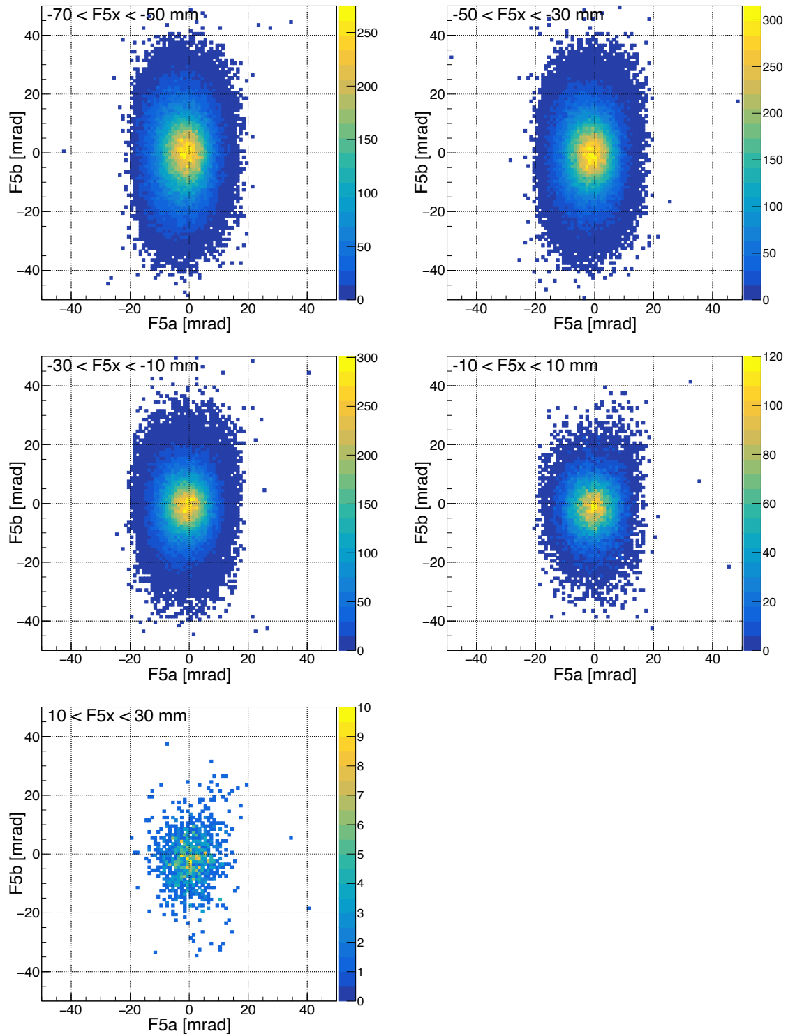
Figure 3.10: Measured angular distribution at F5 at each region of the horizontal position at F5.
