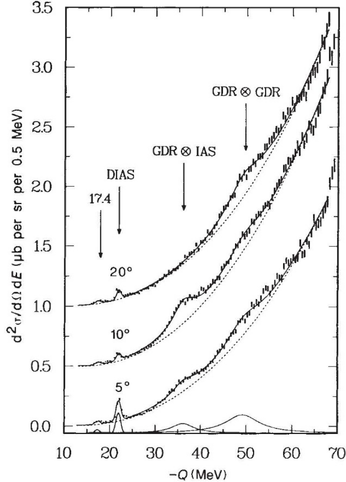
Figure 1.1: Double differential cross section for the (\pi^+, \pi^-) reaction on ^{93}\text{Nb} target at T_\pi = 295 \text{ MeV} and \theta_{\text{lab}} = 5^\circ, 10^\circ , and 20^\circ [1].
