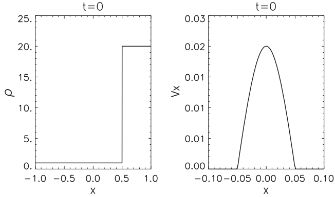
Figure 8. Initial profile of the density (left) and velocity (right) for a quasilinear case with \rho_p = 20 .
