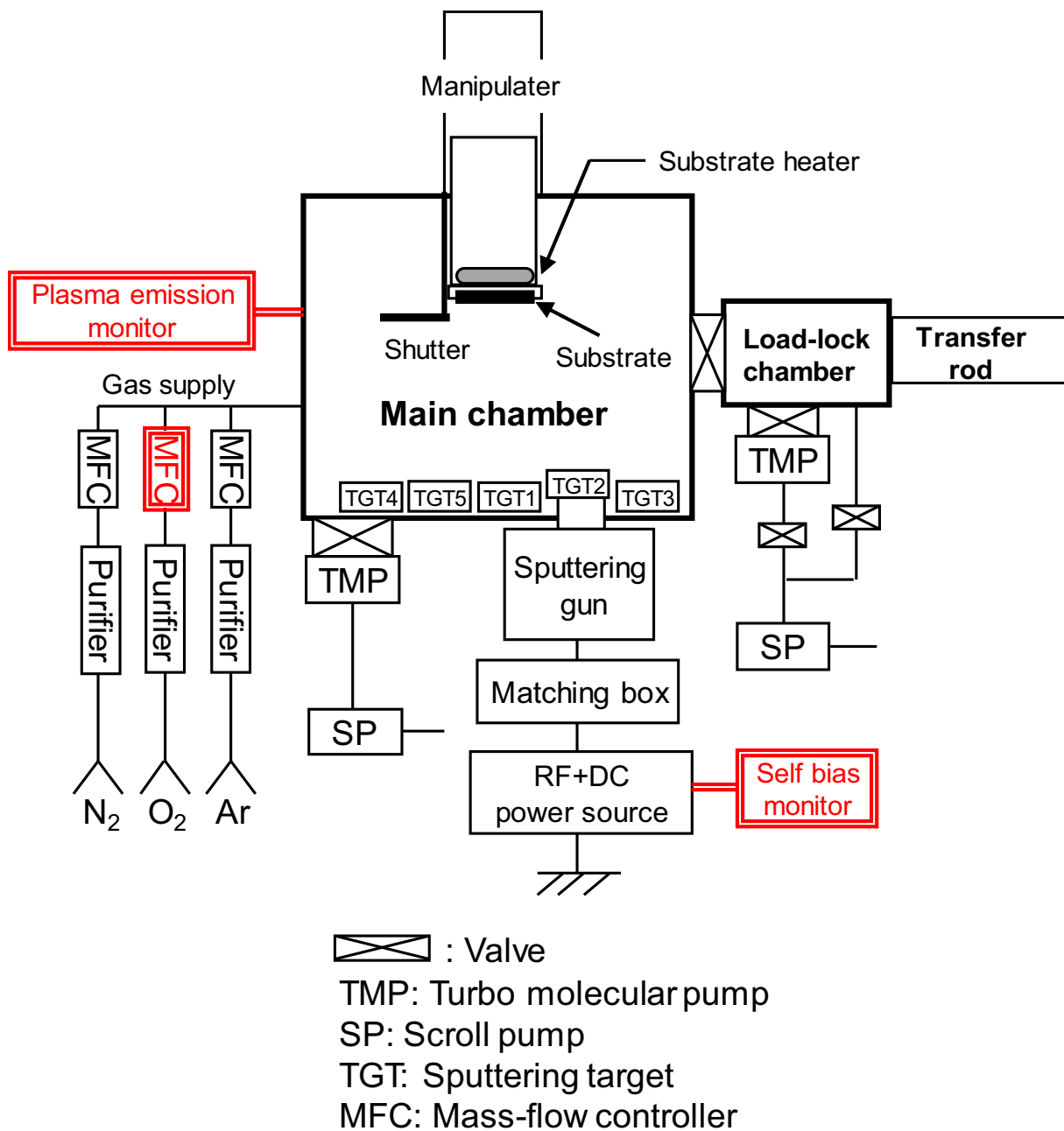
Figure 2.4: A schematic illustration of the sputtering system for \text{TiO}_2 deposition.
