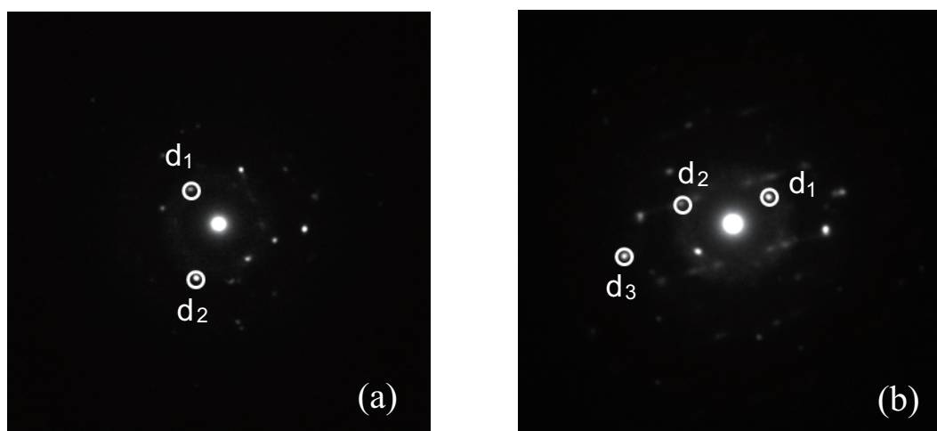
Figure 4.16: Selected area electron diffraction (SAED) patterns of (a) an area of TiO 2 at a distance approximately 60 nm from the TiO 2 /Pt interface and (b) an area of TiO 2 near the interface of the EB-Pt sample. Several diffraction spots of d 1 , d 2 , and d 3 indicate rutile-type TiO 2 (110), (101), and (310), respectively.
