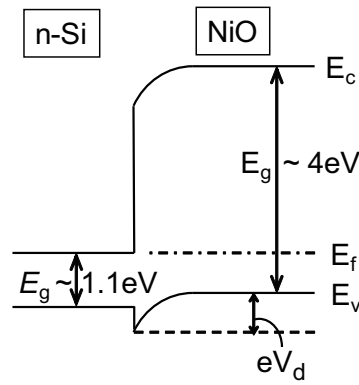
Figure 3.2: The band diagram of pn junction between p -type \text{NiO} and n -type \text{Si} .
