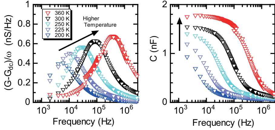
(a) p\text{-NiO}_{1.05}/n\text{-Si}
