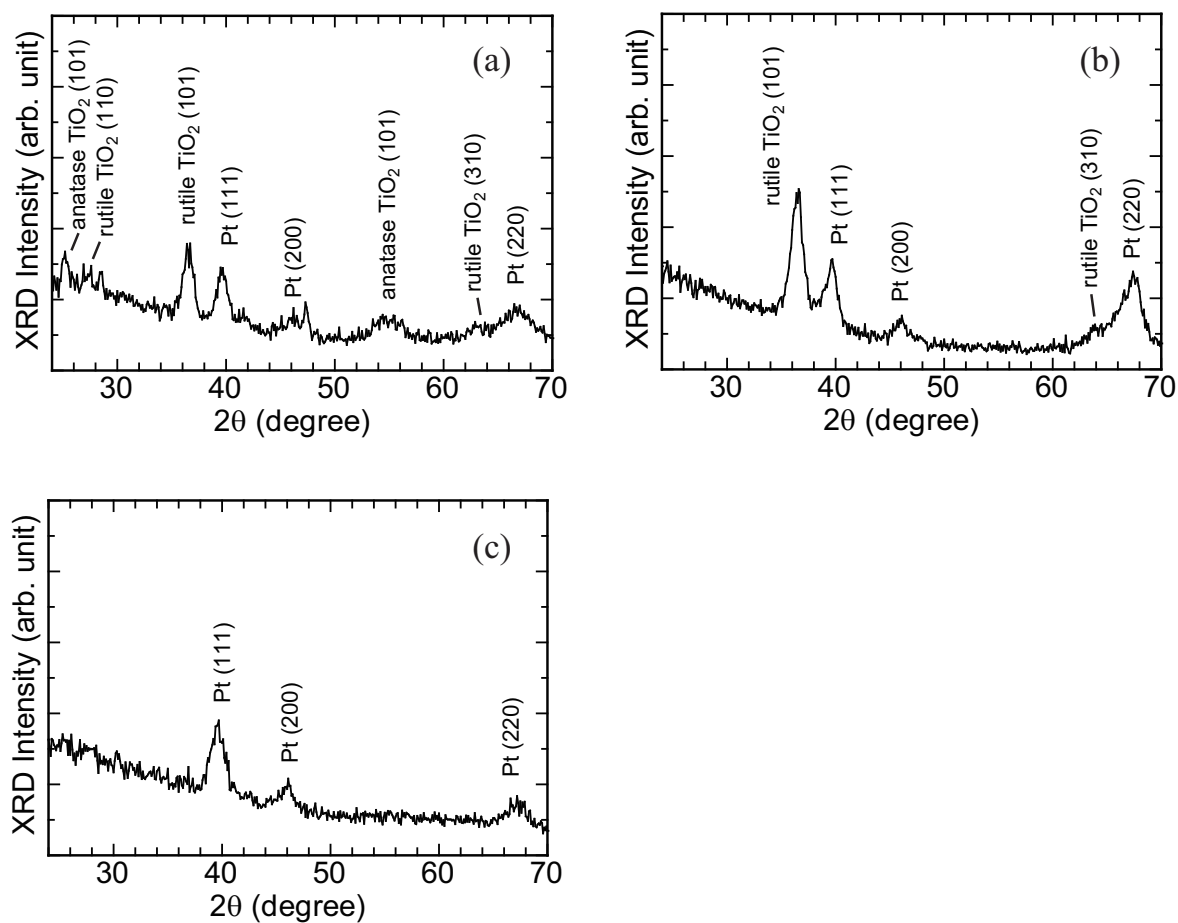
Figure 4.19: In-plane XRD curves of (a) the EB-Pt \text{TiO}_2 samples, (b) the SP-Pt \text{TiO}_2 samples, and (c) the thinner EB-Pt \text{TiO}_2 samples. The thickness of \text{TiO}_2 layers is approximately 40 nm.
