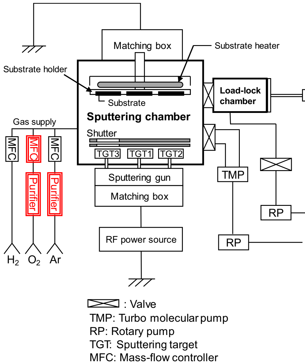
Figure 2.3: A schematic illustration of the sputtering system for NiO deposition.
