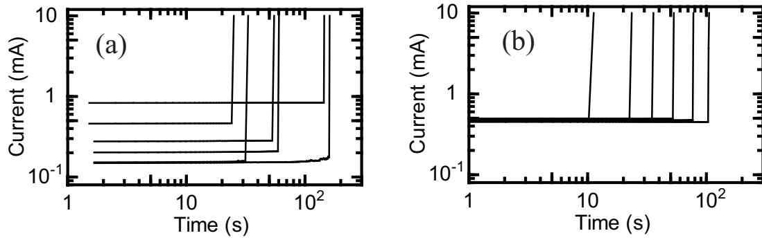
Figure 4.26: Representative current-time curves of (a) the EB-Pt NiO samples with a TE-diameter of 50\ \mu\text{m} and a NiO thickness of 50\ \text{nm} under V_S of 3.25\ \text{V} , and of (b) the SP-Pt NiO samples with a TE-diameter of 200\ \mu\text{m} and a NiO thickness of 80\ \text{nm} under V_S of 7.0\ \text{V} .
