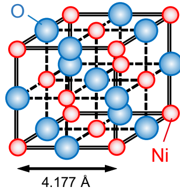
Figure 2.1: Crystalline structure of NiO.
