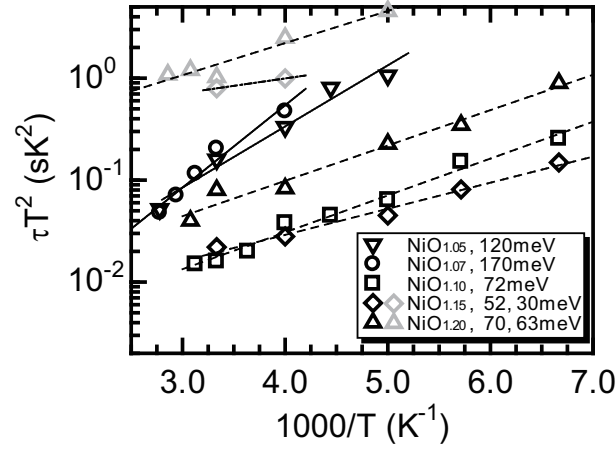
Figure 3.11: Arrhenius plots of \tau T^2 in various \text{NiO}_x/\text{n-Si} heterojunctions.
