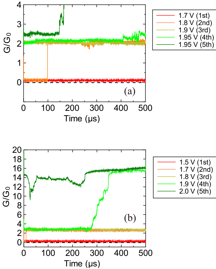
Figure 6.11: An example of changes of cell conductance in sample A by five times application of pulse voltage with a width of 500 \mu s . The RS cell size of (a) 625\pi \mu m^2 and (b) 2500\pi \mu m^2 .
