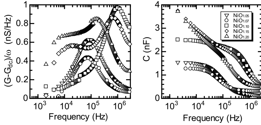
Figure 3.10: Frequency dependence of (G - G_{dc})/\omega and C for \text{NiO}_x/\text{n-Si} heterojunction at RT.
