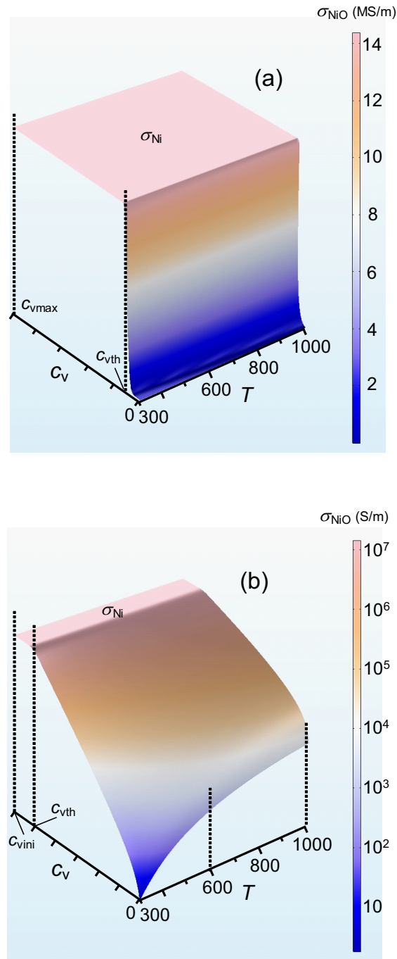
Figure B.1: Temperature and the concentration of \text{V}_{\text{O}} dependence of electrical conductivity of NiO in (a) linear and (b) log scale.
