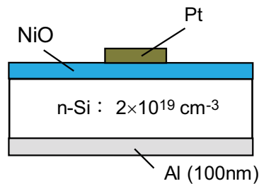
Figure 3.3: A Pt/ \text{NiO} / n -Si/ \text{Al} stack structure for admittance spectroscopy.
