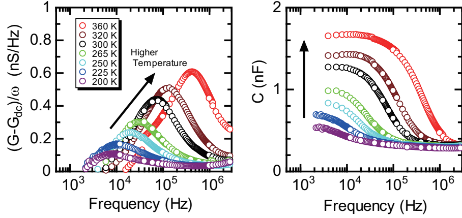
(b) p\text{-NiO}_{1.07}/n\text{-Si}
