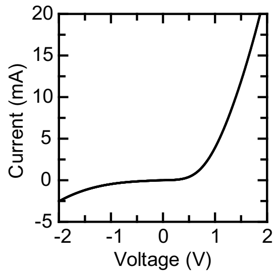
Figure 3.8: Current-voltage characteristics of \text{NiO}_{1.07}/n\text{-Si} heterojunction.
