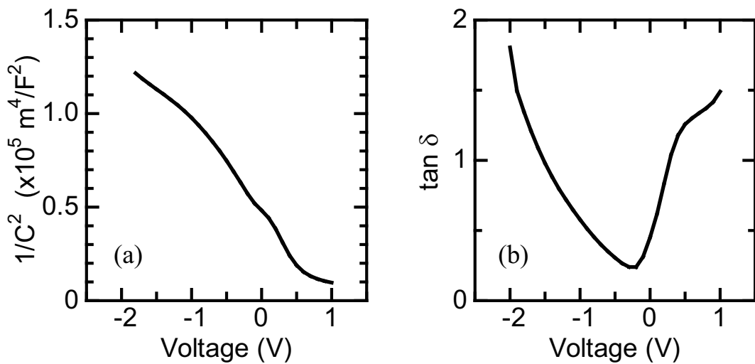
Figure 3.7: Voltage dependence of (a) 1/C^2 and (b) \tan \delta in NiO 1.07 / n -Si heterojunction.
