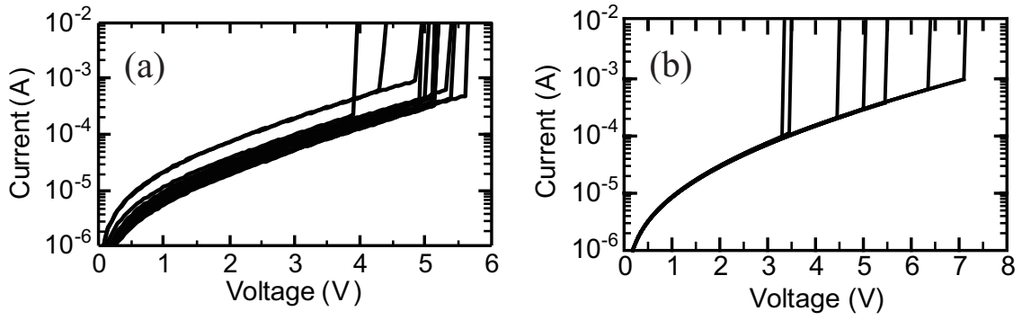
Figure 4.24: Typical current-voltage curves in (a) the EB-Pt NiO samples with a TE-diameter of 100\ \mu\text{m} and a NiO thickness of 50\ \text{nm} , and in (b) the SP-Pt NiO samples with a TE-diameter of 200\ \mu\text{m} and a NiO thickness of 60\ \text{nm} .
