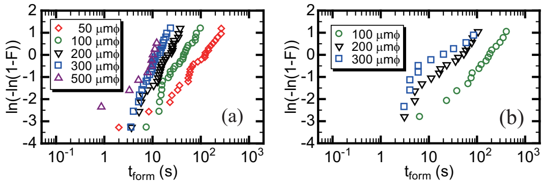
Figure 4.28: Individual Weibits of t_{\text{form}} for different cell sizes of (a) the EB-Pt NiO samples with a NiO thickness of 50\ \text{nm} under V_S of 3.25\ \text{V} , and of (b) the SP-Pt NiO samples with a NiO thickness of 80\ \text{nm} under V_S of 7.0\ \text{V} .
