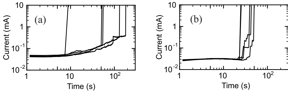
Figure 4.27: Representative current-time curves of (a) the EB-Pt \text{TiO}_2 samples under V_S of 4.2\ \text{V} , and of (b) the SP-Pt \text{TiO}_2 samples under V_S of 6.6\ \text{V} . A TE-diameter and \text{TiO}_2 thickness are 100\ \mu\text{m} and 35\ \text{nm} , respectively.
