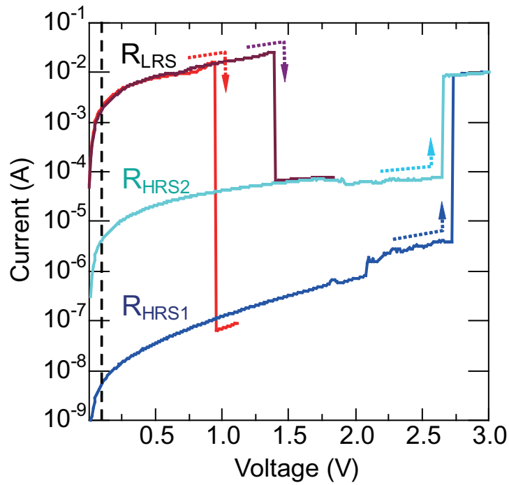
Figure 4.10: RS characteristics with two ranges of resistance in the high resistance state in the samples annealed at 400 ^{\circ}C during 30 min in Ar atmosphere.
