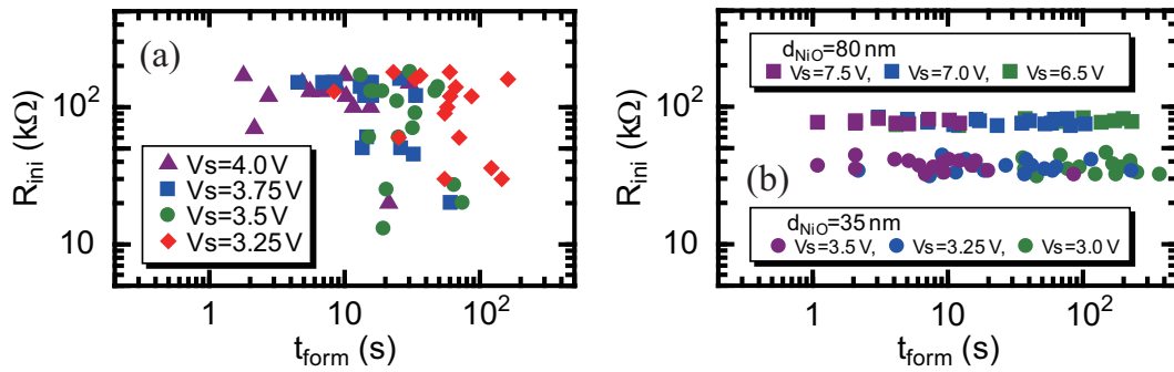
Figure 4.33: Distributions of R_{\text{ini}} vs t_{\text{form}} in (a) the EB-Pt NiO samples with a TE-diameter of 50 \mu\text{m} and a NiO thickness of 50 nm and in (b) the SP-Pt NiO samples with a TE-diameter of 200 \mu\text{m} and a NiO thickness of 35~80 nm.
