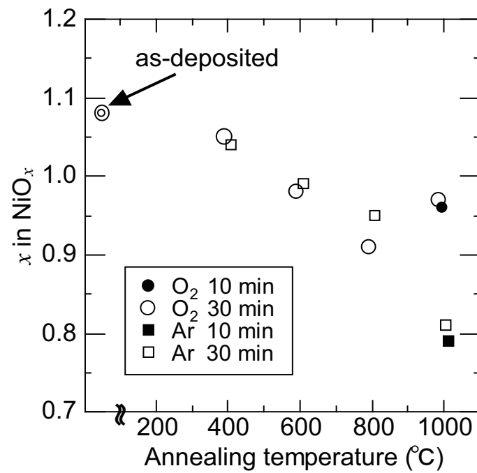
Figure 4.6: Annealing temperature dependence of oxygen composition in NiO layers estimated by SEM-EDX in \text{O}_2 and Ar atmosphere.
