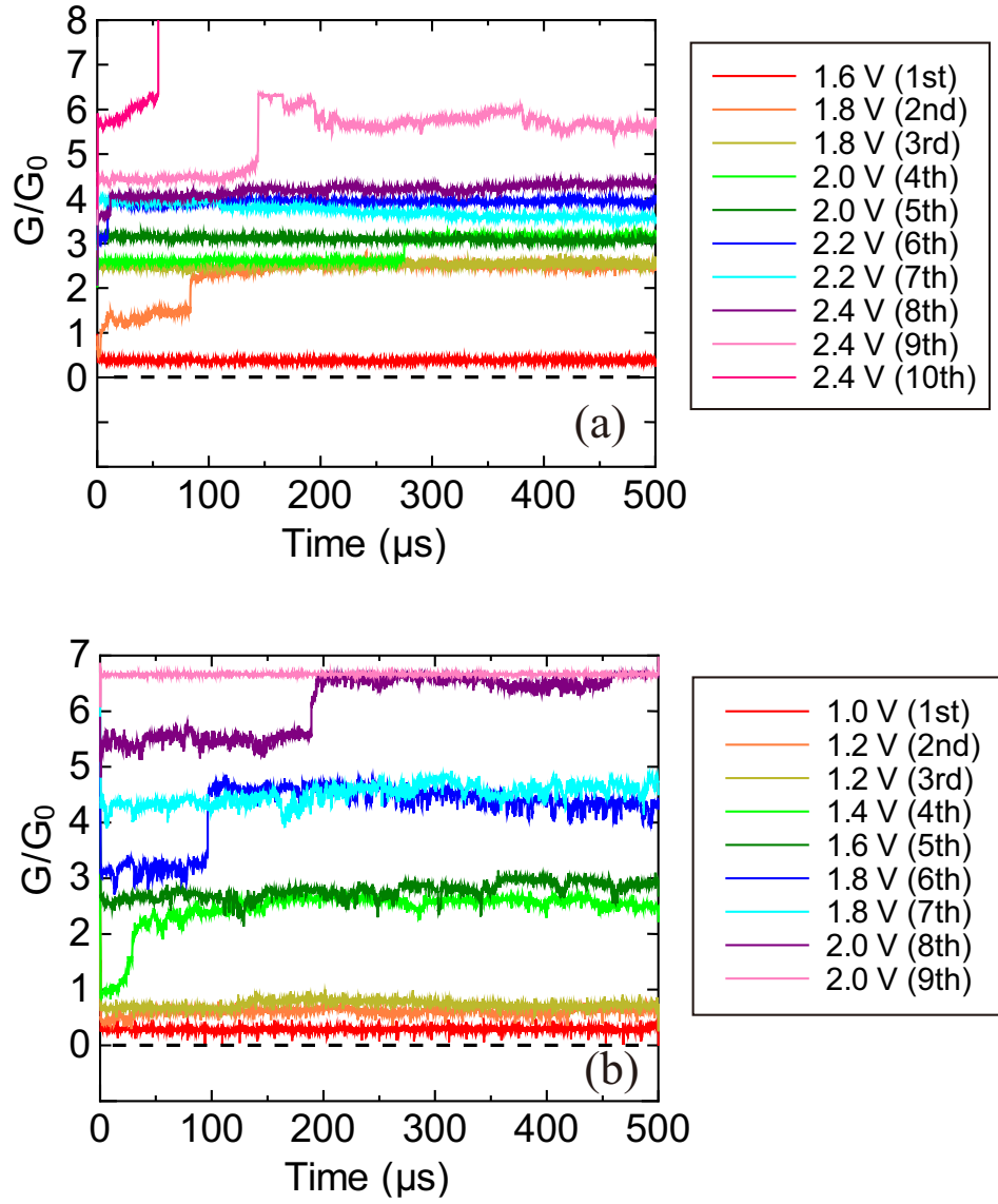
Figure 6.12: An example of changes of cell conductance in sample B by nine or ten times application of pulse voltage with a width of 500 \mu s . The RS cell size of (a) 625\pi \mu m^2 and (b) 2500\pi \mu m^2 .
