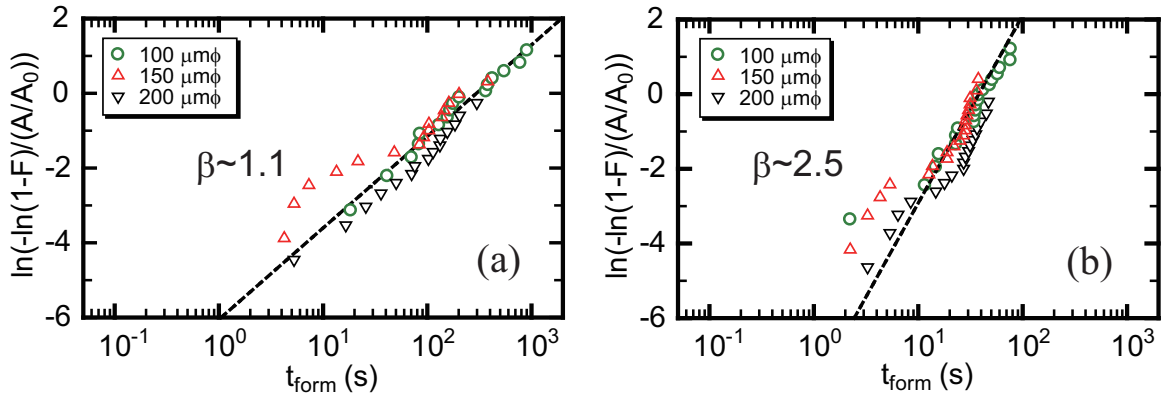
Figure 4.30: Individual Weibits of t_{\text{form}} normalized by cell sizes of (a) the EB-Pt \text{TiO}_2 samples with a \text{TiO}_2 thickness of 50 nm under V_S of 6.0 V and of (b) the SP-Pt \text{TiO}_2 samples with a \text{TiO}_2 thickness of 35 nm under V_S of 6.6 V at A_0 of \pi(100 \mu\text{m} / 2)^2 .
