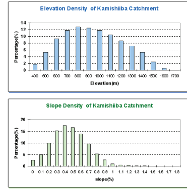
Fig. 4 Elevation and Slope Density graphs of Kamishiiba catchment.
