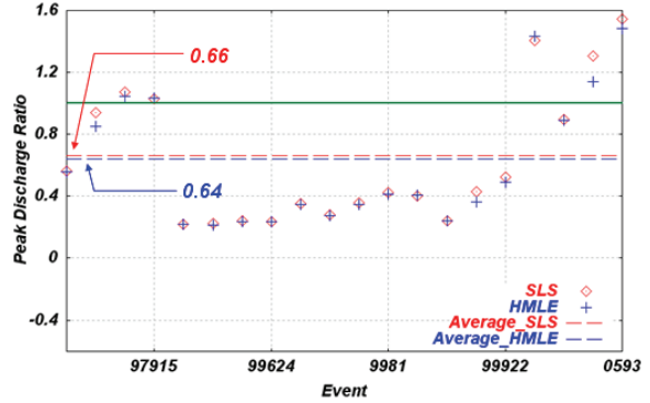
(b) KsEdgeFC2D
