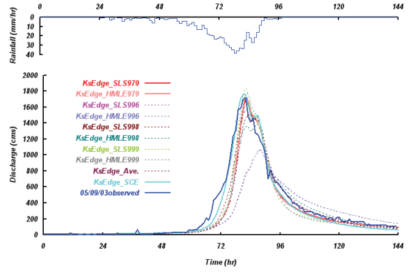
(b) KsEdgeFC2D
