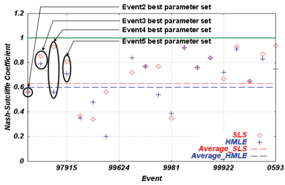
(a) SFM
