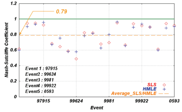
(b) KsEdgeFC2D
