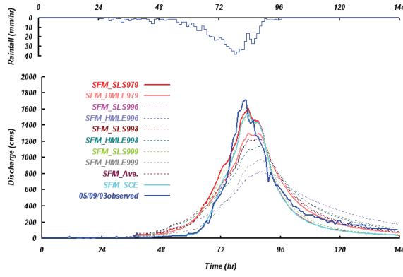
(a) SFM
