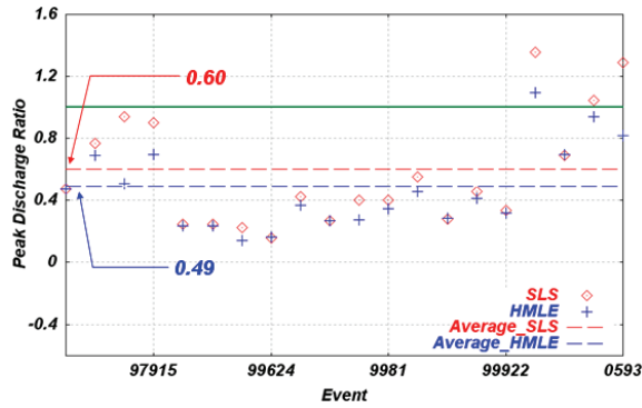
(a) SFM
