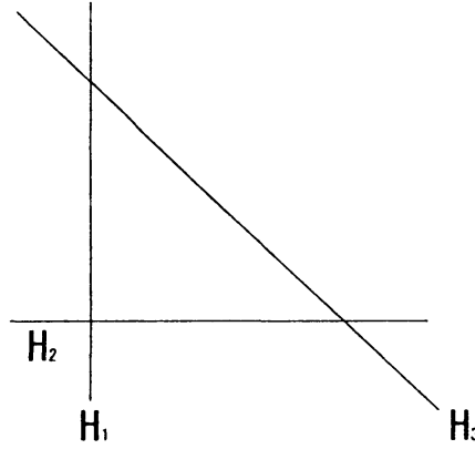
FIGURE 1. A hyperplane arrangement of T^*\mathbb{CP}(2)
