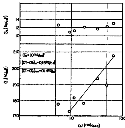
Fig. 11 Experimental relationships of G_1 - \omega and G_2 - \omega .
