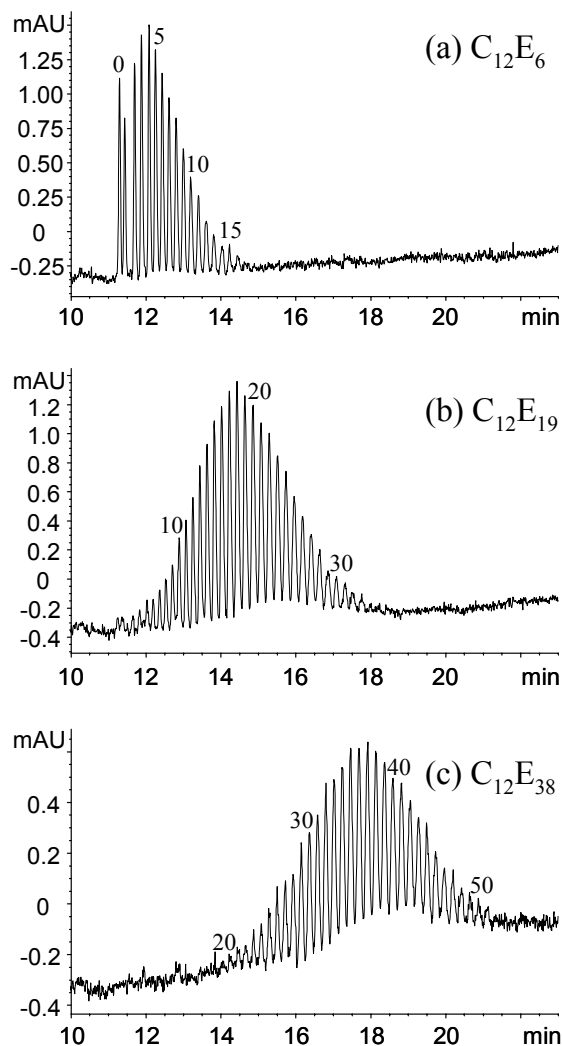
Figure 4-7. Optimal DTAC-MEKC separation of the FAE derivatives: (a) C_{12}E_6 , (b) C_{12}E_{19} , (c) C_{12}E_{38} . BGS, 30 mM DTAC in 10 mM phosphate buffer (pH 2.5) containing 20% (v/v) acetonitrile. Other conditions and peak identifications are as in Figure 4-6.
