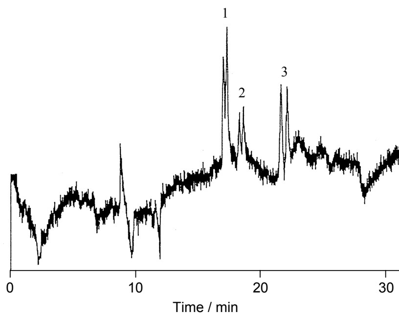
Figure 6-5. Chiral separation of three PTH–DL-amino acids by MEKC with digitonin. 1 = Nva; 2 = Val; 3 = Aba. Micellar solution, 50 mM digitonin–50 mM STDC–1 M urea (pH 2.5); capillary, 540 mm \times 50 \mu m I.D.; effective length, 340 mm; total applied voltage, 17.5 kV (324 V \text{cm}^{-1} ); current, 46 \mu A. Other conditions are as in Figure 6-2.
