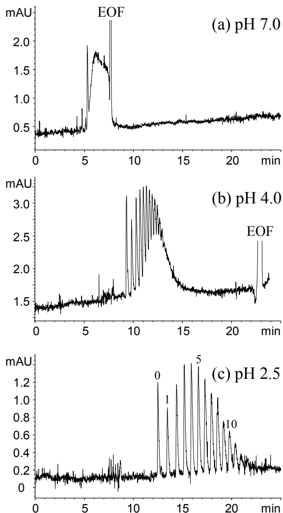
Figure 4-2. CZE separation of the C_{12}E_6 derivatives at pH (a) 7.0, (b) 4.0 and (c) 2.5. Capillary, 56.0 cm effective length, 64.5 cm total length, 50 \mu m I.D.; BGS, 20 mM phosphate buffer; applied voltage, +20 kV; injection, 1 s at 50 mbar; temperature, 25 ^{\circ} C; detection, 280 nm. The numbers above the peaks correspond to the number of the EO groups of the FAEs.
