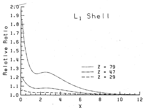
Fig. 16. The same as Fig. 15, but for L_1 shell.
