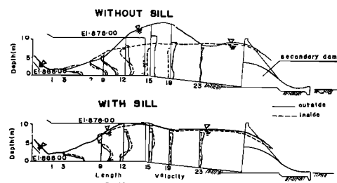
Fig. 6. Surface profile and velocity distribution in basin.
