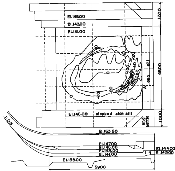
Fig. 13. Erosion pattern in apron for Tase Dam.
