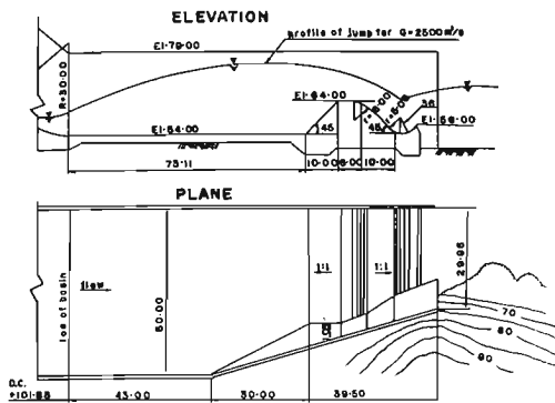
Fig. 8. Tsuruta Dam stilling basin works.
