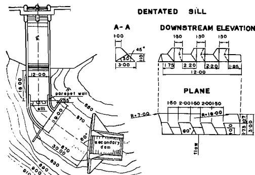
Fig. 5. Shinaki Dam spillway works and dentated sill.
