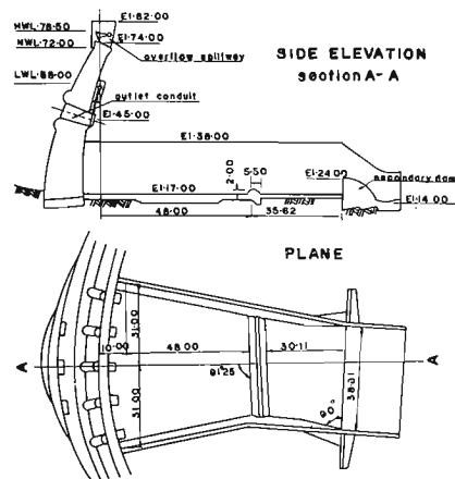
Fig. 10. Amagase Dam spillway works and stilling pool.
