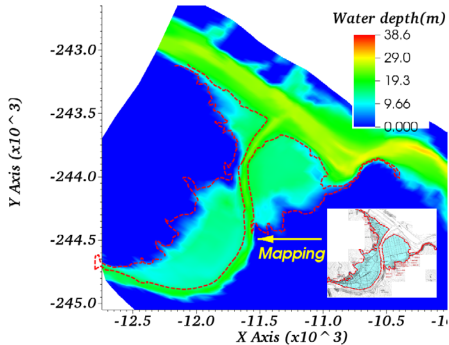
Figure 5-10 Comparison of an inundation area, which is the upper part of the study area(as shown in Fig. 2 by a blue line) and is marked by a red broken line to compare a simulated inundation area with an observed inundation area(bottom right).
