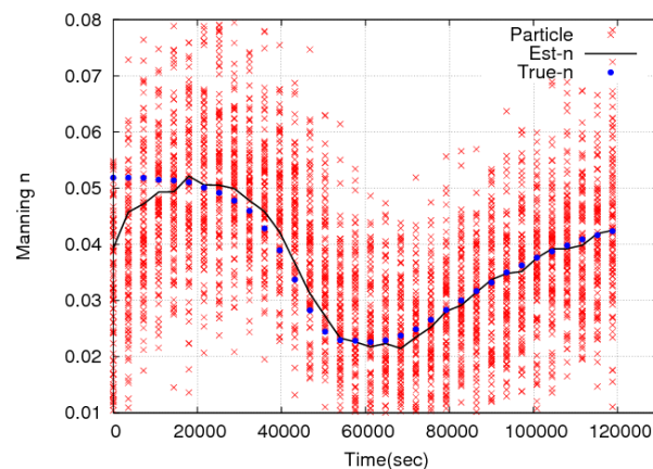
Figure 3-6 The comparison of Manning roughness coefficient in the synthetic experiment.
