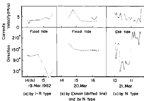
Fig. 10. Results of trials by the photoelectric current meters, I-R type and N type at the Oceanographic Tower Station of Kyoto University.
