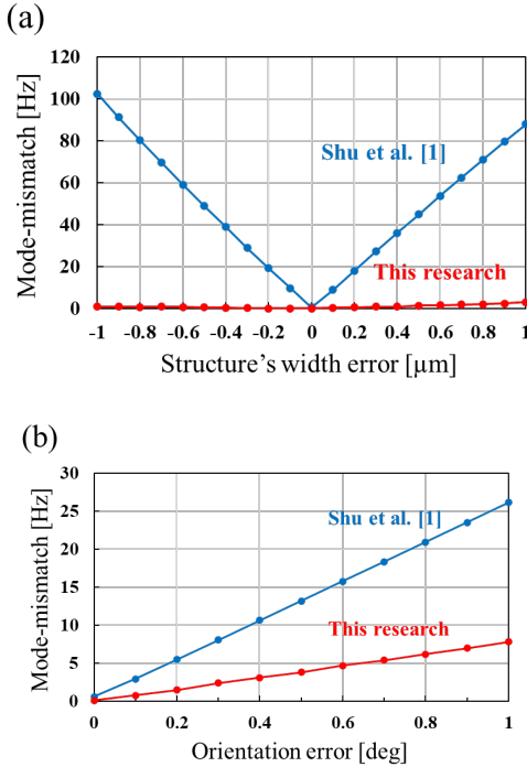
Fig. 4. Mode mismatch as a function of (a) structure's width error and (b) orientation error
