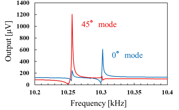
Fig. 8. Typical frequency response of ring resonator without any electrical tunings.
