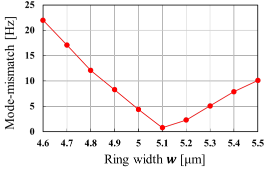
Fig. 3. Mode mismatch of designs shown in Fig.2 by adding fabrication errors of -0.8\text{ }\mu\text{m} .
