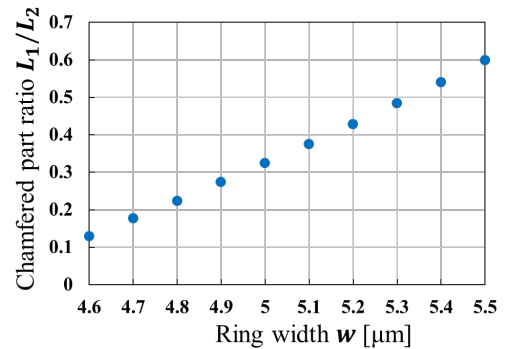
Fig. 2. Chamfered part ratio L_1/L_2 of mode-matched designs as a function of ring width w .
