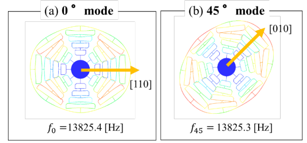
Fig. 5. Wineglass mode shapes of optimized resonator having smallest sensitivity to fabrication errors. The ring width is 5.1\text{ }\mu\text{m} and the chamfered part ratio L_1/L_2 is 0.375. (a) 0^\circ mode and (b) 45^\circ mode
