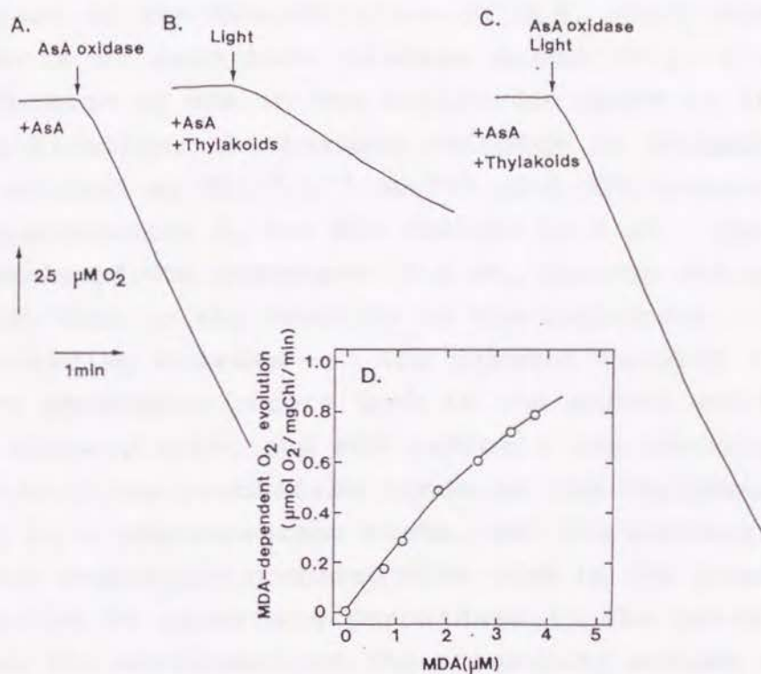
Fig. II-9 MDA radical-dependent oxygen evolution in illuminated thylakoids from spinach intact chloroplasts. (A) The reaction mixture (1 ml) contained the assay medium containing 1 mM ascorbate (AsA) and ascorbate oxidase (0.58 unit), and the oxygen uptake due to the oxidase activity was measured in the dark. (B) The reaction mixture (1 ml) contained the assay medium, thylakoid membranes (60 \mu\text{g} Chl) and 50 \mu\text{M} pCMB, and the photoreduction of dioxygen was measured under illumination at 320 \text{ W m}^{-2} . (C) The reaction mixture was the same as in (B), but the same amounts of ascorbate oxidase as in (A) was added. The oxygen uptake was measured under illumination at the same intensity as in (B). (D) The differences of \text{O}_2 uptake rates [(A) + (B) - (C)], corresponding to the MDA radical-dependent \text{O}_2 evolution, are plotted against the steady state concentrations of MDA radical, which were adjusted by the various amounts of ascorbate oxidase.
