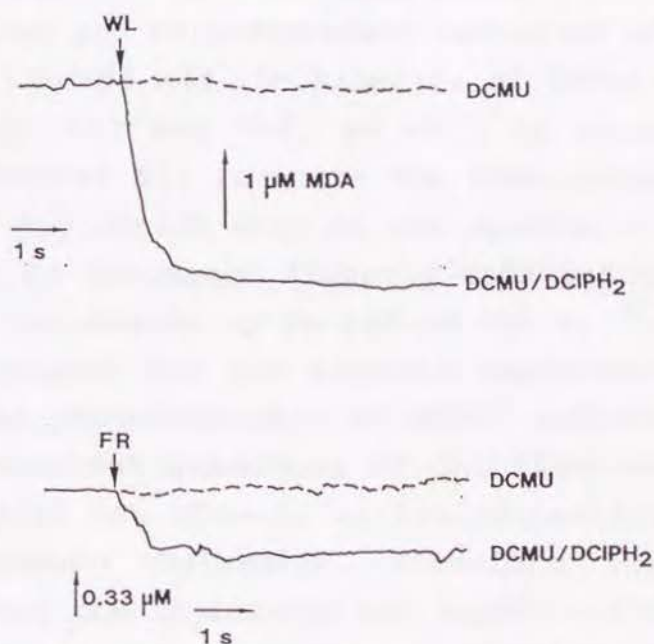
Fig. V-3 Reduced dichloroindophenol-dependent (DCIPH 2 -dependent) photoreduction of the MDA radical in spinach thylakoids in the presence of DCMU. The reaction mixture (70 \mu l) contained 50 mM HEPES-KOH, pH 7.6/0.4 M sucrose/2 mM MgCl 2 /0.1 \mu M nigericin/10 mM NaCl/2 mM ascorbate/sufficient ascorbate oxidase to generate 3.0 \mu M MDA radical/thylakoid membranes (0.7 \mu g Chl)/10 \mu M DCMU/5 \mu M Fd. Where indicated, 0.1 mM DCIP was added. In the presence of DCIP, the concentration of the MDA radical decreased to 2.4 \mu M as a result of the reduction of DCIP by ascorbate. Conditions for EPR were the same as described in Materials and Methods. The reaction mixture was illuminated by either white light (WL, 300 W m -2 ) or far-red light (FR, \geq 710 nm; 16 W m -2 ). After the light had been turned on, the decreases in the intensity of the EPR signal from the MDA radical at 338.6 mT were recorded.
