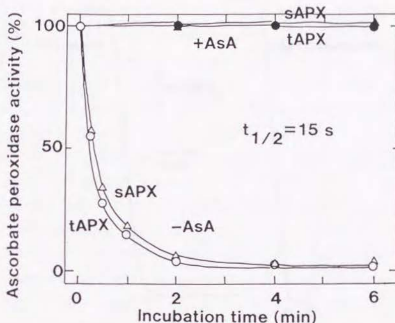
Fig. II-2 Inactivation of thylakoid-bound and stromal ascorbate (AsA) peroxidases from spinach chloroplasts in ascorbate-depleted medium. The thylakoids and stroma were separated from intact spinach chloroplasts as described in Materials and Methods. The thylakoid (5 \mu l, 1.1 \mu g Chl, tAPX, open circle) and the stroma (5 \mu l, sAPX, open triangle) fractions in the assay medium containing 1 mM ascorbate were diluted with 1 ml of 50 mM potassium phosphate, pH 7.0. At the indicated times after the dilution, 0.5 mM ascorbate was added, and the ascorbate peroxidase activity was assayed by the addition of 0.1 mM hydrogen peroxide. Where indicated (+AsA), the dilution was done with the buffer containing 0.5 mM ascorbate (tAPX, closed circle and sAPX, closed triangle).
