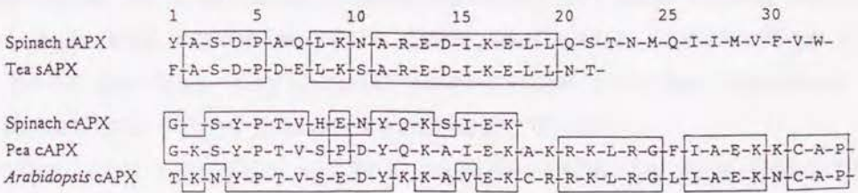
Fig. III-3 Amino acid sequences of the amino-terminal region of spinach tAPX (this study), tea sAPX (Chen et al. 1992), spinach cAPX (Tanaka et al. 1991), pea cAPX (Mittler and Zilinskas 1991b) and Arabidopsis cAPX (Kubo et al. 1992).
