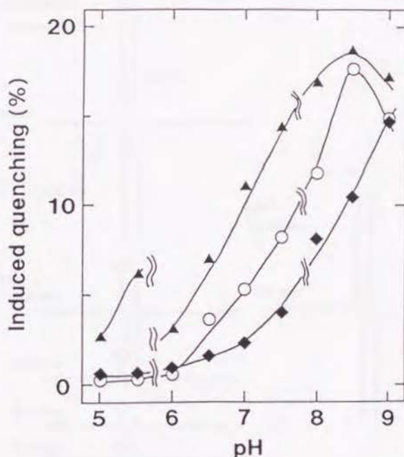
Fig. II-7 The effect of pH on MDA-dependent and hydrogen peroxide-dependent quenchings of chlorophyll fluorescence in the thylakoid membranes from spinach intact chloroplasts. The reaction mixture (1 ml) contained thylakoid membranes (60 \mu\text{g} Chl) and 0.1 \mu\text{M} nigericin in the buffers as in Fig. II-1. Hydrogen peroxide-dependent quenching (closed triangle) was determined after the addition of 100 \mu\text{M} hydrogen peroxide, as in Fig. II-5. MDA radical-dependent quenching (open circle) was determined by the addition of ascorbate oxidase (0.21 unit) which gave a steady state concentration of MDA of 1.2 \mu\text{M} , pH 7.0, as in Fig. II-6. Under the same conditions, the steady state concentration of MDA radical (closed diamond) was determined from the absorbance at 360 nm using an absorption coefficient of 3.3 \text{ mM}^{-1} \text{ cm}^{-1} . The hydrogen peroxide or MDA-dependent photochemical quenching is shown by the difference between the quenching before and after the addition of hydrogen peroxide or ascorbate oxidase. The maximum values of quenching after the addition were used.
