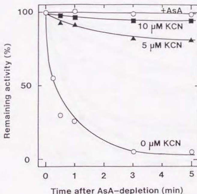
Fig. IV-3 Suppression of tAPX inactivation in ascorbate-depleted medium by potassium cyanide. tAPX (2 \mu\text{l} , 500 nM) containing 1 mM ascorbate (AsA) was diluted with 1 ml of 50 mM potassium phosphate, pH 7.0. At the indicated times after the dilution, 0.5 mM ascorbate was added to the diluted mixture to quench the inactivation, and the ascorbate peroxidase activity was assayed by the addition of 0.1 mM hydrogen peroxide as described in Materials and Methods. Where indicated, the dilutions were done with the buffer containing 0.5 mM ascorbate (AsA) and KCN at indicated concentrations. Activity of tAPX in the presence of ascorbate at 0 min was 0.04 unit and is taken as 100%. In the presences of 5 and 10 \mu\text{M} cyanide, activities of tAPX in the presence of ascorbate at 0 min was 60% and 24% of that in the absence of cyanide, respectively, and these activities are taken as 100%.
