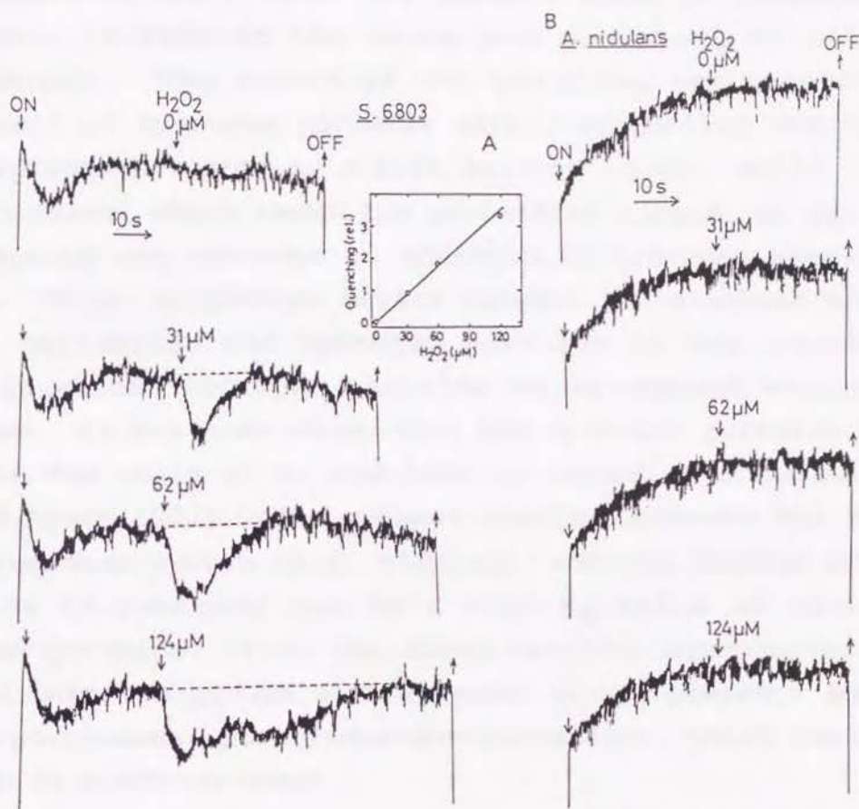
Fig. VI-6 The effect of hydrogen peroxide concentration on chlorophyll a fluorescence in the photoreductant peroxidase-containing S. 6803 (A) and the photoreductant peroxidase-lacking A. nidulans (B). The reaction mixture (0.8 ml) contained the cells (20 \mu\text{g} Chl a ) in the BG-11 medium. Hydrogen peroxide was added after the fluorescence reached F_m at the concentrations indicated. The relative quenching was determined from the area below the dotted lines after addition of hydrogen peroxide.
