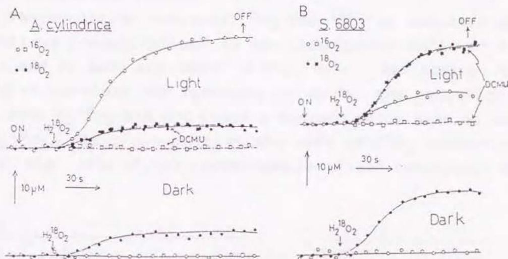
Fig. VI-3 Light-dependent decomposition of \text{H}_2^{18}\text{O}_2 and evolution of ^{16}\text{O}_2 and ^{18}\text{O}_2 in the photoreductant-peroxidase containing (A) A. cylindrica and (B) S. 6803 . The reaction mixture (1.0 ml) contained the cells ( A. cylindrica , 26 \mu\text{g} Chl a; S. 6803 , 29.0 \mu\text{g} Chl a), in 50 mM potassium phosphate, pH 7.0. \text{H}_2^{18}\text{O}_2 (80 \mu\text{M} ) was added 30 s after the light was turned on (400 \text{W m}^{-2} ) (ON). The dark controls were kept in the dark during the entire process. Where indicated, 10 \mu\text{M} DCMU (dotted lines, square and closed square) was added before the addition of \text{H}_2^{18}\text{O}_2 . With the disappearance of 80 \mu\text{M} \text{H}_2^{18}\text{O}_2 , 33 \mu\text{M} ^{16}\text{O}_2 ( A. cylindrica ) and 9.5 \mu\text{M} ^{16}\text{O}_2 ( S. 6803 ) were generated in the light. Thus, 83% ( A. cylindrica ) and 24% ( S. 6803 ) of the decomposition of hydrogen peroxide was accounted for by the peroxidase-catalyzed reaction linked to the photosynthetic electron transport. The amount of ^{18}\text{O}_2 evolved was 7 \mu\text{M} ( A. cylindrica ) and 22 \mu\text{M} ( S. 6803 ) in both the light and dark. Thus, 9% ( A. cylindrica ) and 55% ( S. 6803 ) of the hydrogen peroxide was decomposed by the catalase-catalyzed reaction. The remaining hydrogen peroxide would be reduced by a peroxidase using endogeneous reductants.
