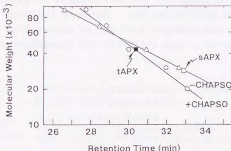
Fig. III-2 Determination of the molecular weight of purified tAPX from spinach thylakoids and APX in the stromal fraction of intact spinach chloroplasts by gel filtration on a column of TSK gel G3000SW XL . For the determination of molecular weight of tAPX, buffer B containing 1% (w/v) CHAPSO was used, and for that of sAPX, buffer B without CHAPSO was used. The molecular weight of each APX was determined from the retention time of the peak of activity of APX. The column was calibrated with the same molecular-weight standard proteins as indicated in the legend to Fig. III-1. [open circles (+CHAPSO) and triangles (-CHAPSO)].
