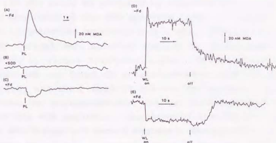
Fig. V-7 Flash-induced and continuous light-induced production of the MDA radical and its reduction by Fd in spinach thylakoids. The reaction mixture (70 \mu\text{l} ) contained 50 mM HEPES-KOH, pH 7.6/0.4 M sucrose/2 mM \text{MgCl}_2 /10 mM NaCl/0.1 \mu\text{M} nigericin/1 mM ascorbate/thylakoids (70 \mu\text{g Chl} ). Under the present conditions, 50 nM MDA radical was produced in darkness by the autooxidation of ascorbate. Where indicated, 30 \mu\text{M} CuZn-superoxide dismutase (SOD) or 5 \mu\text{M} Fd was added to the reaction mixture prior to the illumination by single-turnover pulse light (PL, 1,500 \text{ W m}^{-2} ; 14 \mu\text{s} ) or white light (WL, 300 \text{ W m}^{-2} ). The inhibition of EPR signals from the MDA radical at 338.6 mT were monitored. Conditions for EPR were the same as described in Materials and Methods, with the exception that the receiver gain was 1 \times 1,000 .
