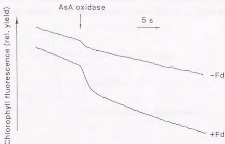
Fig. V-2 Effects of Fd on the photochemical quenching of Chl fluorescence in thylakoid membranes induced by the MDA radical. Fluorescence yield was monitored with a weak, modulated measuring light, and the relative yield of Chl fluorescence was induced by saturating actinic white light ( 300 \text{ W m}^{-2} ). The reaction mixture (1 ml) contained 50 mM HEPES-KOH, pH 7.6/0.4 M sucrose/2 mM \text{MgCl}_2 /0.1 \mu\text{M} nigericin/10 mM NaCl/1 mM ascorbate/thylakoid membranes (20 \mu\text{g} Chl) and 5 \mu\text{M} Fd as indicated. Sufficient ascorbate (AsA) oxidase was added 15 s after the start of illumination by actinic light to give a steady-state concentration of the MDA radical of 2.6 \mu\text{M} in darkness.
