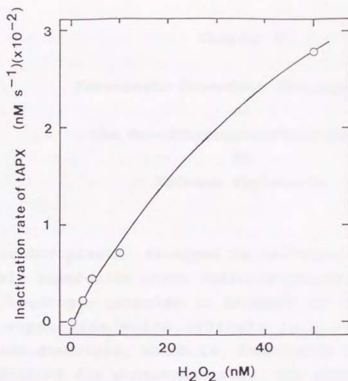
Fig. IV-6 Effect of hydrogen peroxide concentration on inactivation rate of tAPX under anaerobic conditions. Inactivation rate of tAPX was calculated from Fig. IV-4 as described in text and is plotted against the concentrations of hydrogen peroxide.
