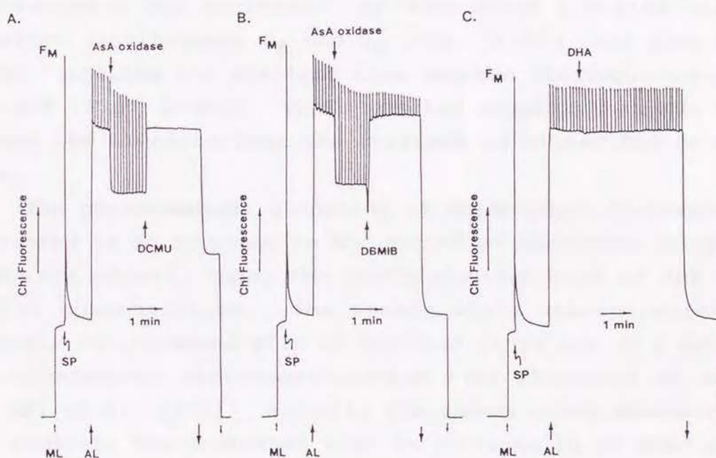
Fig. II-6 Quenching of chlorophyll fluorescence by MDA radical in thylakoid membranes. Fluorescence was measured as in Fig. II-5. The reaction mixture (1 ml) contained thylakoid membranes (60 \mu\text{g} Chl) in the assay medium, in which the concentration of ascorbate was 0.5 mM. Ascorbate oxidase (0.35 unit, A and B) which gave a steady state concentration of MDA radical of 2.1 \mu\text{M} or 2 mM DHA (C) was added 60 s after the actinic light was turned on. DCMU (10 \mu\text{M} , A) and DBMIB (0.5 \mu\text{M} , B) were added at a time, where indicated.
