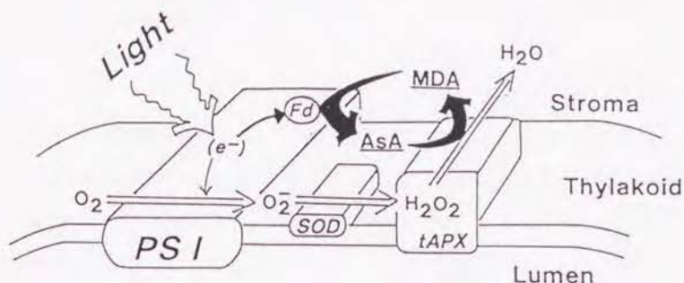
Fig. V-10 The proposed thylakoid scavenging system for superoxide radicals and hydrogen peroxide in chloroplasts. For details, see the text.
