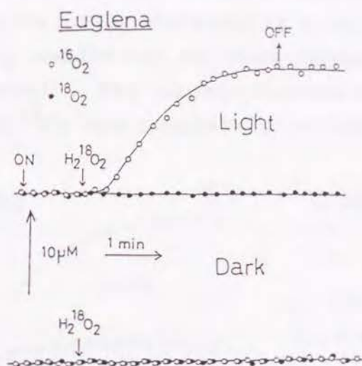
Fig. VI-2 Light-dependent decomposition of \text{H}_2^{18}\text{O}_2 and evolution of ^{16}\text{O}_2 and ^{18}\text{O}_2 in the cells of Euglena gracilis . The reaction mixture (0.5 ml) contained the cells (23.7 \mu\text{g} Chl) in 50 mM HEPES-KOH, pH 7.0. \text{H}_2^{18}\text{O}_2 (69 \mu\text{M} ) was added 1 min after the light was turned on (400 \text{W m}^{-2} ) (ON), and no \text{H}_2^{18}\text{O}_2 was found after the reaction. The dark control was kept in the dark during the entire process, and 13 \mu\text{M} \text{H}_2^{18}\text{O}_2 was decomposed during the dark reaction.
