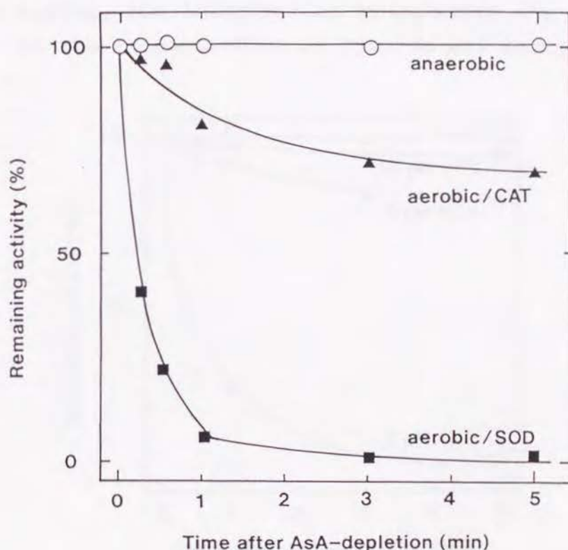
Fig. IV-2 Effects of dioxygen, catalase and superoxide dismutase on tAPX inactivation in ascorbate-depleted medium. tAPX (2 \mu\text{l} , 500 nM) containing 1 mM ascorbate (AsA) was diluted with 1 ml of 50 mM potassium phosphate, pH 7.0. At the indicated times after the dilution, 0.5 mM ascorbate was added to the diluted mixture to quench the inactivation, and the ascorbate peroxidase activity was assayed as described in Materials and Methods. Where indicated, the dilutions were done with the following buffers: aerobic/SOD, the buffer was equilibrated with air and contained CuZn-superoxide dismutase (200 units); aerobic/CAT, the buffer was equilibrated with air and contained catalase (1,000 units); anaerobic, the buffer was deaerated with argon gas and the dilution was done under anaerobic conditions. Activity of tAPX in the presence of ascorbate at 0 min was 0.04 unit and is taken as 100%.
