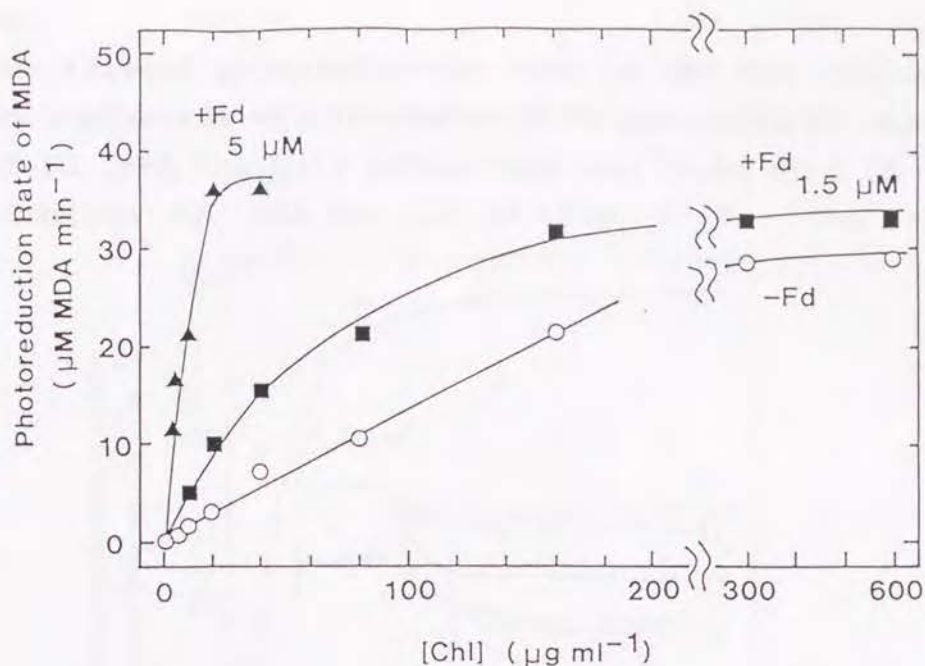
Fig. V-4 Effects of the concentration of thylakoids on the rate of photoreduction of the MDA radical in the presence of Fd. The reaction mixture (70 \mu l) contained 50 mM HEPES-KOH, pH 7.6/0.4 M sucrose/2 mM \text{MgCl}_2 /0.1 \mu M nigericin/10 mM NaCl/2 mM ascorbate/sufficient ascorbate oxidase to generate 3.1 \mu M MDA radical. Thylakoid membranes and Fd were added to the reaction mixture at indicated concentrations. After white light (300 \text{W m}^{-2} ) had been turned on, the rate of photoreduction of the MDA radical was determined from the initial rate of decrease in the intensity of the EPR signal from the MDA radical at 338.6 mT.
