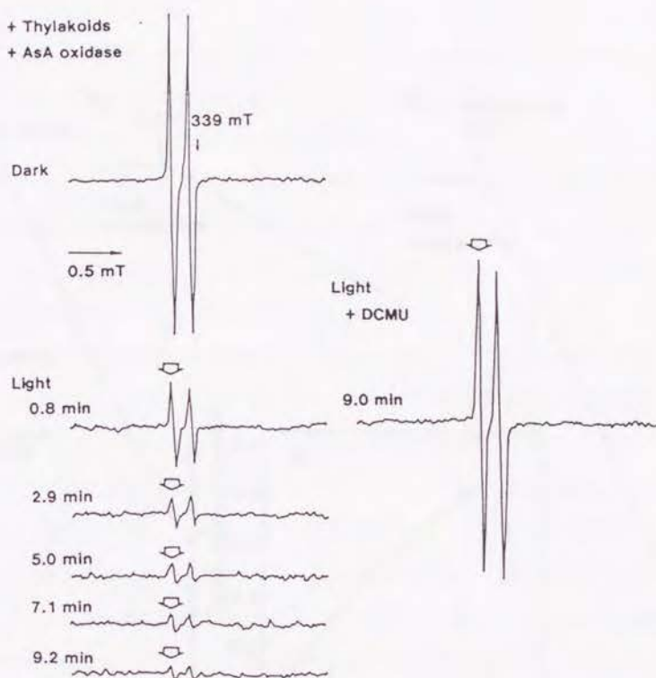
Fig. II-8 Photoreduction of MDA radical generated by ascorbate oxidase in thylakoids as measured by EPR spectrum. The reaction mixture (1.0 ml) contained the 1 mM ascorbate-containing assay medium, thylakoid membranes (60 \mu g Chl) and ascorbate oxidase (1.27 unit) which produced 4 \mu M MDA radical. Where indicated, 10 \mu M DCMU was added before the light was turned on. More than 80% of MDA signal was kept for 20 min in the dark. EPR conditions were set as follows: Microwave power, 3 mW; Sweep time, 2 min; Receiver gain, 1.6 \times 100 ; Time constant, 0.3 s; Modulation amplitude, 0.032 mT. Time shown at the left side of EPR signals is the time when EPR signal with open arrow was recorded after the light was turned on.
