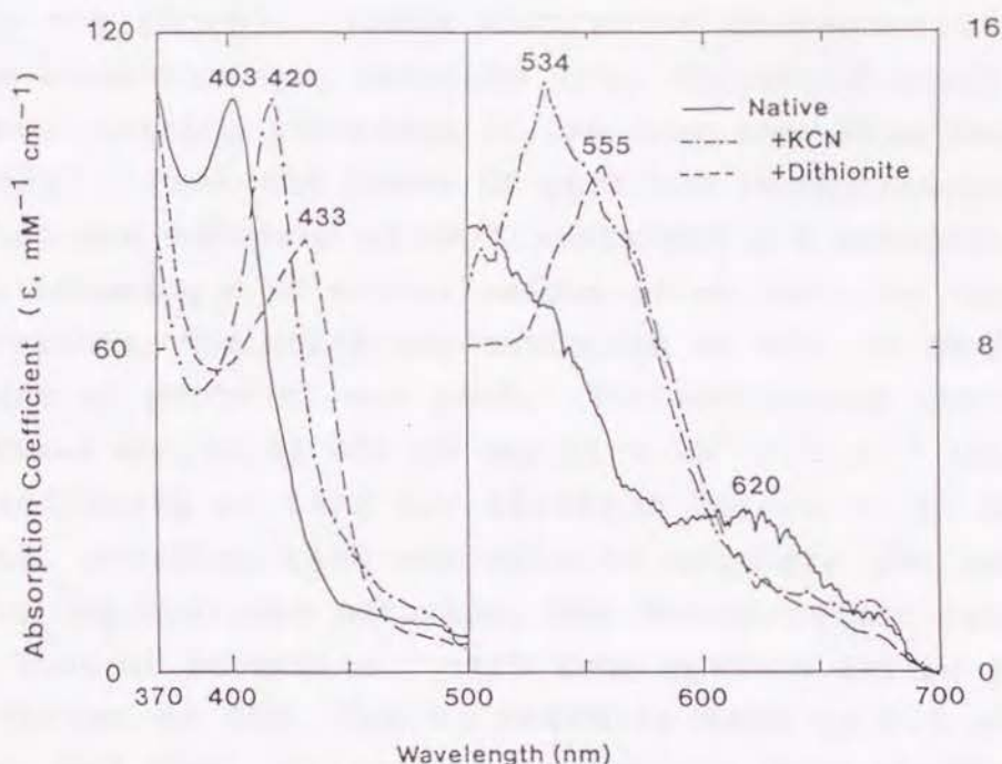
Fig. III-4 Absorption spectra of purified tAPX from spinach thylakoids. The absorption spectra of tAPX were recorded from a 1.3 \mu\text{M} solution in 50 mM potassium phosphate (pH 7.5)/0.1 mM EDTA/1 mM PMSF/5 mM ascorbate/0.1 M KCl/1% CHAPSO. Native form (—), no additions; reduced form (---), dithionite was added; CN-form (---), 1 mM KCN was added.
