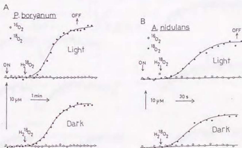
Fig. VI-5 Decomposition of \text{H}_2^{18}\text{O}_2 in the cells of the photoreductant peroxidase-lacking (A) P. boryanum and (B) A. nidulans . To the reaction mixture ( P. boryanum , 29.2 \mu\text{g} Chl a in 0.5 ml of 50 mM HEPES-KOH, pH 7.0; A. nidulans , 25 \mu\text{g} Chl a in 1 ml of 50 mM potassium phosphate, pH 7.0), \text{H}_2^{18}\text{O}_2 ( P. boryanum , 36 \mu\text{M} ; A. nidulans , 80 \mu\text{M} ) was added at indicated times after the light was turned on ( 400 \text{ W m}^{-2} ) (ON). During the light incubation, 22 \mu\text{M} \text{H}_2^{18}\text{O}_2 ( P. boryanum ) and 32 \mu\text{M} \text{H}_2^{18}\text{O}_2 ( A. nidulans ) were decomposed. Dark control was kept in the dark during the entire process. During the dark incubation, 18 \mu\text{M} \text{H}_2^{18}\text{O}_2 ( P. boryanum ) and 34 \mu\text{M} \text{H}_2^{18}\text{O}_2 ( A. nidulans ) were decomposed.
