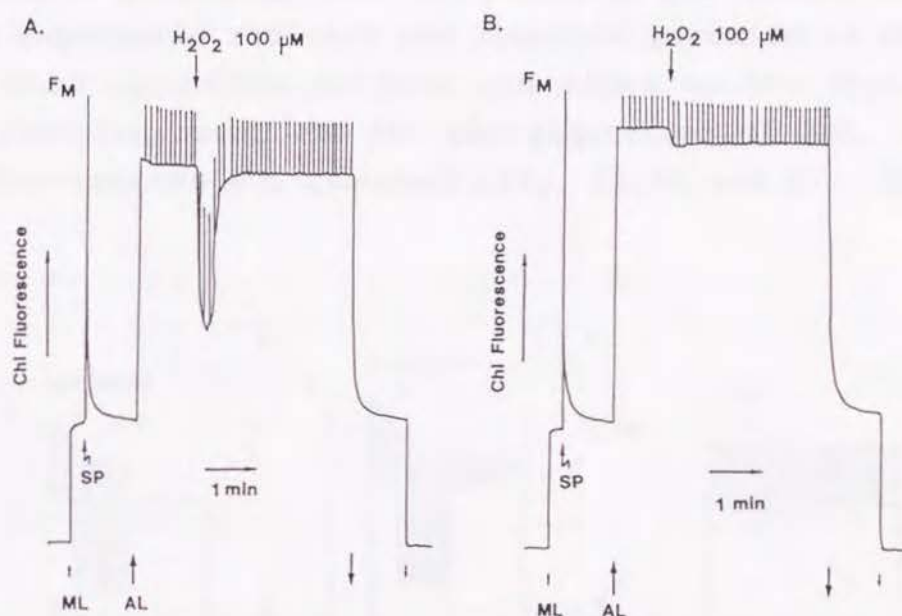
Fig. II-5 Effect of hydrogen peroxide on chlorophyll fluorescence in thylakoid membranes. Fluorescence yield was monitored with a weak, modulated measuring light (ML) and the maximum yield ( F_M ) was induced by 500-ms pulses of saturating white light (SP). Illumination of continuous actinic light (AL, red light) was started by the AL arrow. (A) The reaction mixture (1.0 ml) contained thylakoid membranes (60 \mu g Chl), 0.1 \mu M nigericin in the assay medium containing 1 mM ascorbate. Hydrogen peroxide (100 \mu M) was added 60 s after the actinic light was turned on. (B) The reaction mixture was the same as in (A), but thylakoid membranes had been treated with the ascorbate-depleted assay medium as in Fig. II-3.
