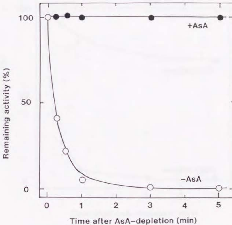
Fig. IV-1 Inactivation of tAPX purified from spinach thylakoids in ascorbate-depleted medium. tAPX (2 \mu l, 500 nM) containing 1 mM ascorbate (AsA) was diluted with 1 ml of 50 mM potassium phosphate, pH 7.0. At the indicated times after the dilution, 0.5 mM ascorbate was added to the diluted mixture to quench the inactivation, and the ascorbate peroxidase activity was assayed by the addition of 0.1 mM hydrogen peroxide as described in Materials and Methods. Where indicated (+AsA), the dilution was done with the buffer containing 0.5 mM ascorbate. Activity of tAPX in the presence of ascorbate at 0 min was 0.04 unit and is taken as 100%.
