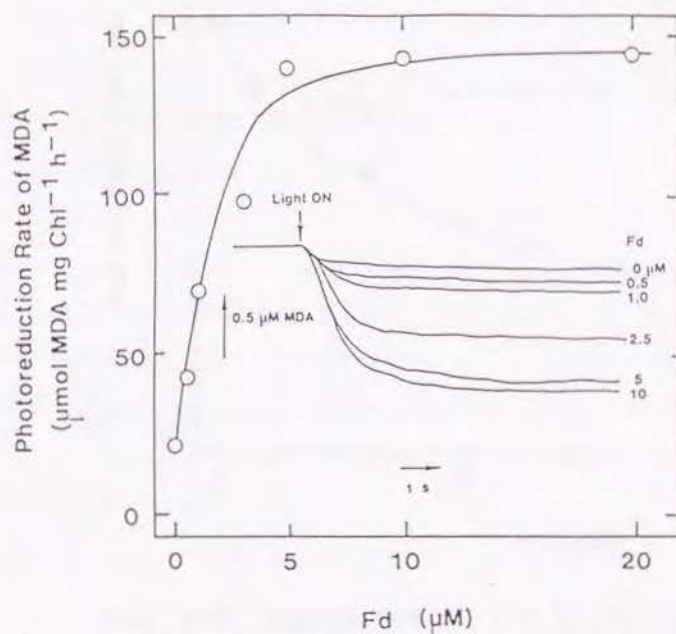
Fig. V-5 Dependence of the photoreduction of the MDA radical on the concentration of Fd in spinach thylakoids. The reaction mixture (70 \mu\text{l} ) contained 50 mM HEPES-KOH, pH 7.6/0.4 M sucrose/2 mM \text{MgCl}_2 /0.1 \mu\text{M} nigericin/10 mM NaCl/2 mM ascorbate/sufficient ascorbate oxidase to generate 1.1 \mu\text{M} MDA radical/thylakoid membranes (0.7 \mu\text{g} Chl). Fd was added at indicated concentrations. Conditions for EPR are described in Materials and Methods. After white light (300 \text{W m}^{-2} ) had been turned on, the photoreduction rate of the MDA radical was determined from the initial rate of decrease in the intensity of the EPR signal from the MDA radical at 338.6 mT. Inserts show the time course of the reduction of MDA radicals.
