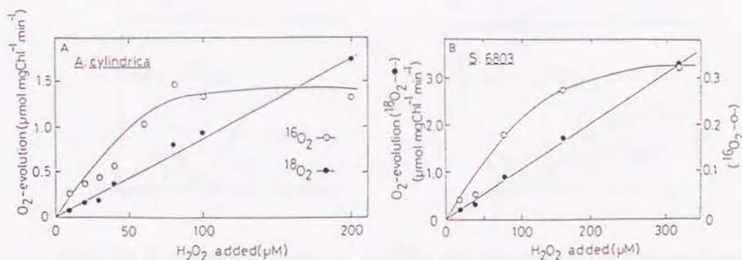
Fig. VI-4 Effect of \text{H}_2^{18}\text{O}_2 concentration on ^{16}\text{O}_2 and ^{18}\text{O}_2 evolution in illuminated cells of (A) A. cylindrica and (B) S. 6803 . The reaction mixture (1.0 ml) contained the cells (25 \mu\text{g} Chl a) in 50 mM potassium phosphate, pH 7.0, and \text{H}_2^{18}\text{O}_2 was added at the indicated concentrations. The other conditions were the same as in the legend to Fig. VI-3, and the maximum evolution rates of ^{16}\text{O}_2 and ^{18}\text{O}_2 were determined.
