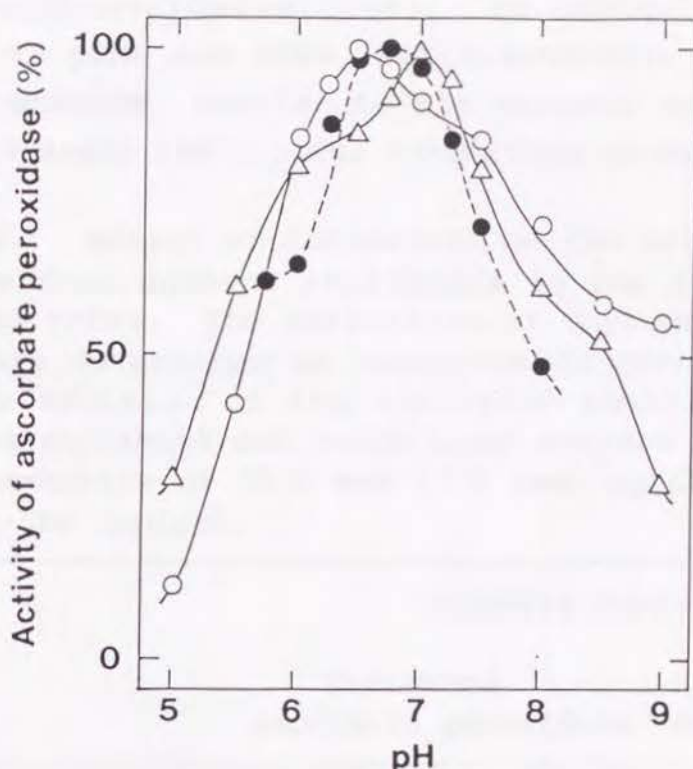
Fig. II-1 The effect of pH on the activities of ascorbate peroxidase from spinach chloroplasts in the thylakoid-bound form, solubilized form from the thylakoids and the stroma. The reaction mixture (1 ml) contained 0.33 M sorbitol, 10 mM NaCl, 1 mM \text{MgCl}_2 , 2 mM EDTA, 0.5 mM \text{KH}_2\text{PO}_4 , 0.5 mM ascorbate, the enzyme and the following buffers; pH 5.0-5.5, 50 mM MES-KOH; pH 6.0-7.5, 50 mM potassium phosphate; pH 8.0-9.0, 50 mM Tricin-KOH. The enzyme activities were assayed by the addition of 0.1 mM hydrogen peroxide as described in Materials and Methods. The enzyme used was the thylakoid fraction (open circle), 1.5% octyl-glucoside solubilized enzyme (closed circle) or the stroma fraction (triangle) which gave the oxidation rate of ascorbate of 9.7, 9.1 or 7.3 \mu\text{mol mg Chl}^{-1} \text{min}^{-1} , respectively, at pH 7.0.
