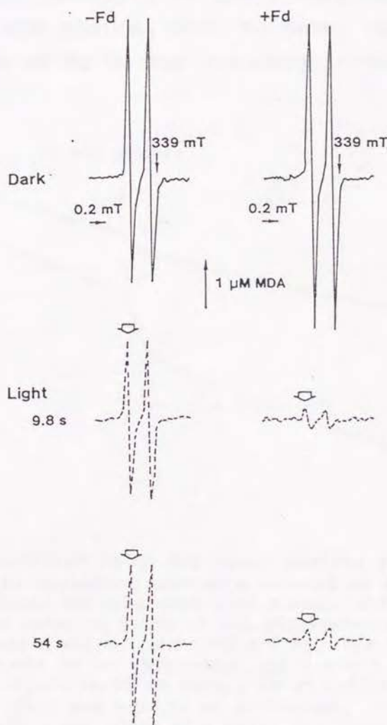
Fig. V-1 Fd-dependent photoreduction of the MDA radical generated by ascorbate oxidase in spinach thylakoids, as monitored by EPR. The reaction mixture (70 \mu l) contained 50 mM HEPES-KOH, pH 7.6/0.4 M sucrose/2 mM \text{MgCl}_2 /10 mM NaCl/0.1 \mu M nigericin/2 mM ascorbate/sufficient ascorbate oxidase to generate 3.0 \mu M MDA radical/thylakoid membranes (0.7 \mu g Chl). Where indicated, 5 \mu M Fd was added. Conditions for EPR were the same as described in Materials and Methods, with the exception that the sweep time was 43 s for each scan. Indicated times show the time of the recording of the EPR signal at 338.6 mT (open arrow) after the white light had been turned on ( 300 \text{ W m}^{-2} ).
