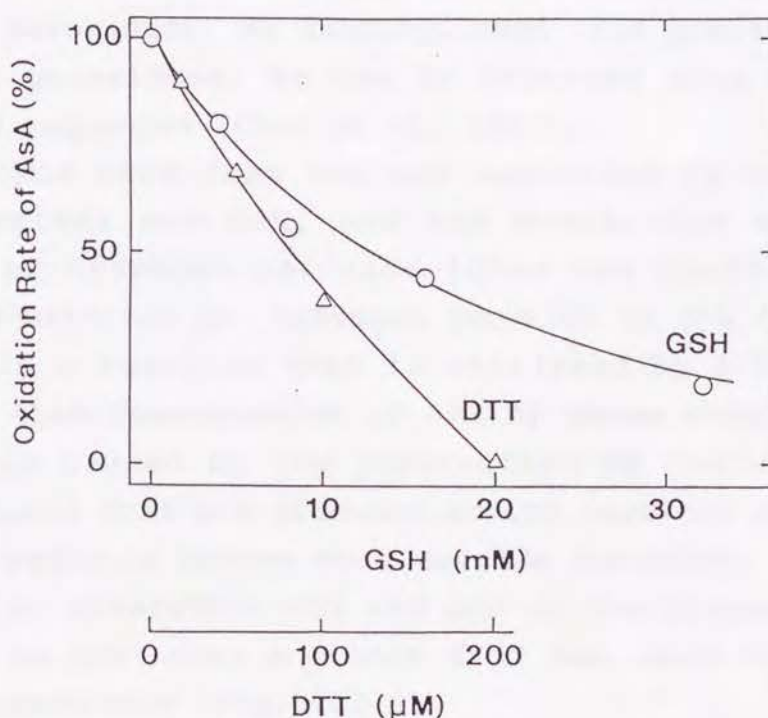
Fig. III-6 Inhibition of tAPX from spinach thylakoids by thiols, as determined from the rate of oxidation of ascorbate. The reaction mixture contained 50 mM potassium phosphate (pH 7.0)/0.5 mM ascorbate/tAPX (0.04 unit)/0.1 mM hydrogen peroxide/dithiothreitol (DTT) (triangles) or GSH (circles) at the indicated concentrations. The initial rate of oxidation of AsA was determined from the decrease in the absorbance at 290 nm which was recorded for 5 s from 1.5 s after the start of the reaction by the addition of hydrogen peroxide. The rate in the absence of thiols is taken as 100%.
