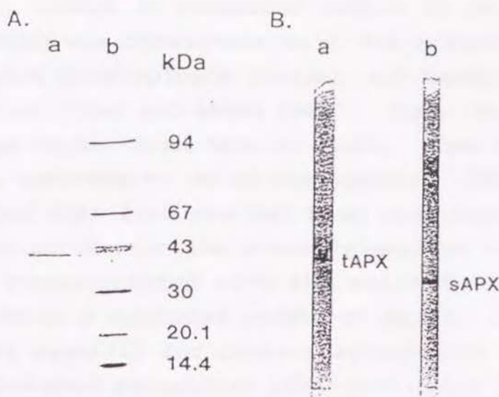
Fig. III-1 (A) SDS-Polyacrylamide gel electrophoresis of the purified tAPX from spinach. Lane a, purified tAPX (4 \mu g). Lane b, molecular-mass standard proteins (kDa, 30 \mu g total): phosphorylase b (94), bovine serum albumin (67), ovalbumin (43), carbonic anhydrase (30), trypsin inhibitor (20.1), \alpha -lactoalbumin (14.4). (B) Immunoblotting of purified tAPX from spinach and purified sAPX from tea (Chen and Asada 1989) with the antibody against the tea sAPX after SDS-PAGE. Lane a, spinach tAPX (4 \mu g). Lane b, tea sAPX (4 \mu g).
