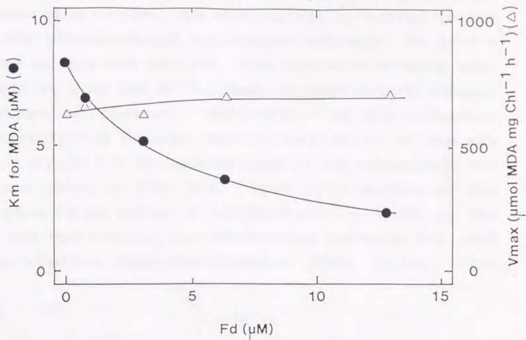
Fig. V-6 Dependence of the K_m for the MDA radical and the V_{max} of its photoreduction by spinach thylakoids on the concentration of Fd. The reaction mixture (70 \mu l) contained 50 mM HEPES-KOH, pH 7.6/0.4 M sucrose/2 mM MgCl_2 /0.1 \mu M nigericin/10 mM NaCl/2 mM ascorbate/thylakoid membranes (0.7 \mu g Chl)/Fd at indicated concentrations. Ascorbate oxidase was added to the reaction mixture to generate the indicated concentrations of the MDA radical up to 3 \mu M. The initial photoreduction rate of the MDA radical was measured as described in the legend to Fig. V-4. Apparent K_m values for the MDA radical (closed circles) and V_{max} for its photoreduction (open triangles) at several concentrations of Fd were determined from the non-linear regression analysis of the photoreduction rates using Michaelis and Menten's equation (Sakota and Hiromi 1976).
