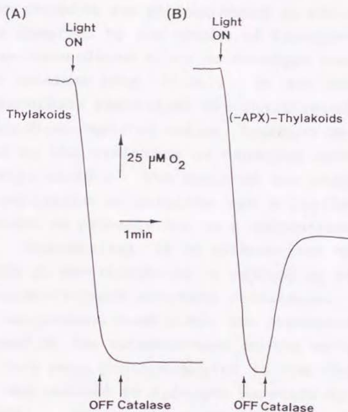
Fig. II-3 Reduction of the hydrogen peroxide generated in illuminated thylakoids by ascorbate catalyzed with the thylakoid-bound ascorbate peroxidase (APX). In trace (A), the reaction mixture (1 ml) contained the spinach thylakoids (30 \mu\text{g} Chl) which had been prepared from intact chloroplast as described in Materials and Methods, 1 mM methyl viologen and 0.1 \mu\text{M} nigericin in the assay medium containing 1 mM ascorbate. In trace (B), the thylakoids (30 \mu\text{g} Chl) whose APX activity had been inactivated by the treatment with an ascorbate-depletion assay medium. For the treatment, thylakoids (7.5 mg Chl) in 5 ml of the 1 mM ascorbate containing assay medium were diluted with 250 ml of the ascorbate-depleted assay medium. After 10 min the diluted thylakoids were centrifuged at 5,500 \times g for 10 min, and the sedimented thylakoids suspended in the ascorbate-depleted assay medium were centrifuged again under the same conditions. The sedimented thylakoids were suspended in 4 ml of the 1 mM ascorbate-containing assay medium for the measurement. After the light was turned off, catalase (280 units) was added. The oxygen uptake under the illumination ( 320 \text{ W m}^{-2} ) and the catalase-dependent oxygen evolution were measured using an oxygen electrode.
