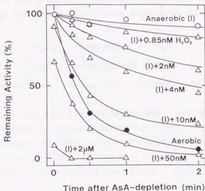
Fig. IV-4 Inactivation of tAPX by hydrogen peroxide in ascorbate (AsA)-depleted medium under anaerobic conditions. tAPX (2 \mu l, 425 nM) in 1 mM ascorbate was diluted with 1 ml of 50 mM potassium phosphate, pH 7.0, containing hydrogen peroxide at the indicated concentrations under anaerobic conditions, unless otherwise specified. The final concentration of tAPX was 0.85 nM. At the indicated times, the inactivation was quenched by the addition of 0.5 mM ascorbate to the incubation mixture. Subsequently, APX activity was determined under the standard assay conditions as described in Materials and Methods. Activity of tAPX in the presence of ascorbate at 0 min was 0.034 unit and is taken as 100%.
