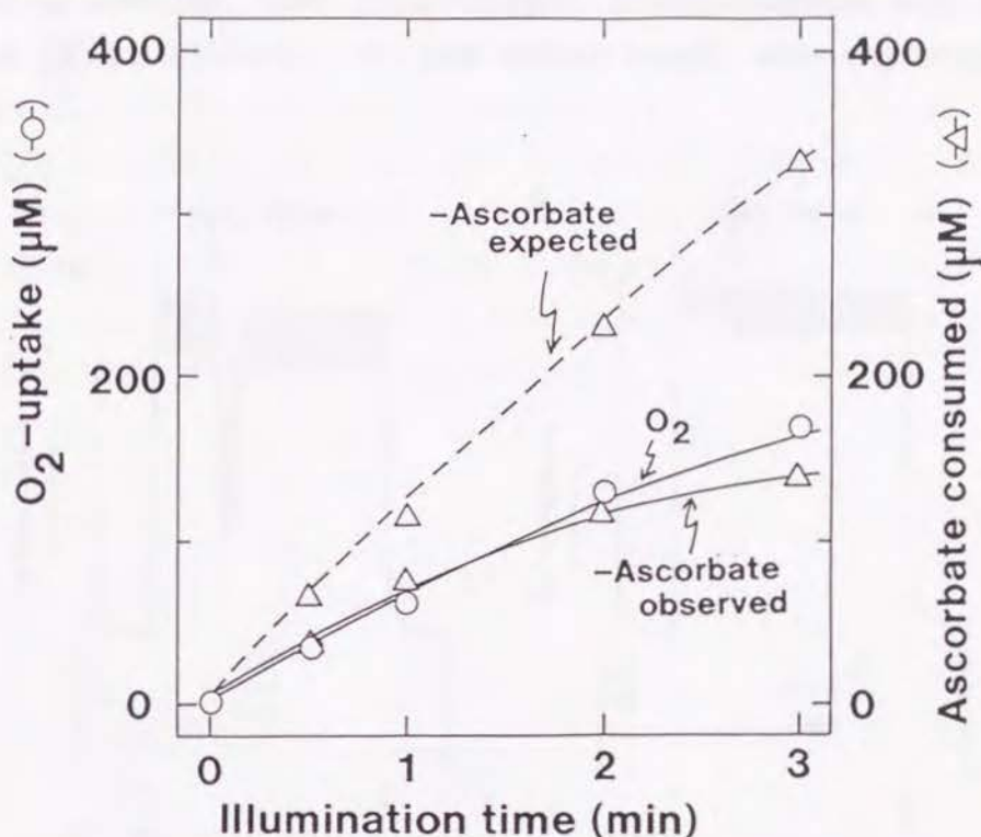
Fig. II-4 Stoichiometry of ascorbate oxidation coupled to the reduction of superoxide and hydrogen peroxide produced in the thylakoids. The reaction mixture (1 ml) in the oxygen electrode vessel contained the thylakoids (30 \mu g Chl), 1 mM methyl viologen and 0.1 \mu M nigericin in the assay medium containing 1 mM ascorbate. After the light was turned on, the uptake of dioxygen was monitored and at indicated times aliquots of the reaction mixture was sampled. The concentration of ascorbate in the sampled aliquots was determined by the decrease in absorbance at 265 nm upon the addition of ascorbate oxidase in 0.1 M potassium phosphate, pH 5.6 (Foyer et al. 1983). The expected decrease of ascorbate is estimated from the oxygen uptake, assuming that no photoregeneration of ascorbate occurred in the thylakoids.
