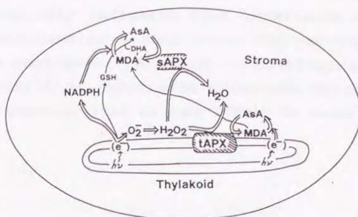
Fig. II-10 Microlocalization of hydrogen peroxide-scavenging systems in chloroplasts. Dioxygen is univalently photoreduced in PS I of thylakoids, and the superoxide anion radicals are disproportionated to hydrogen peroxide and dioxygen by superoxide dismutase. The hydrogen peroxide is reduced to water by the thylakoid-bound ascorbate peroxidase (tAPX), and ascorbate (AsA) is regenerated from the primary oxidation product in a reaction of ascorbate peroxidase, MDA, by its photoreduction in the thylakoids. The hydrogen peroxide and MDA, which are escaped from the interaction in the thylakoids, are reduced by stroma ascorbate peroxidase (sAPX) and MDA reductase in the stroma, respectively. DHA reductase is localized in the stroma, which would regenerate ascorbate from the DHA produced from MDA through its disproportionation.
