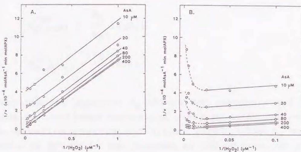
Fig. III-5 Double-reciprocal plots of the initial velocity of the reaction catalyzed by purified tAPX from spinach thylakoids against the concentration of hydrogen peroxide (A, 1.0 - 40 \mu\text{M} ; and B, 10 - 400 \mu\text{M} ) at the indicated concentrations of ascorbate. The initial rates of oxidation of ascorbate catalyzed by tAPX (1 nM) were determined as described in Materials and Methods, with the concentrations of substrate as indicated.
