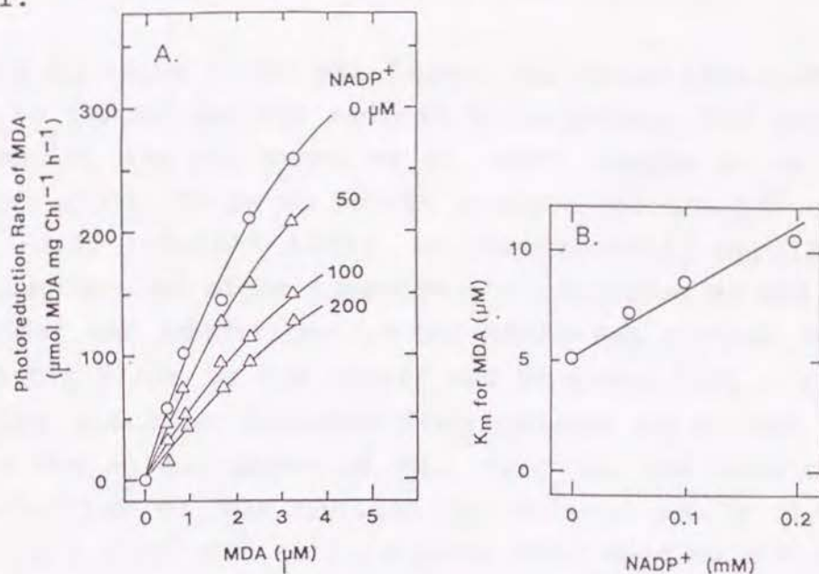
Fig. V-9 Inhibition of the photoreduction of the MDA radical by \text{NADP}^+ in spinach thylakoids. (A) The reaction mixture (70 \mu\text{l} ) contained 50 mM HEPES-KOH, pH 7.6/0.4 M sucrose/2 mM \text{MgCl}_2 /10 mM NaCl/2.5 mM ascorbate/5 \mu\text{M} Fd/0.1 \mu\text{M} nigericin/thylakoid membranes (0.7 \mu\text{g} Chl). \text{NADP}^+ was added at the indicated concentrations. The concentrations of the MDA radical in the reaction mixture were adjusted, as indicated, by changing the concentration of ascorbate oxidase added to the reaction mixture before illumination. Initial rates of photoreduction of the MDA radical were measured as described in the legend to Fig. V-4. (B) Apparent K_m values for the MDA radical during its photoreduction at the indicated concentrations of \text{NADP}^+ were determined from the non-linear regression analysis using Michaelis and Menten's equation (Sakota and Hiromi 1976) and they were plotted against the concentration of \text{NADP}^+ .
