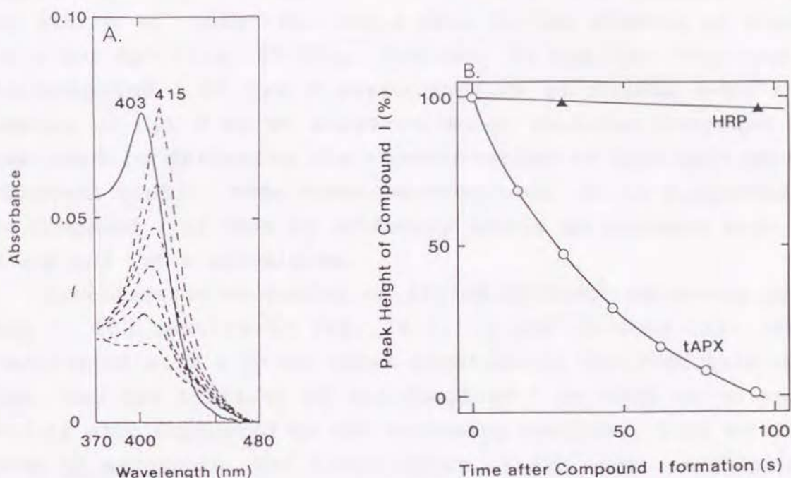
Fig. IV-5 (A) Degradation of Compound I of tAPX in the absence of ascorbate. The absorption spectrum of native tAPX ( 0.9 \mu\text{M} ) was recorded in 50 mM potassium phosphate, pH 7.0, 1 mM ascorbate and 1% CHAPSO (—). Subsequently, 1 mM hydrogen peroxide was added, and the recording of the absorption of the Compound I was started from 480 nm at a scanning rate of 7.1 \text{ nm s}^{-1} (---). The absorbances at 415 nm of APX-I were recorded at 8.8, 23.94, 39.06, 54.18, 69.3, 84.42 and 99.54 s after the addition of hydrogen peroxide from the top to the bottom spectra. (B) Time-dependent decreases of Compounds I of tAPX and horseradish peroxidase (HRP). Native form of 1 \mu\text{M} HRP in 50 mM potassium phosphate, pH 7.0, gave an absorption spectrum characteristic of a ferric high-spin state with a Soret peak at 403 nm (data not shown). The Soret peak of native HRP was shifted to 415 nm to form the two-electron oxidized enzyme, Compound I, by the addition of 2 mM hydrogen peroxide. The absorbances at 415 nm of Compound I of HRP were recorded at 8.8, 39.06 and 99.54 s after the addition of hydrogen peroxide. Absorbance changes at 415 nm of APX-Compound I and HRP Compound I are plotted against times after hydrogen peroxide was added. Absorbances of Compounds I of APX and HRP at 415 nm at 8.8 s, after the addition of hydrogen peroxide, are taken as 100% at 0 s.
