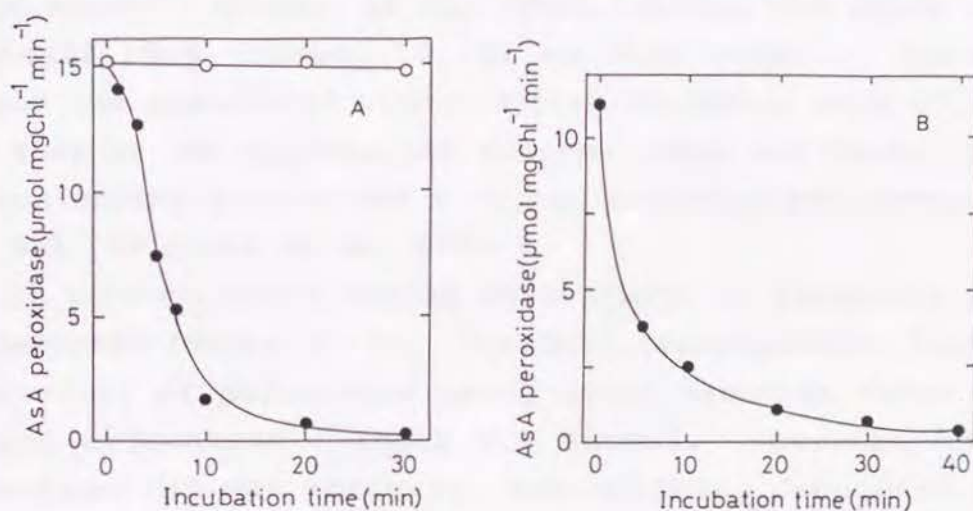
Fig. VI-1 The inactivation of AsA peroxidase by depletion of AsA in an extract (A) and cells (B) of Euglena . (A) The harvested cells were sonicated at 1 mg Chl \text{ml}^{-1} in the suspension medium (50 mM HEPES-KOH, pH 7.0, 330 mM sorbitol, 0.1 mM EDTA and 20 \mu\text{M} AsA) and centrifuged at 15,000 \times g for 1 min. The supernatant was diluted 200-fold with AsA-depleted suspension medium and incubated at 25°C (closed circles). The undiluted supernatant (open circles) also was incubated under the same conditions, and the respective activities were assayed. At the indicated times, each extract was assayed in an AsA-containing reaction mixture, and the activity of AsA peroxidase was determined. (B) The cells (36 \mu\text{g Chl ml}^{-1} ) suspended in 10 mM \text{NaHCO}_3 were incubated at 25°C with 2.6 mM \text{H}_2\text{O}_2 in the dark for the indicated times. The cells were sonicated in the suspension medium and the activity of AsA peroxidase was assayed after centrifugation.
