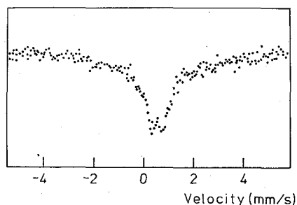
Fig. 6. Mössbauer spectra of amorphous \text{Fe}_{47}\text{Sb}_{53} film at 4.2 K.
