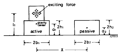
Fig. 9 Foundation-soil-foundation system considered
