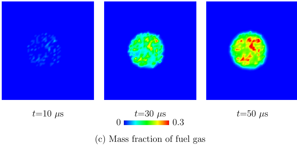
Figure 12: Time variations of distributions of instantaneous (a) gas temperature, T , (b) mass fraction of O_2 , Y_{O_2} , and (c) mass fraction of fuel gas, Y_F , in air at initial gas temperature of T_0=2000 K, ambient pressure of P=0.1 MPa, and ML=0.36 in Case 15.
