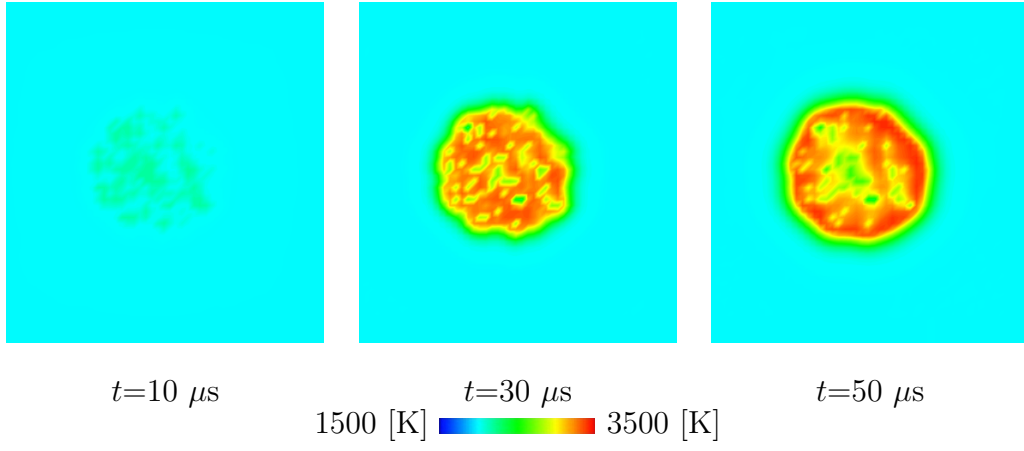
(a) Gas temperature
