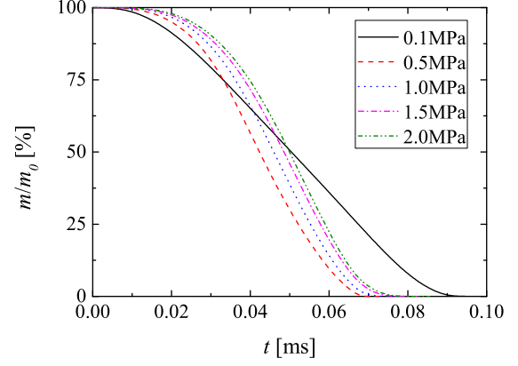
(b) T_0=1500 K (Case 9)
