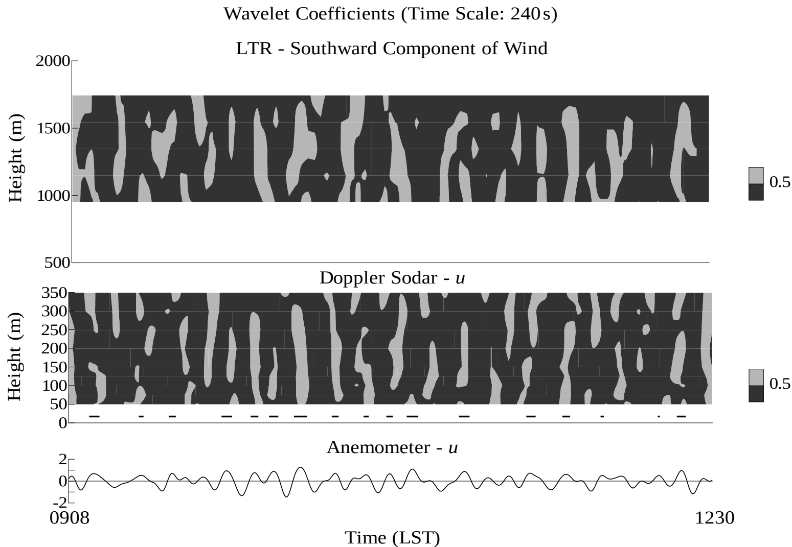
Fig. 9 ( Upper ) Time–height cross-section of wavelet coefficients for the southward component of wind observed by the lower troposphere radar (LTR) on December 10, 2001 at Shigaraki. ( Middle ) Corresponding section of wavelet coefficients for the u velocity component observed by the Doppler sodar. ( Lower ) Corresponding time series of wavelet coefficients for the u velocity component measured by the cup anemometer with the wind vane. Areas of light tone in the upper and middle figures denote the regions in which the wavelet coefficient is larger than the threshold value, and bold bars in the middle figure show the periods during which the wavelet coefficient for the anemometer data is larger than the threshold value
