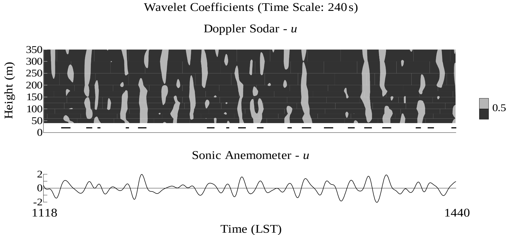
Fig. 8 ( Upper ) Time–height cross-section of wavelet coefficients for the u velocity component observed by the Doppler sodar on December 8, 1998 at Shionomisaki. ( Lower ) Corresponding time series of wavelet coefficients for the same velocity component measured by the sonic anemometer. Areas of light tone denote the regions in which the wavelet coefficient for the Doppler sodar data is larger than the threshold value, and bold bars show the periods during which the wavelet coefficient for the sonic anemometer data is larger than the threshold value
