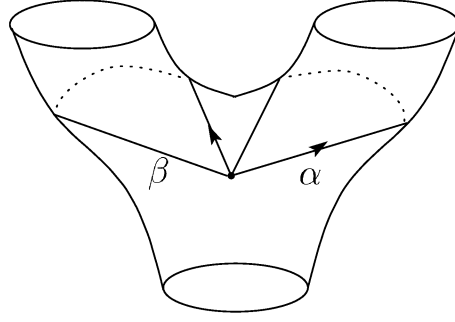
Figure 2. S^2 - \coprod_{i=1}^3 \text{Int } D_i
