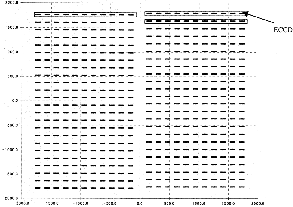
Fig. 4. Element arrangement of a 22 by 24 planar ECCD array (unit: millimeters).
