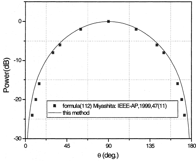
Fig. 2. Comparison of the ECCD radiation patterns simulated by using two kinds of methods. Length of a circular pipe = 0.42 \lambda_0 , diameter of the pipe = 0.46 \lambda_0 .
