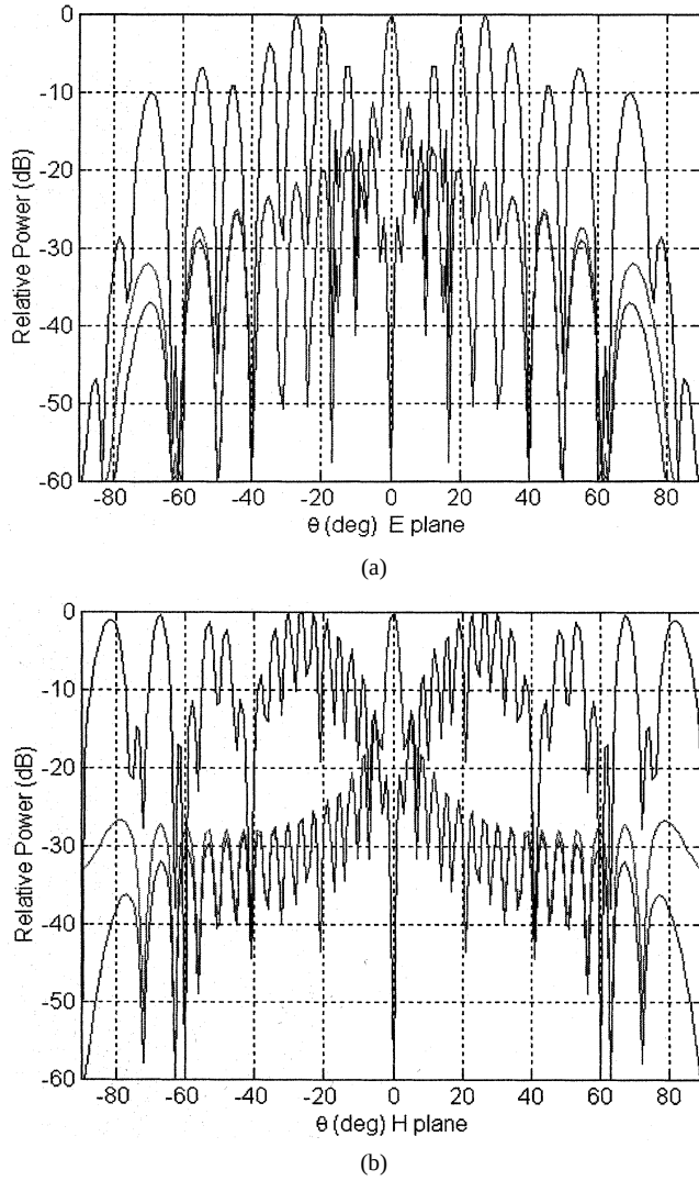
Fig. 5. (a) Effects of height of a 22 by 24 ECCD ( b = 0.025 \lambda_0 , a = 0.009 \lambda_0 , length = 0.5 \lambda_0 ) array over a square plate on radiation pattern. The sidelength of the plate is 18.1818 \lambda_0 . The height of the array over the plate is 0.25 \lambda_0 and 2 \lambda_0 for bottom line and top line, respectively. There is no plate for middle line.
