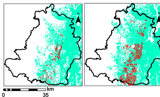
Fig. 10 Comparison between the flood case of 2.33 and 100 year return period (blue part indicates flood extent, red parts indicate the high flood flow area (&gt;0.5m/s)).
