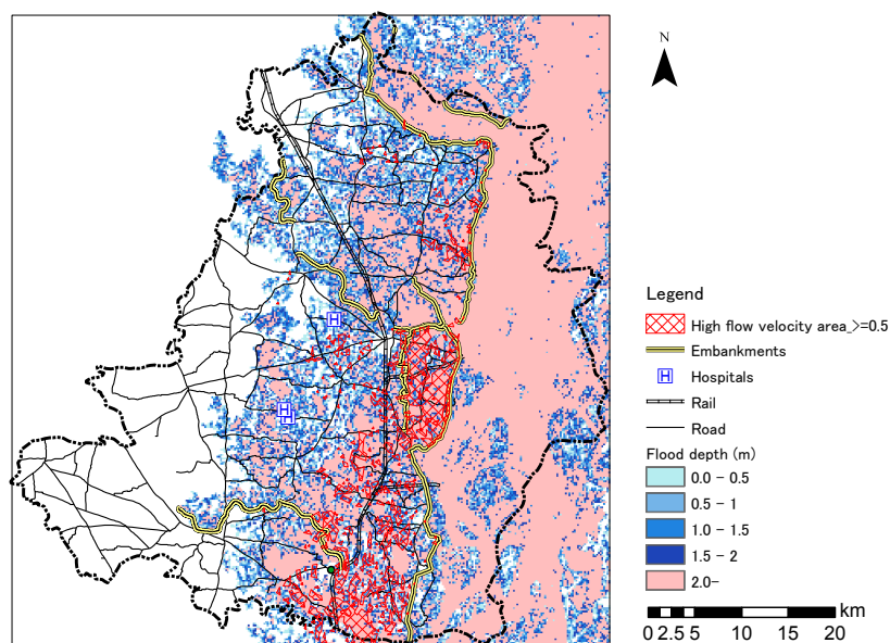
Fig. 11 Flood Hazard Map focusing on the flood depth and velocity.
