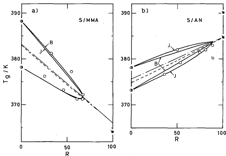
Figure 2 a and b. Plots of T_g against R for (a) S/MMA 12 and (b) S/AN copolymers: 2 data with pip, Hirooka and Kato. 11 For key of each symbol or line, refer to Fig. 1.
