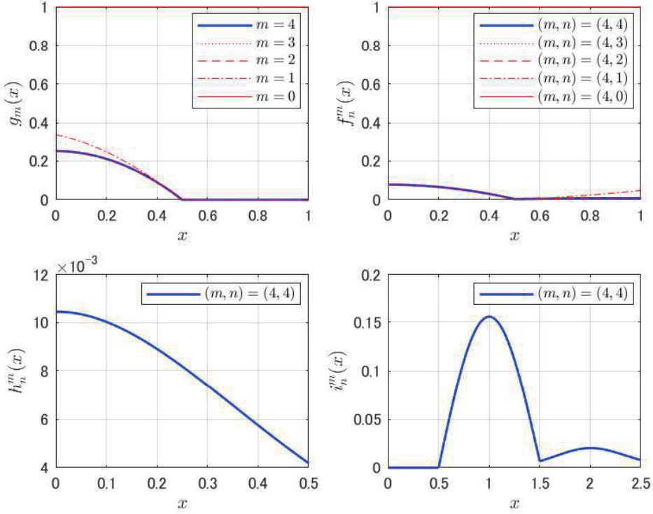
Figure 2: Observer gains for chaotic system.
