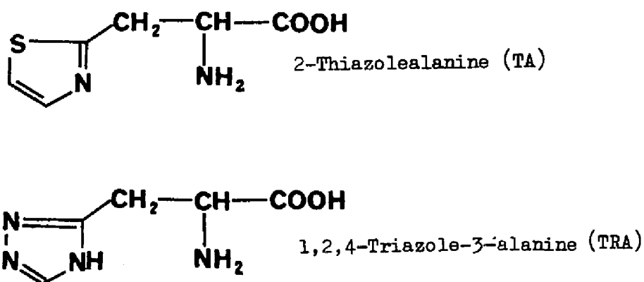
Fig. 1. Histidine Analogs
