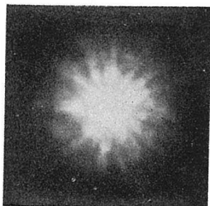
Photo 29. Sn (42%)-Bi alloy. Sand cast. (Transversal section)
