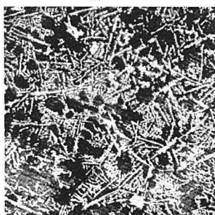
Photo 6. Modified with 0.8% Mg \times 100
