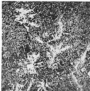
Photo 24. Modified with 0.2% Al (H 2 -treated) \times 100
