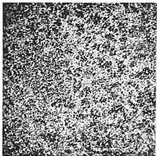
Photo 1. Sb (12.5%)-Pb alloy. Chill cast \times 100
