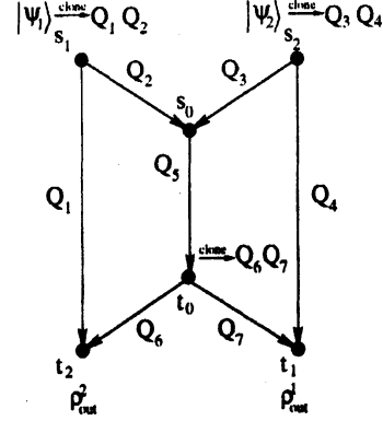
Figure 5: Protocol XQQ.
