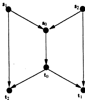
Figure 1: Butterfly network.
