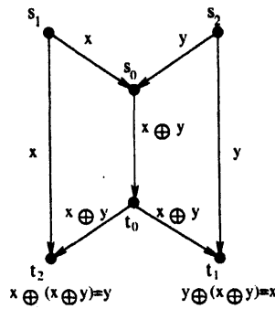
Figure 2: Coding scheme
