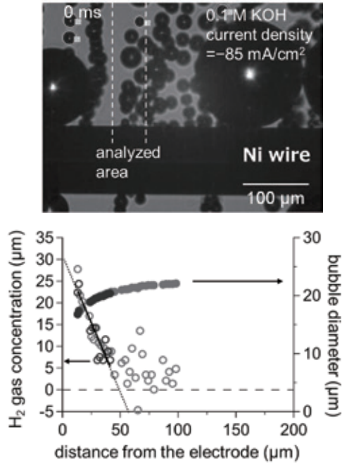
Fig. 2 Analysis of H 2 gas concentration in proximity to the Ni wire electrode. (a) Optical image and (b) H 2 gas concentration obtained from the bubble growth rate at the different distances from the electrode.
