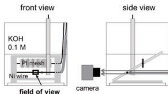
Fig. 1 Experimental setup to optically detect the electrolysis bubble. (a) front view and (b) side view. As shown in (b) bubbles are illuminated from behind the wire electrode by LED.
