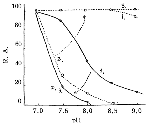
Fig. 6. The effect of \text{CaCl}_2 (0.1M in final) on the Osvan-alkaline treatment.
