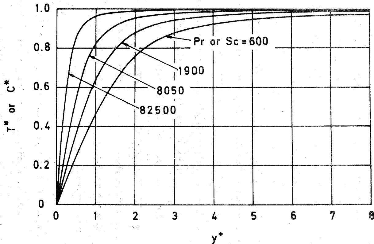
Fig. 5-2 Temperature or concentration distributions at large Prandtl or Schmidt numbers and at Re = 10^4 .
