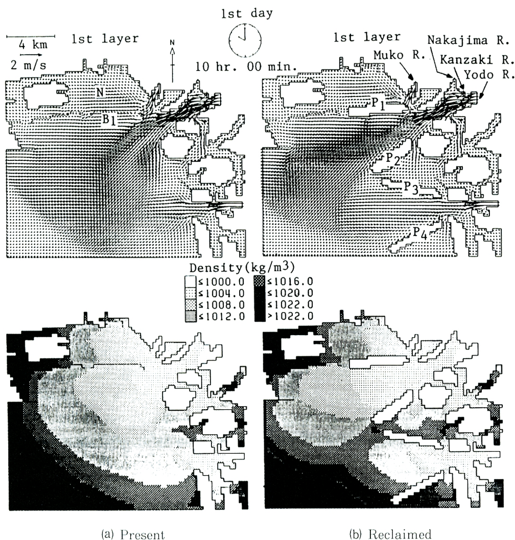
Fig. 6. Velocity and density distribution in surface layer.
