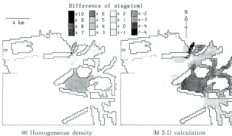
Fig. 10. Water stage rise due to reclamation.
