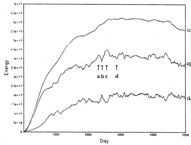
Fig.2 Time series of basin averaged energies for Case 2l. tc (=ap+tk) , ap (= \iint 0.5 \Delta \rho g (\Delta h)^2 dS) , tk (= \iint 0.5 \rho h_1 (u_1^2 + v_1^2) dS + \iint 0.5 \rho h_2 (u_2^2 + v_2^2) dS) represent total energy, available potential energy, total kinetic energy, respectively. The unit is kg m^2 s^{-2} . The arrows show the positions where the rapid conversions between ap and tk occur (See the text).
