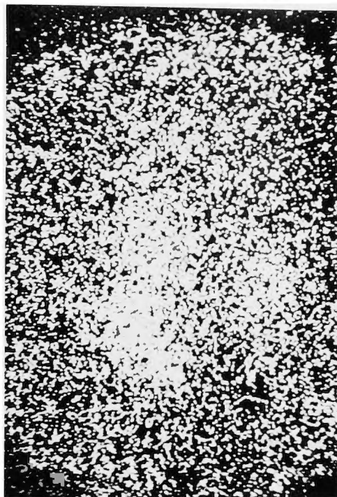
Fig. 2 Scintigram with ^{201}\text{Tl}
